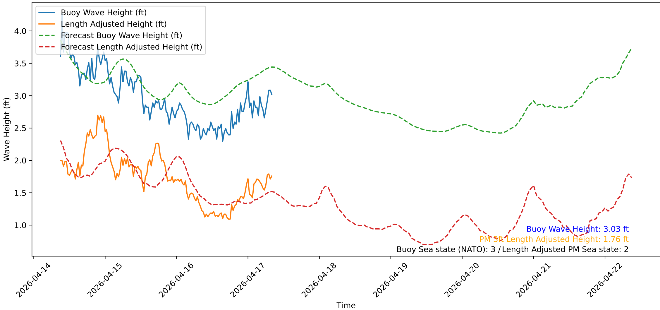
Wave Heights over Time for Oceanside Harbor at 2026-04-17 09:00:31
