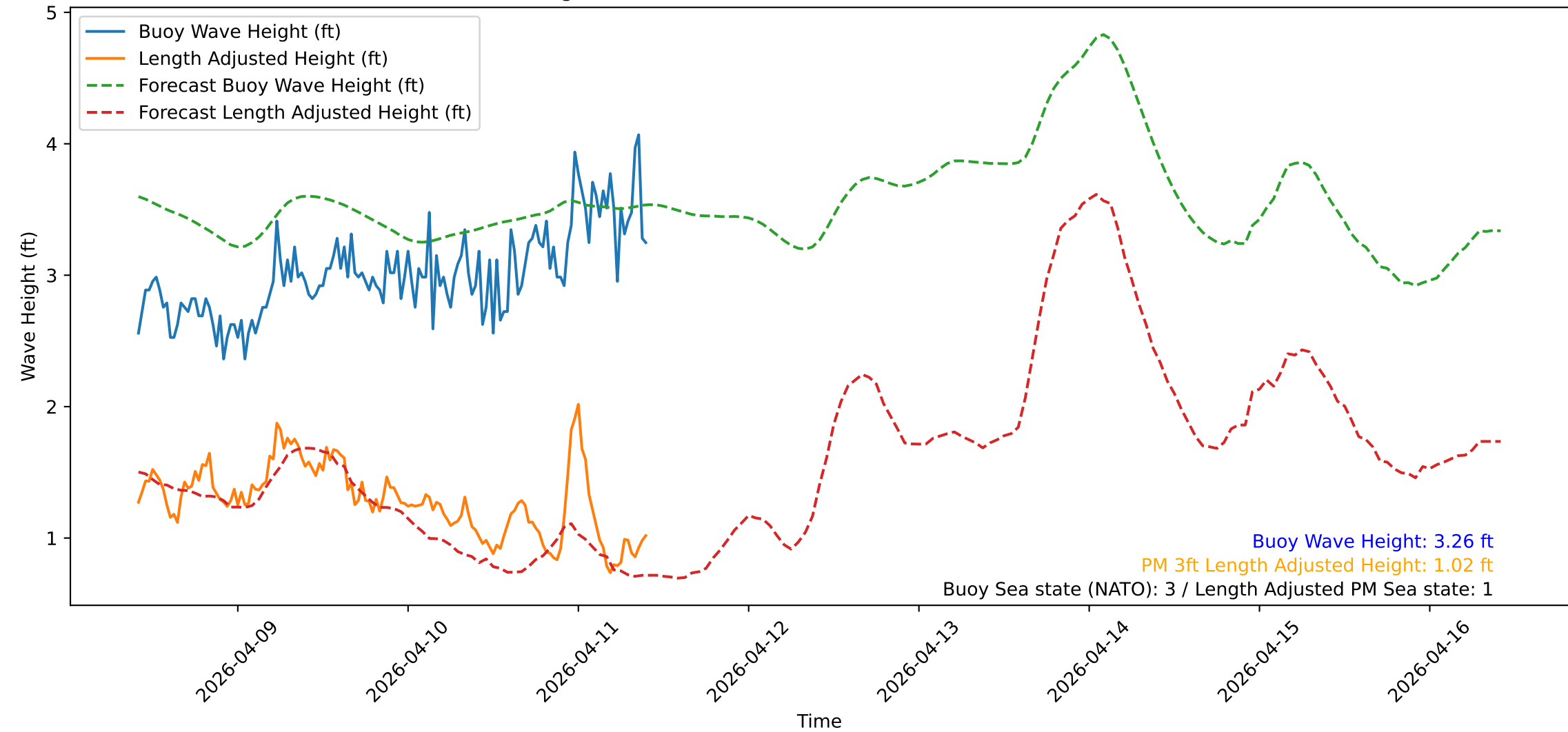
Wave Heights over Time for Green Beach at 2026-04-11 10:11:12
