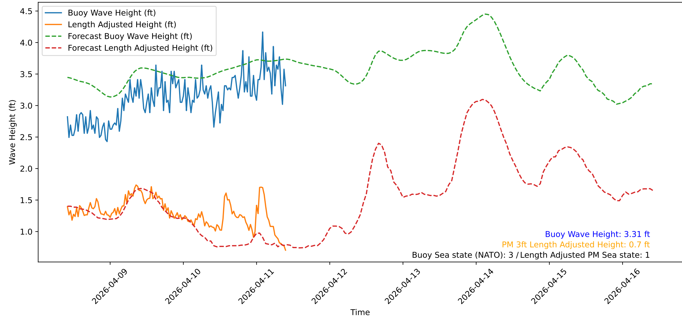
Wave Heights over Time for Oceanside Harbor at 2026-04-11 10:10:31
