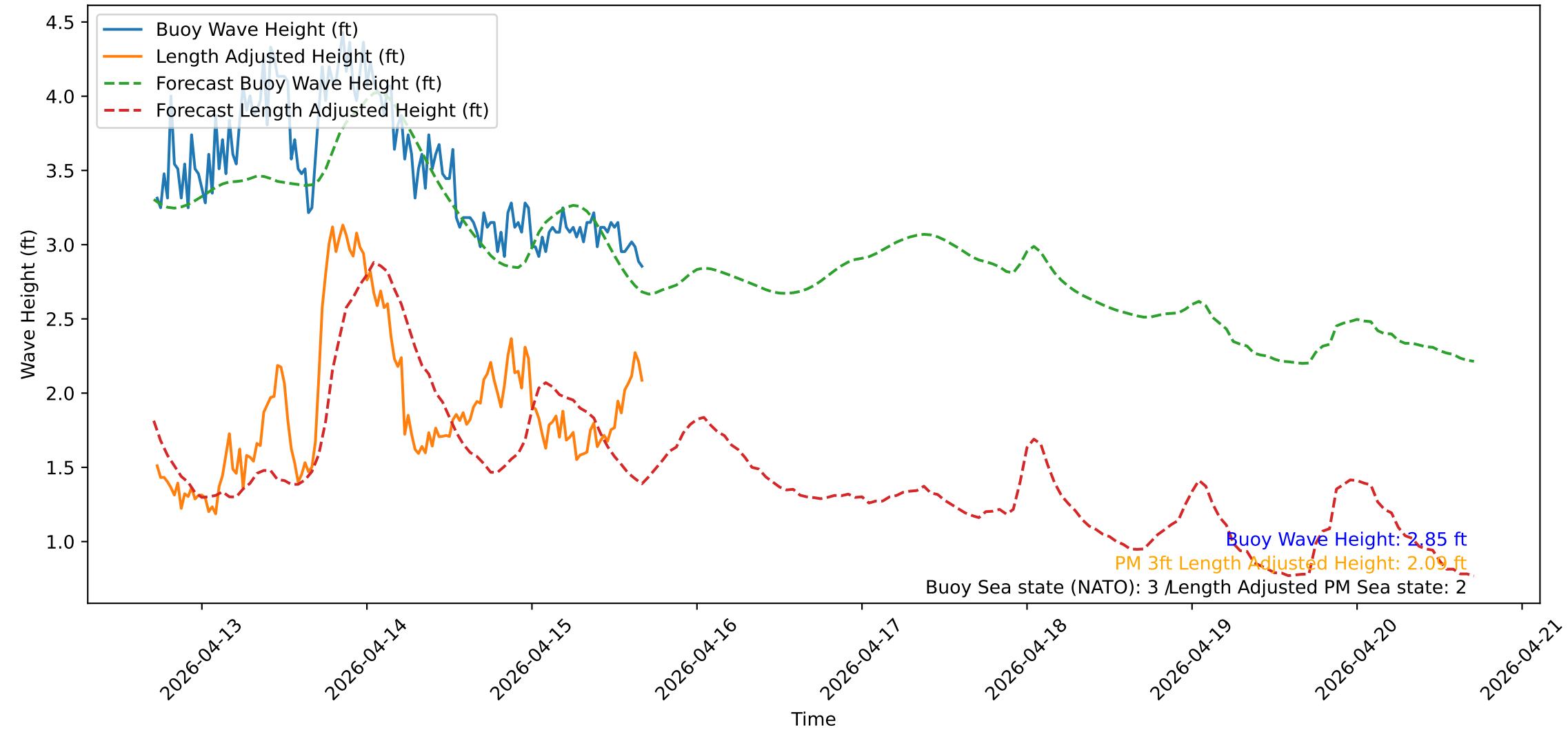
Wave Heights over Time for Red Beach at 2026-04-15 17:00:50
