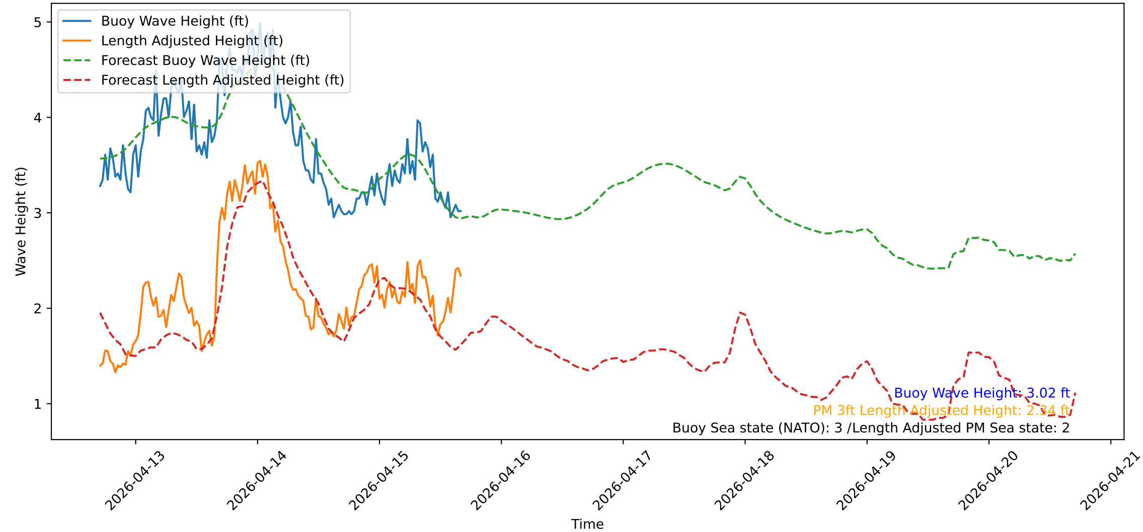
Wave Heights over Time for Green Beach at 2026-04-15 17:01:12
