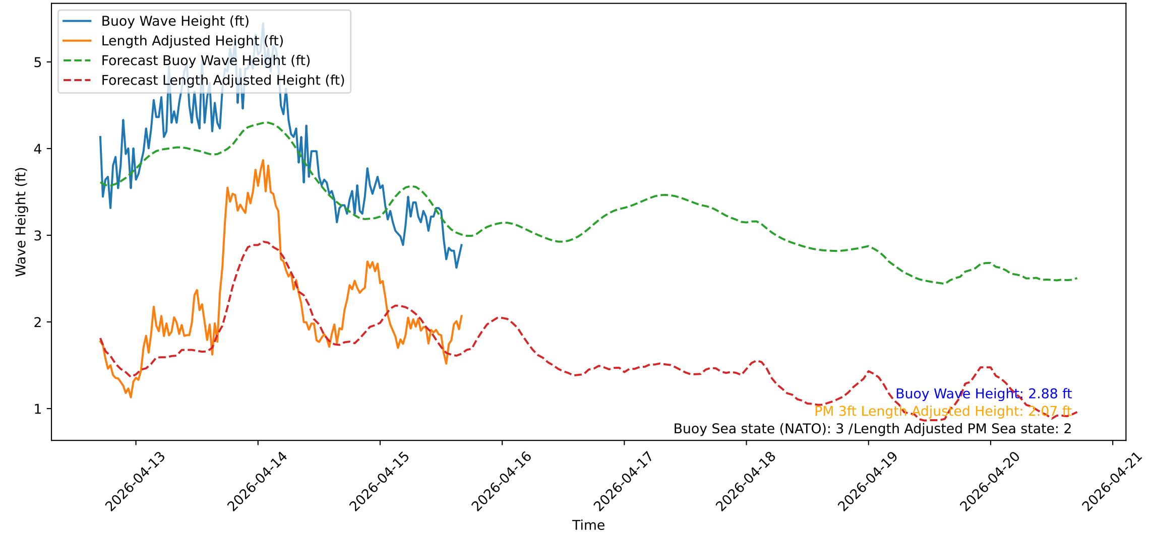
Wave Heights over Time for Oceanside Harbor at 2026-04-15 17:00:31
