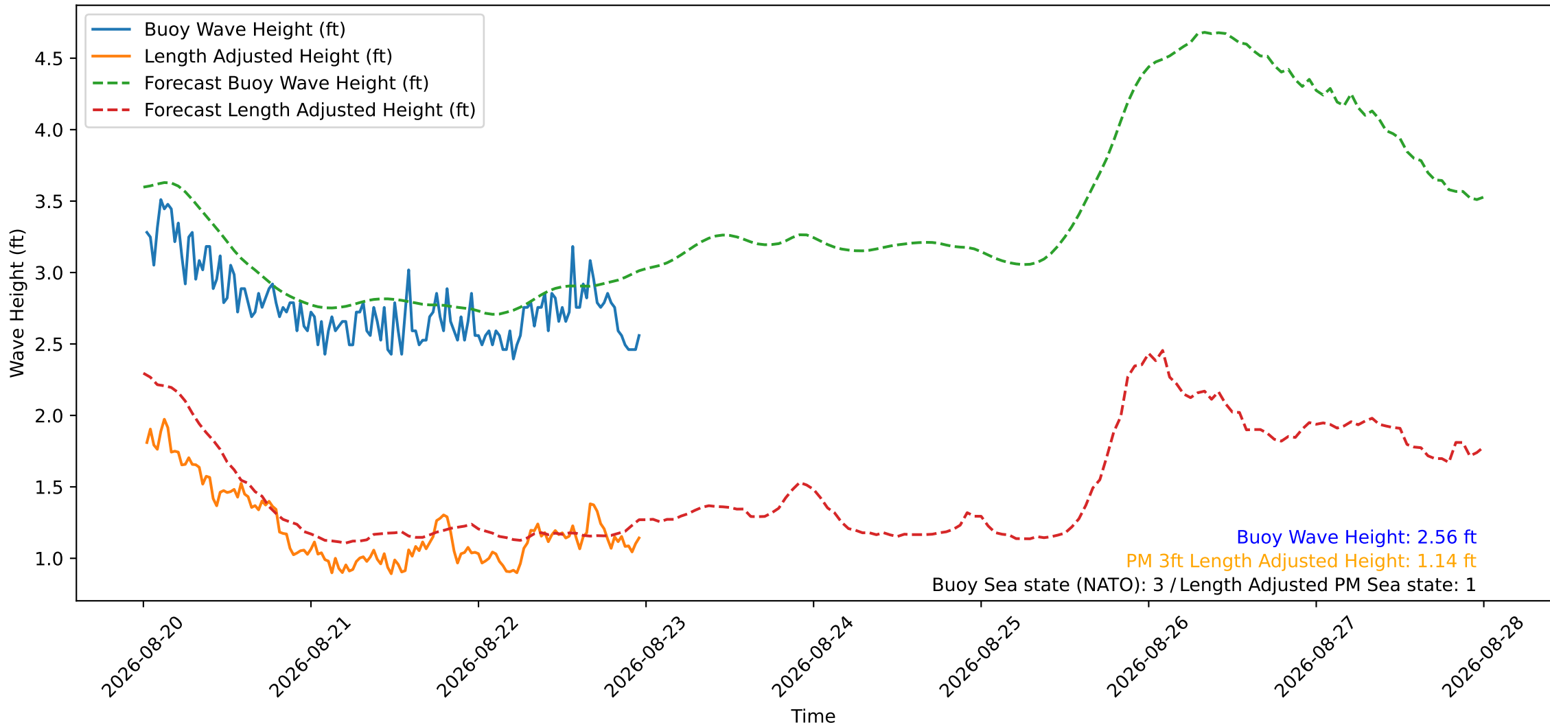
Wave Heights over Time for Green Beach at 2026-08-23 00:01:11
