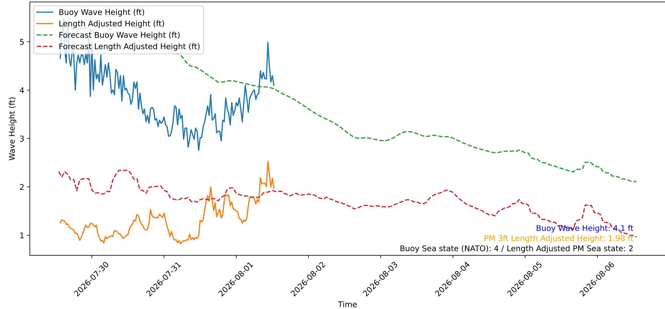
Wave Heights over Time for Green Beach at 2026-08-01 13:21:10
