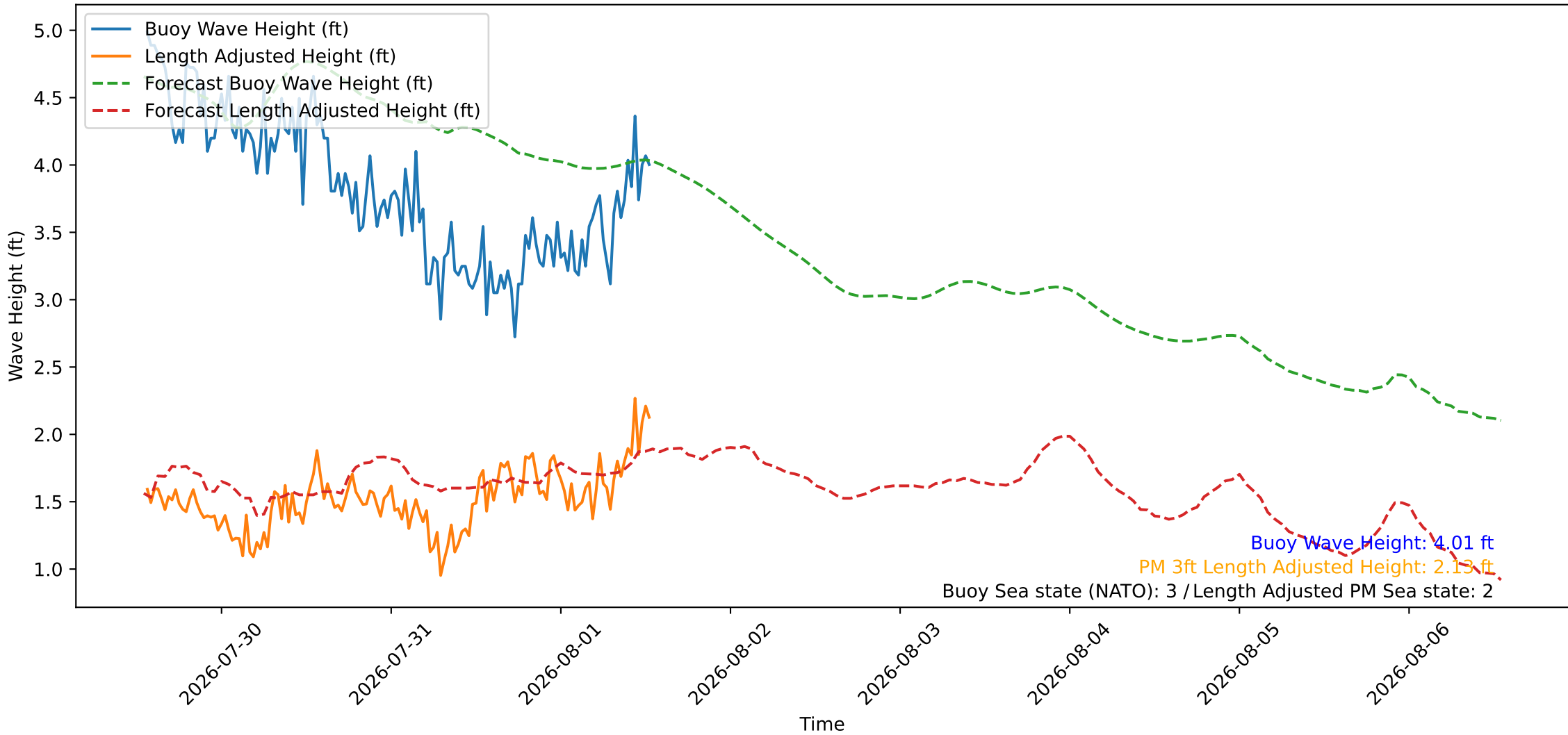
Wave Heights over Time for Oceanside Harbor at 2026-08-01 13:20:26
