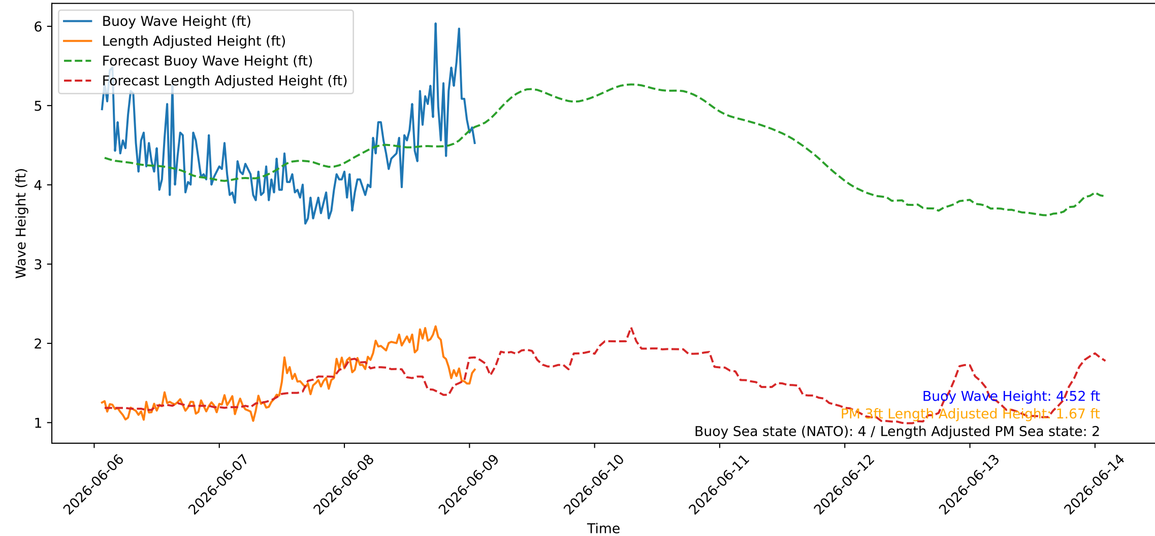
Wave Heights over Time for Oceanside Harbor at 2026-06-09 01:40:26
