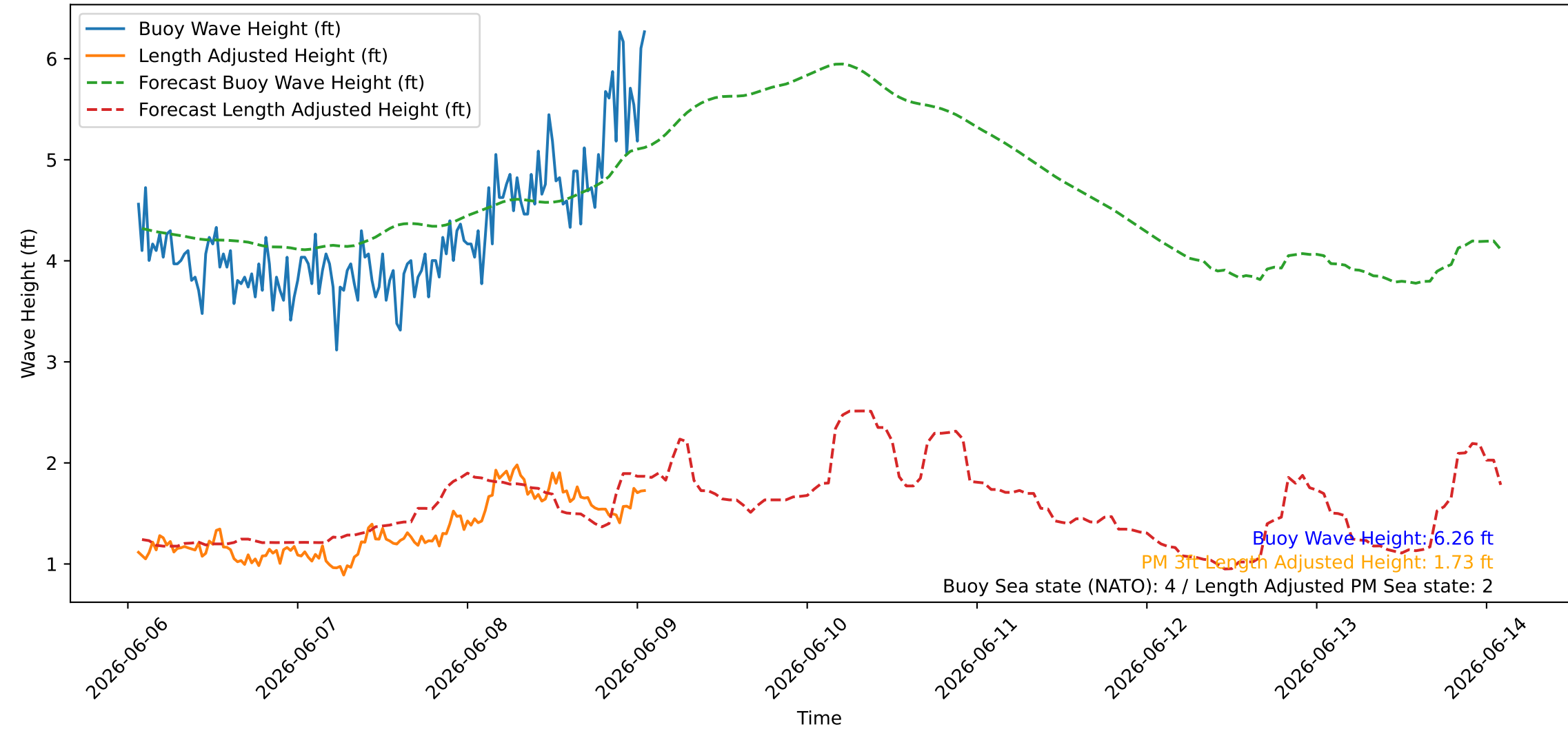
Wave Heights over Time for Green Beach at 2026-06-09 01:41:09
