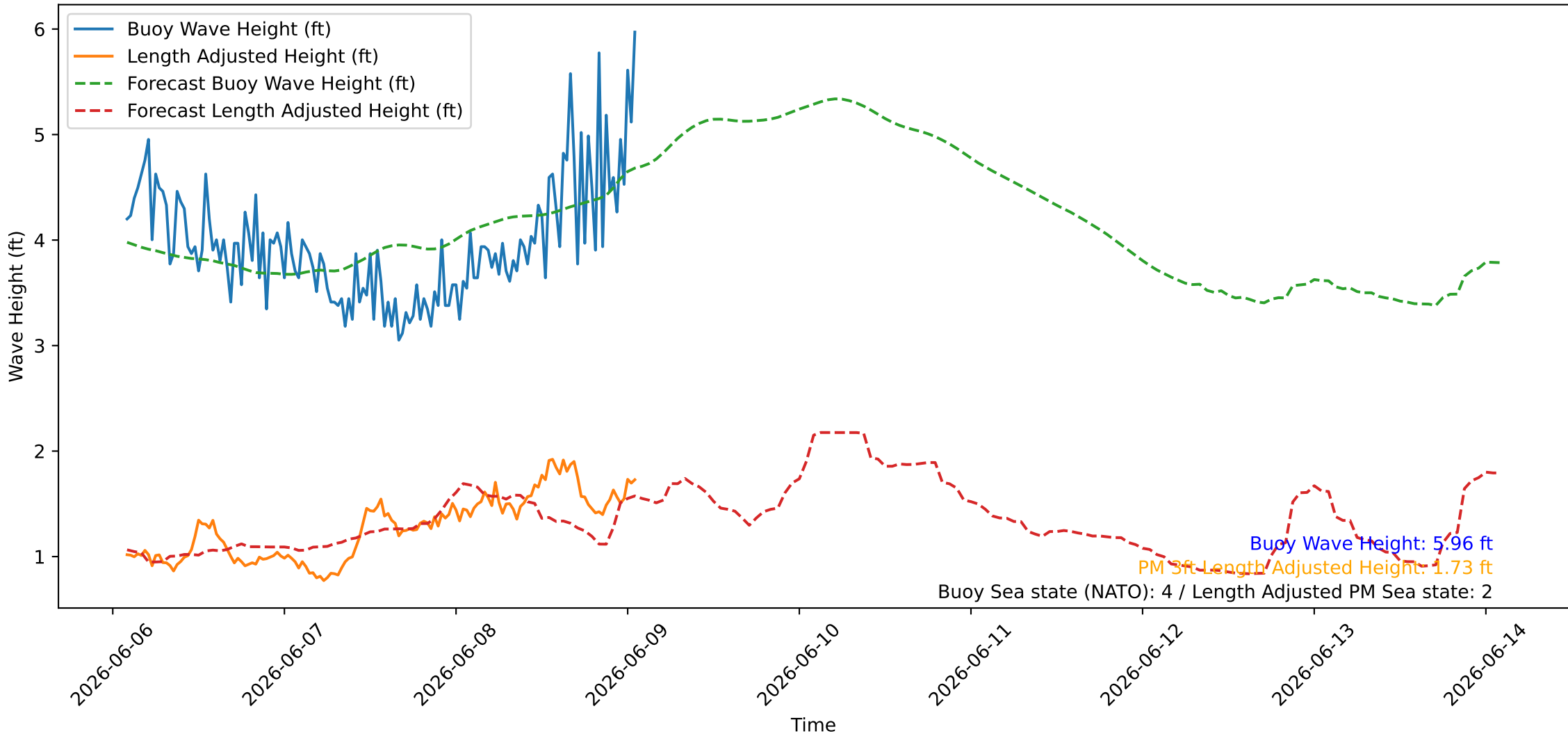
Wave Heights over Time for Red Beach at 2026-06-09 01:40:46
