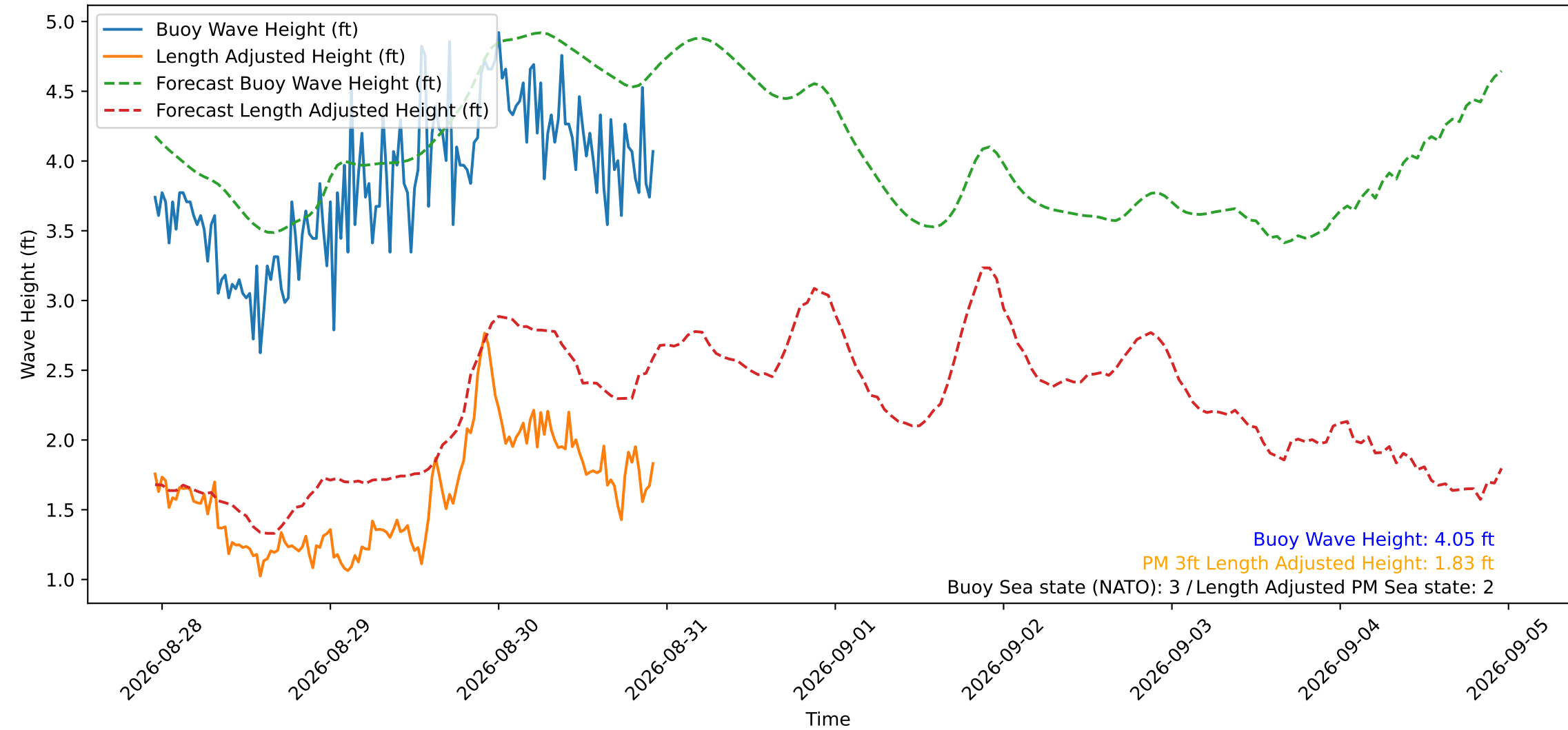
Wave Heights over Time for Green Beach at 2026-08-30 22:41:12
