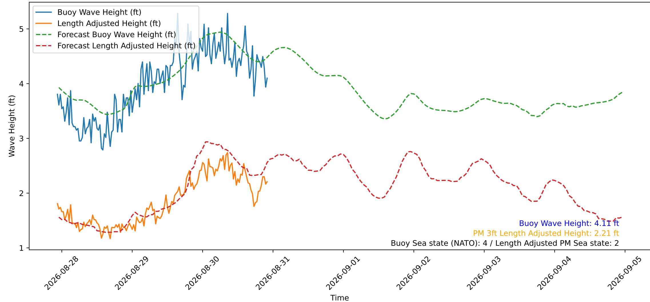
Wave Heights over Time for Oceanside Harbor at 2026-08-30 22:40:29
