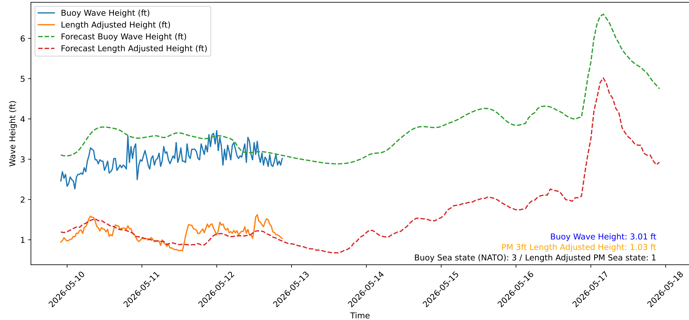
Wave Heights over Time for Oceanside Harbor at 2026-05-12 21:50:32
