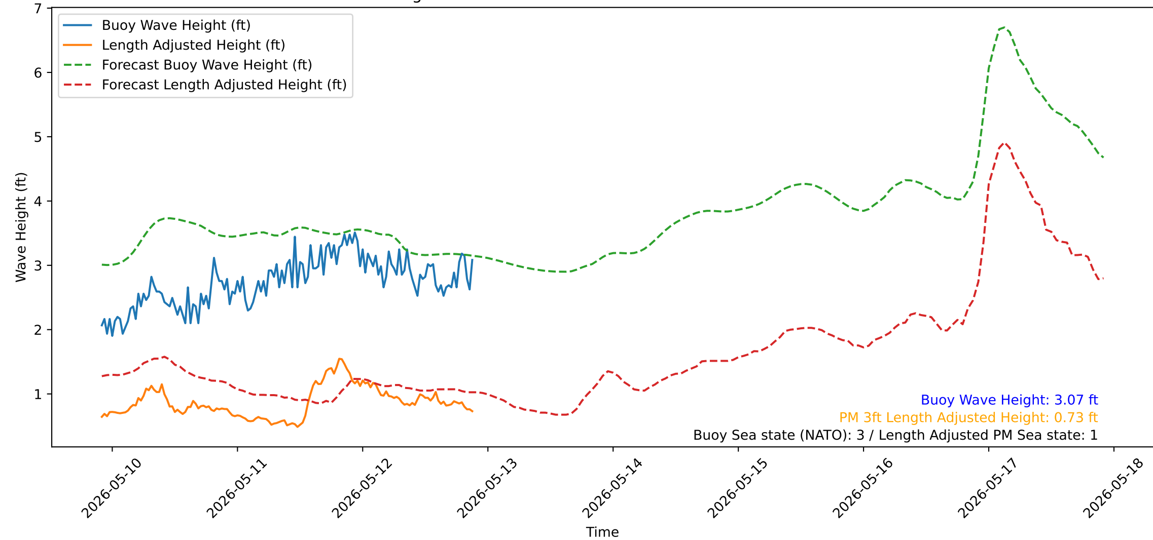
Wave Heights over Time for Green Beach at 2026-05-12 21:51:17
