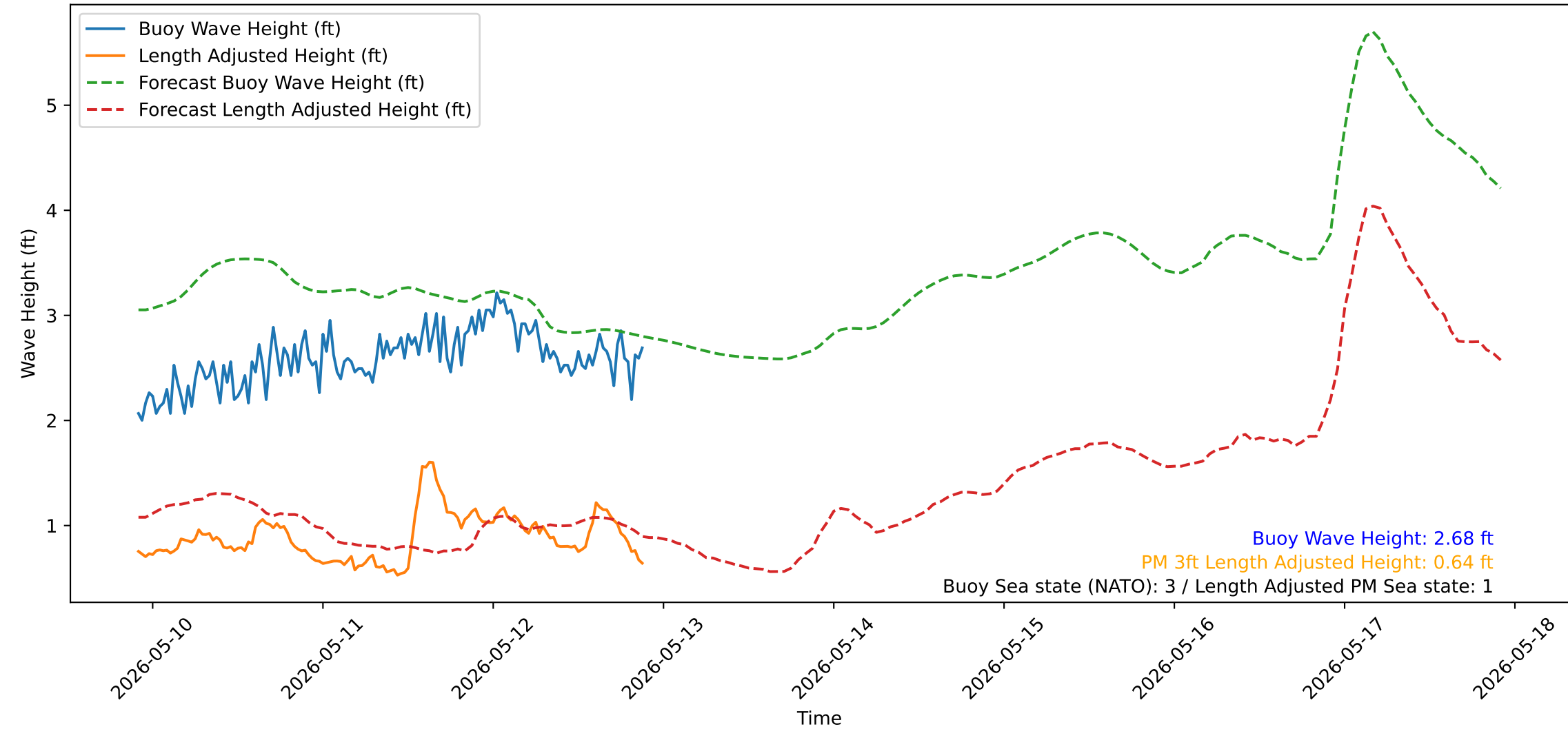
Wave Heights over Time for Red Beach at 2026-05-12 21:50:55
