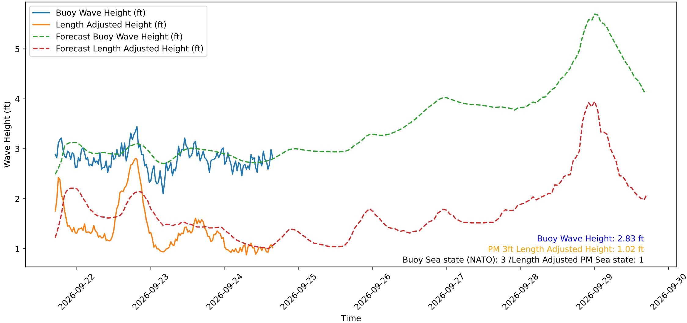
Wave Heights over Time for Green Beach at 2026-09-24 16:31:12
