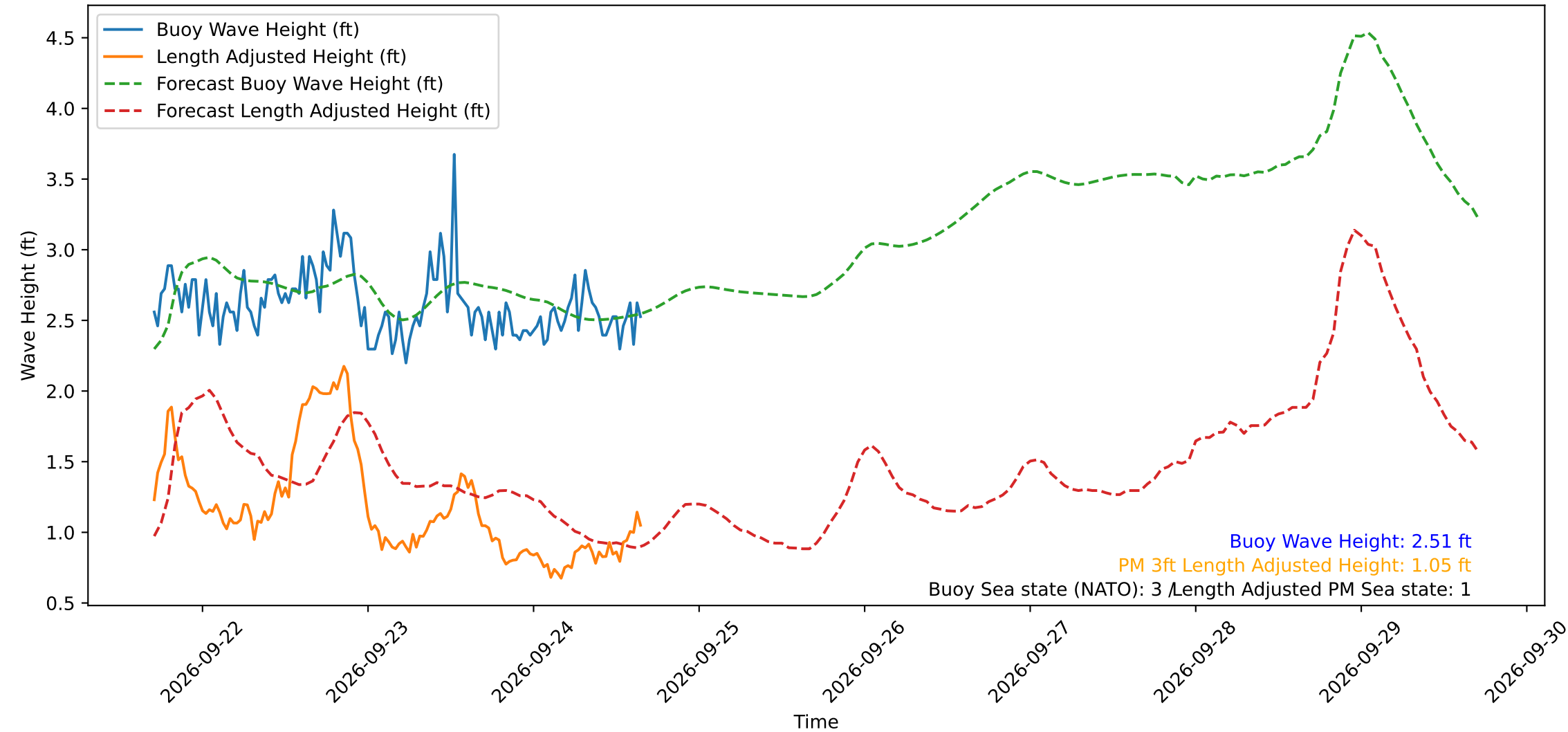
Wave Heights over Time for Red Beach at 2026-09-24 16:30:49
