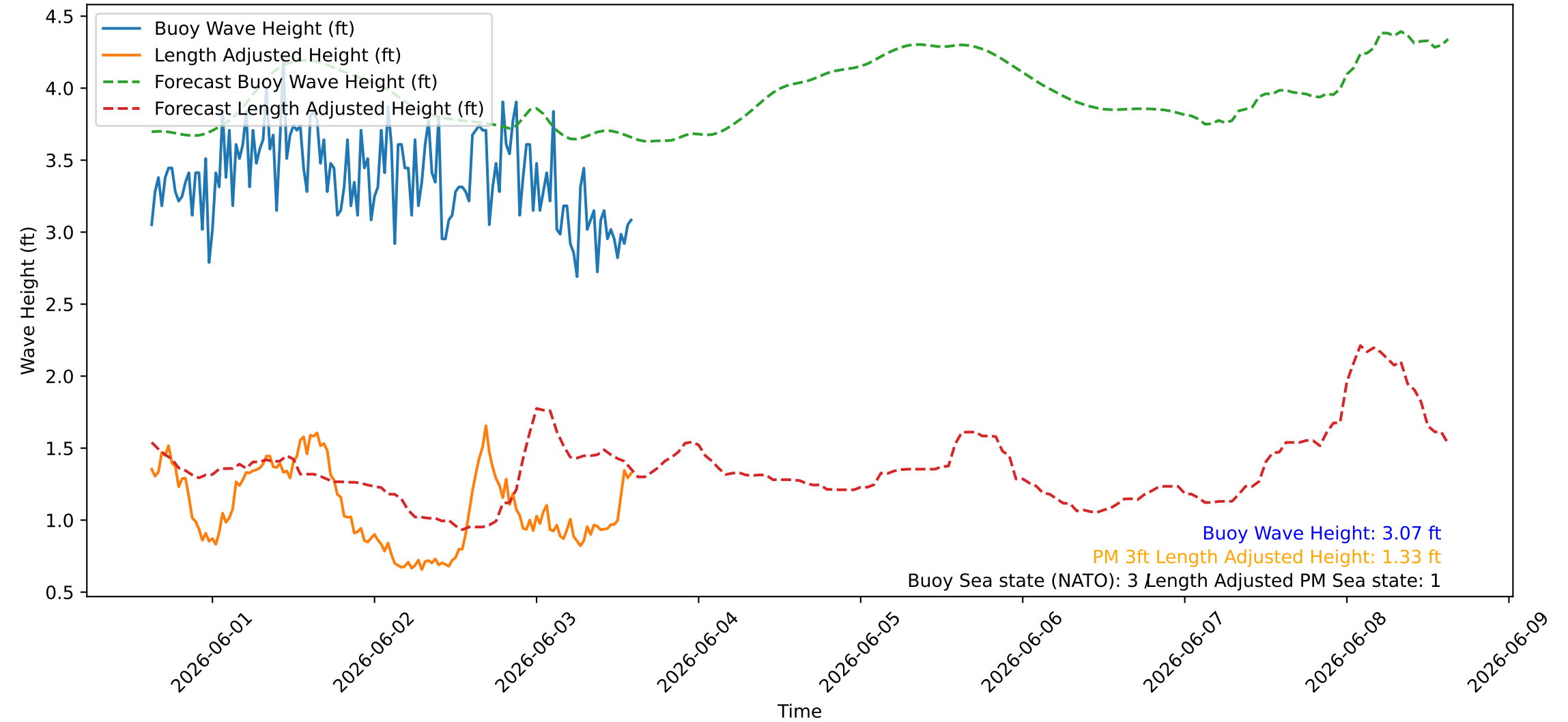
Wave Heights over Time for Red Beach at 2026-06-03 14:50:45
