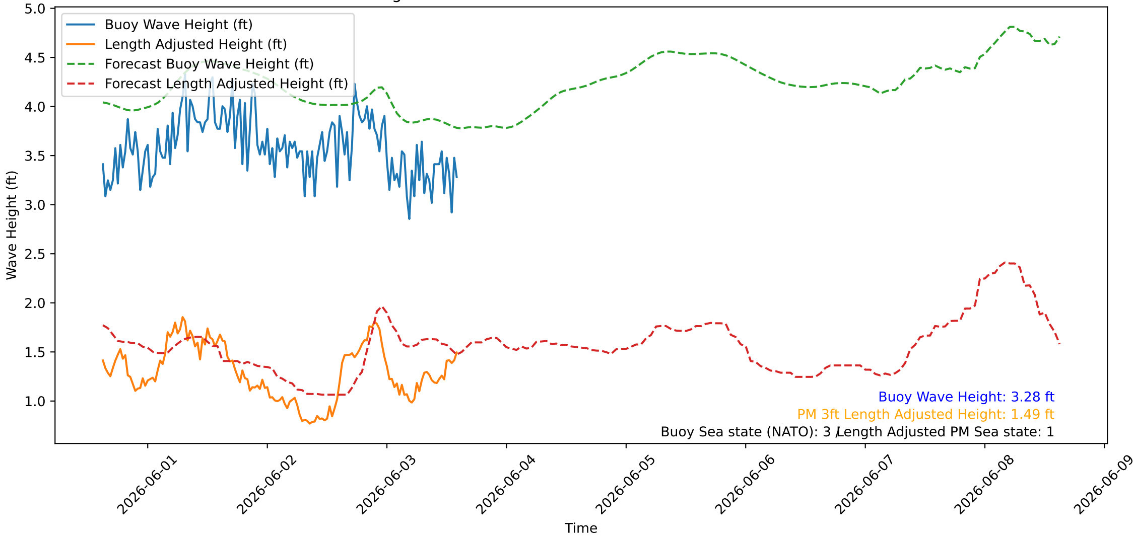
Wave Heights over Time for Green Beach at 2026-06-03 14:51:08
