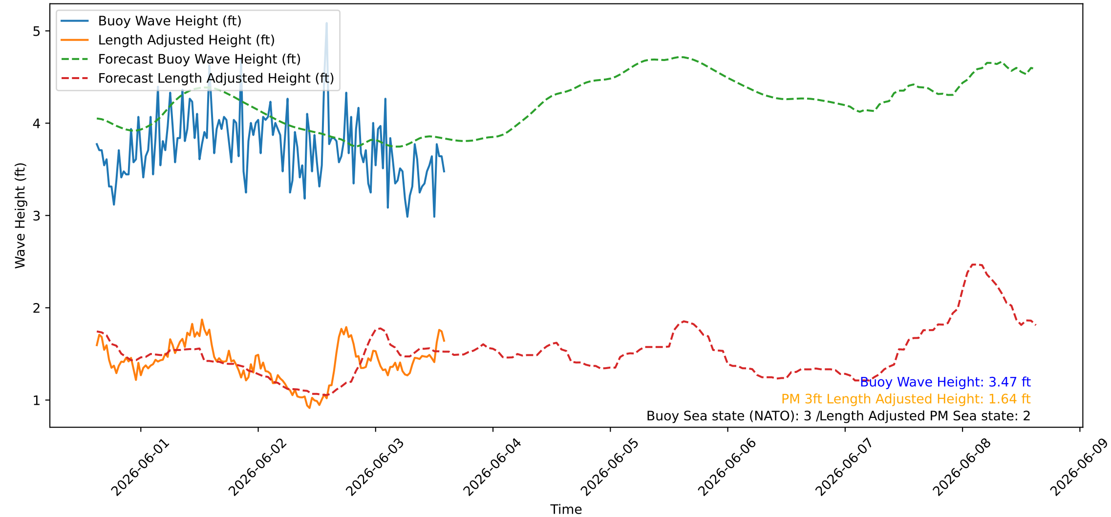
Wave Heights over Time for Oceanside Harbor at 2026-06-03 14:50:25
