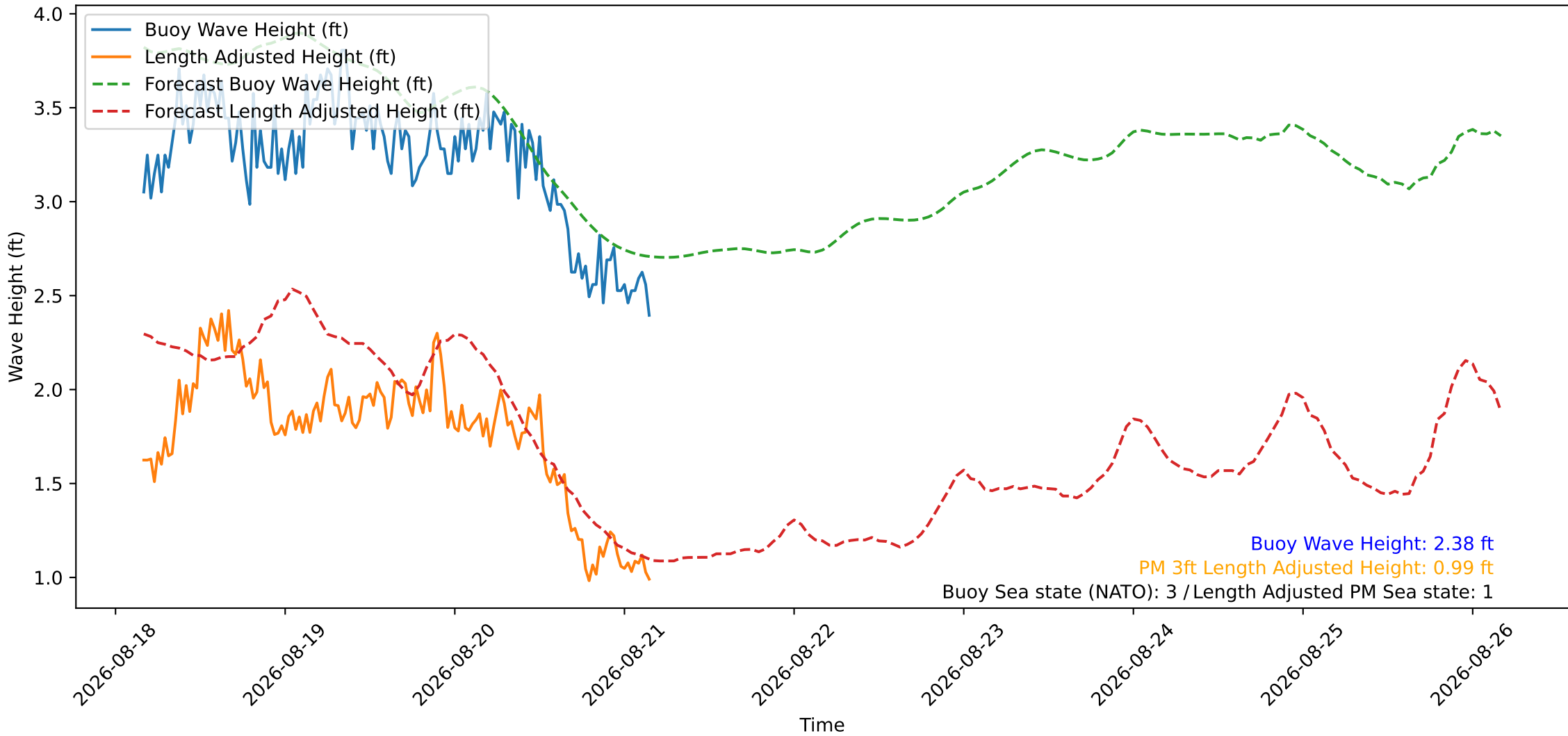
Wave Heights over Time for Oceanside Harbor at 2026-08-21 04:10:26
