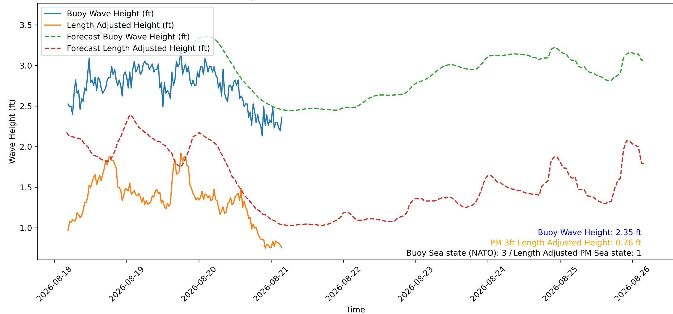
Wave Heights over Time for Red Beach at 2026-08-21 04:10:45
