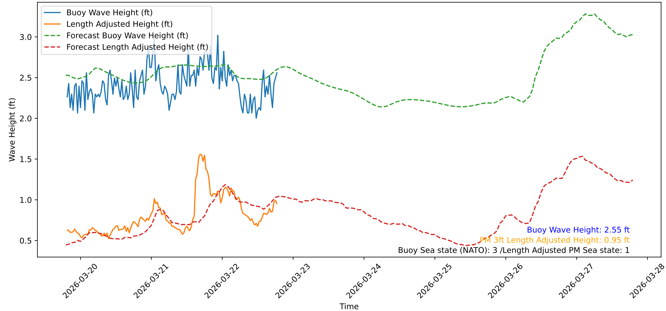
Wave Heights over Time for Oceanside Harbor at 2026-03-22 19:20:31
