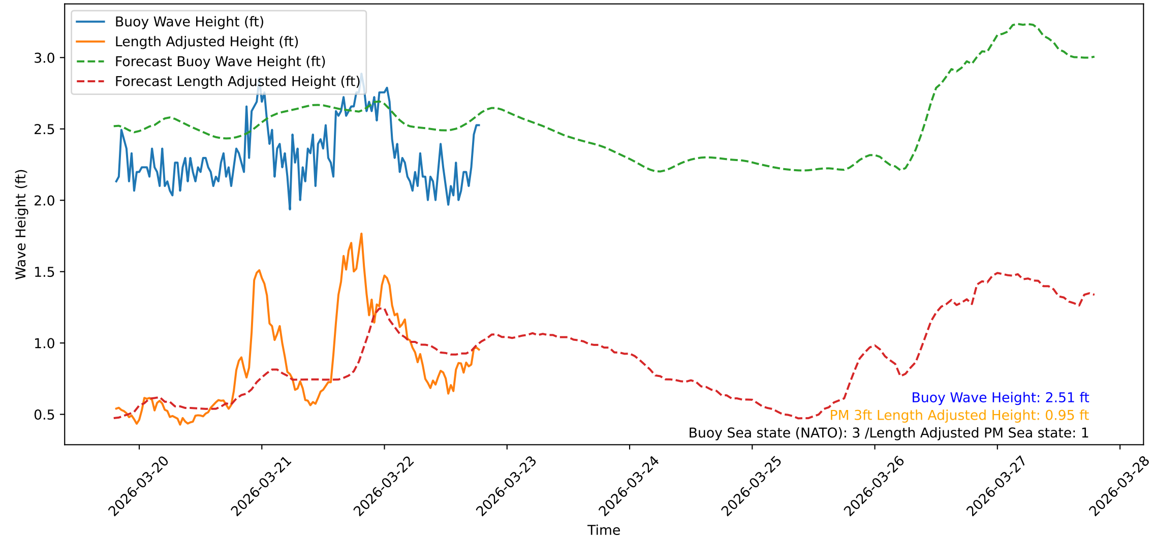
Wave Heights over Time for Green Beach at 2026-03-22 19:21:09
