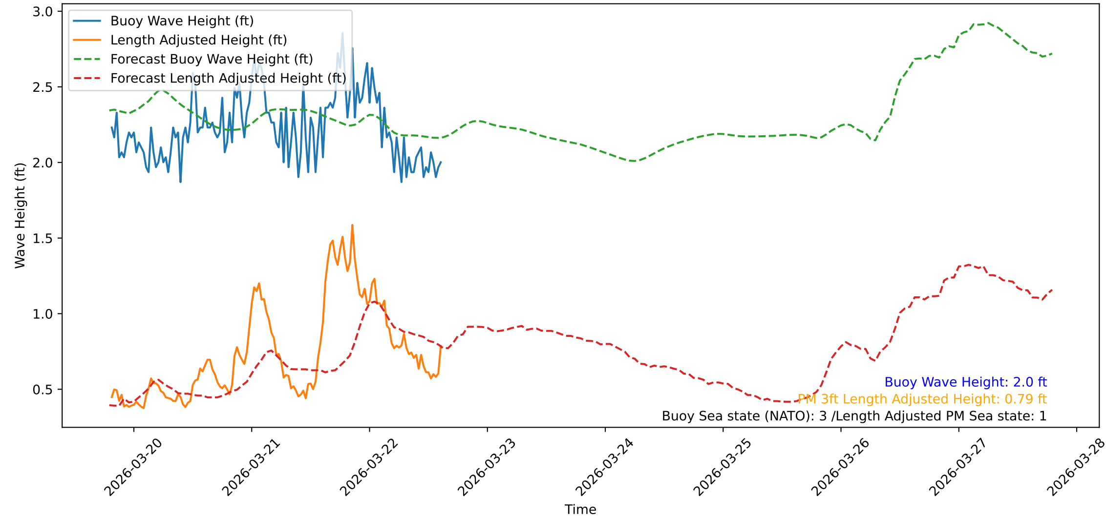
Wave Heights over Time for Red Beach at 2026-03-22 19:20:47
