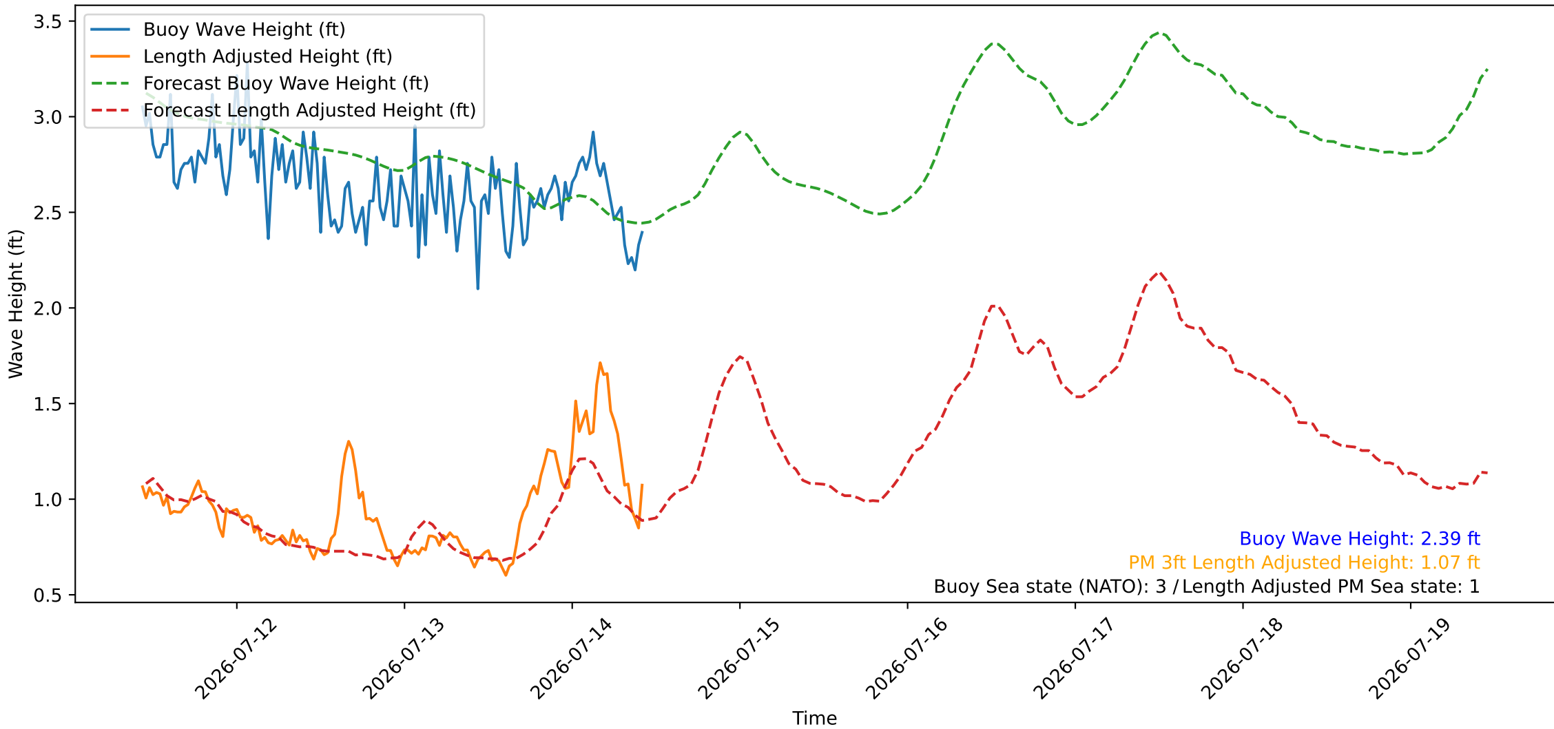
Wave Heights over Time for Oceanside Harbor at 2026-07-14 10:30:26
