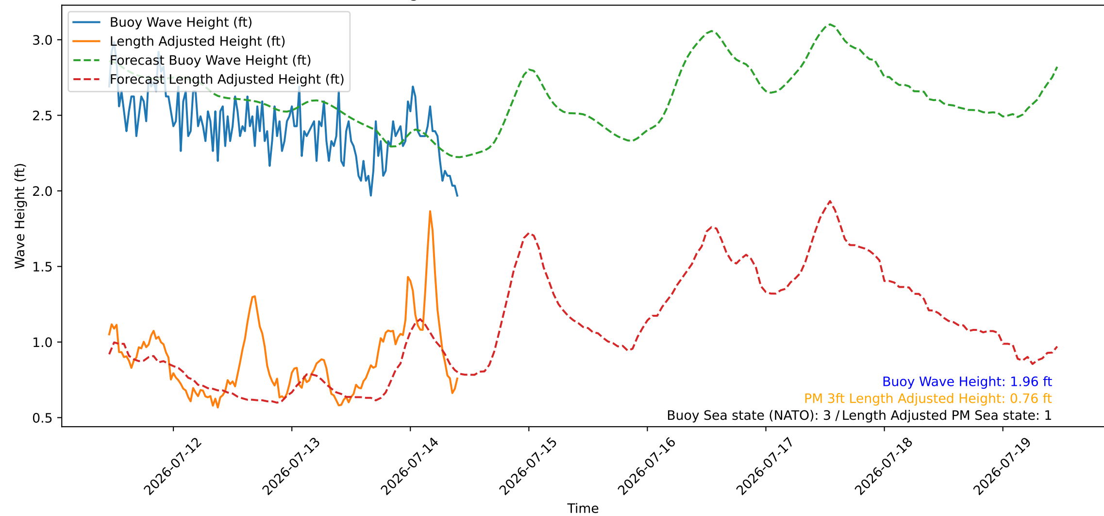
Wave Heights over Time for Red Beach at 2026-07-14 10:30:46
