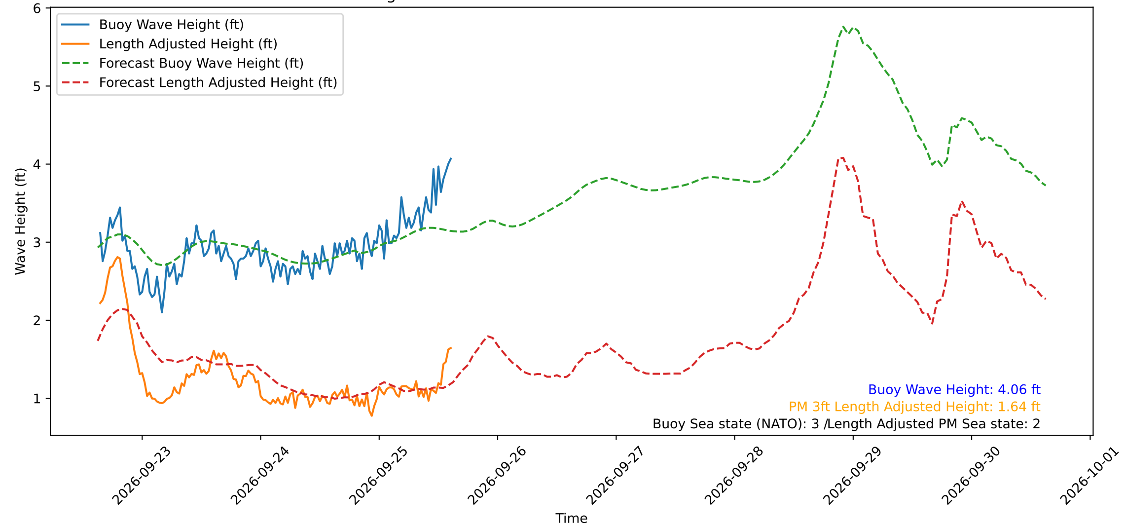
Wave Heights over Time for Green Beach at 2026-09-25 15:21:14
