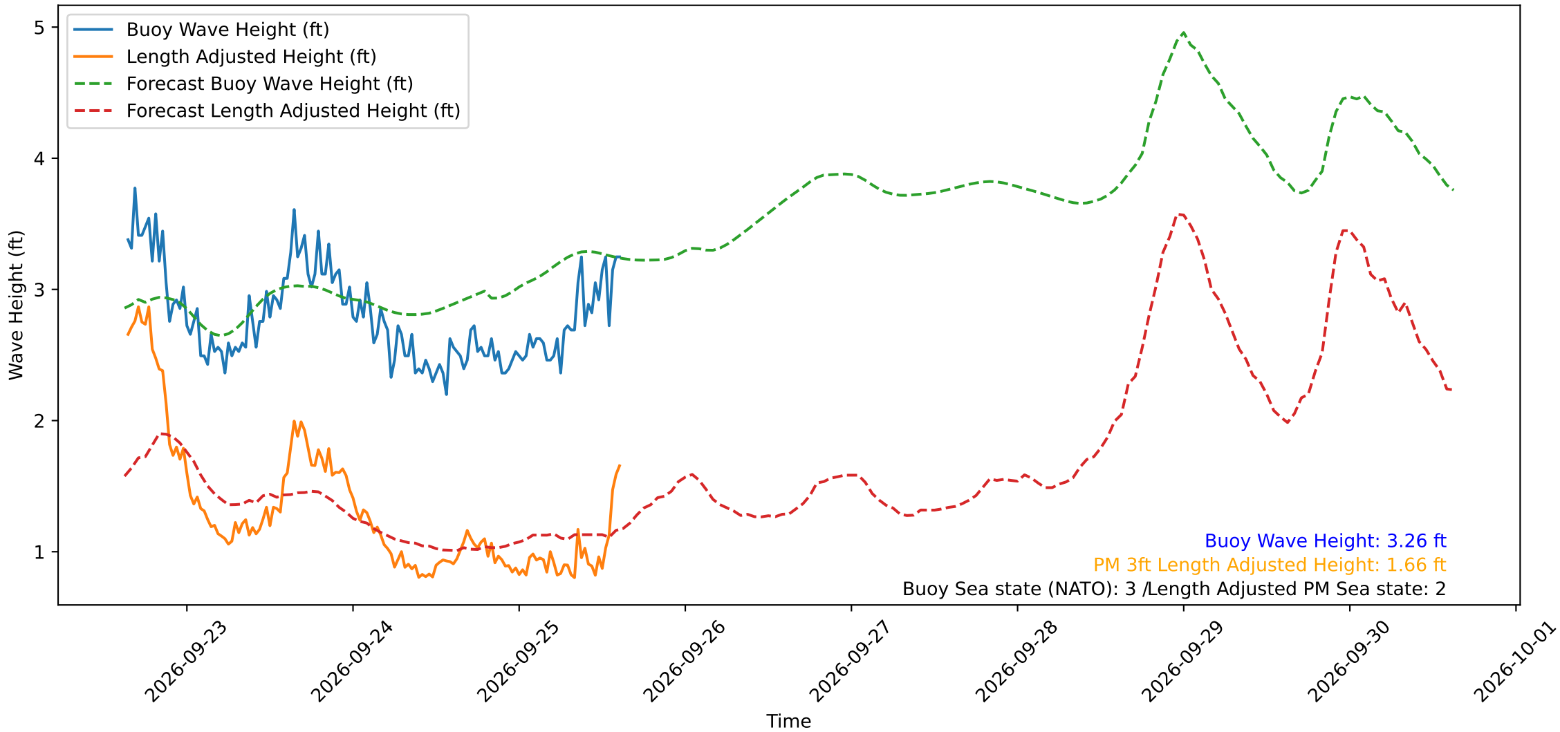
Wave Heights over Time for Oceanside Harbor at 2026-09-25 15:20:29
