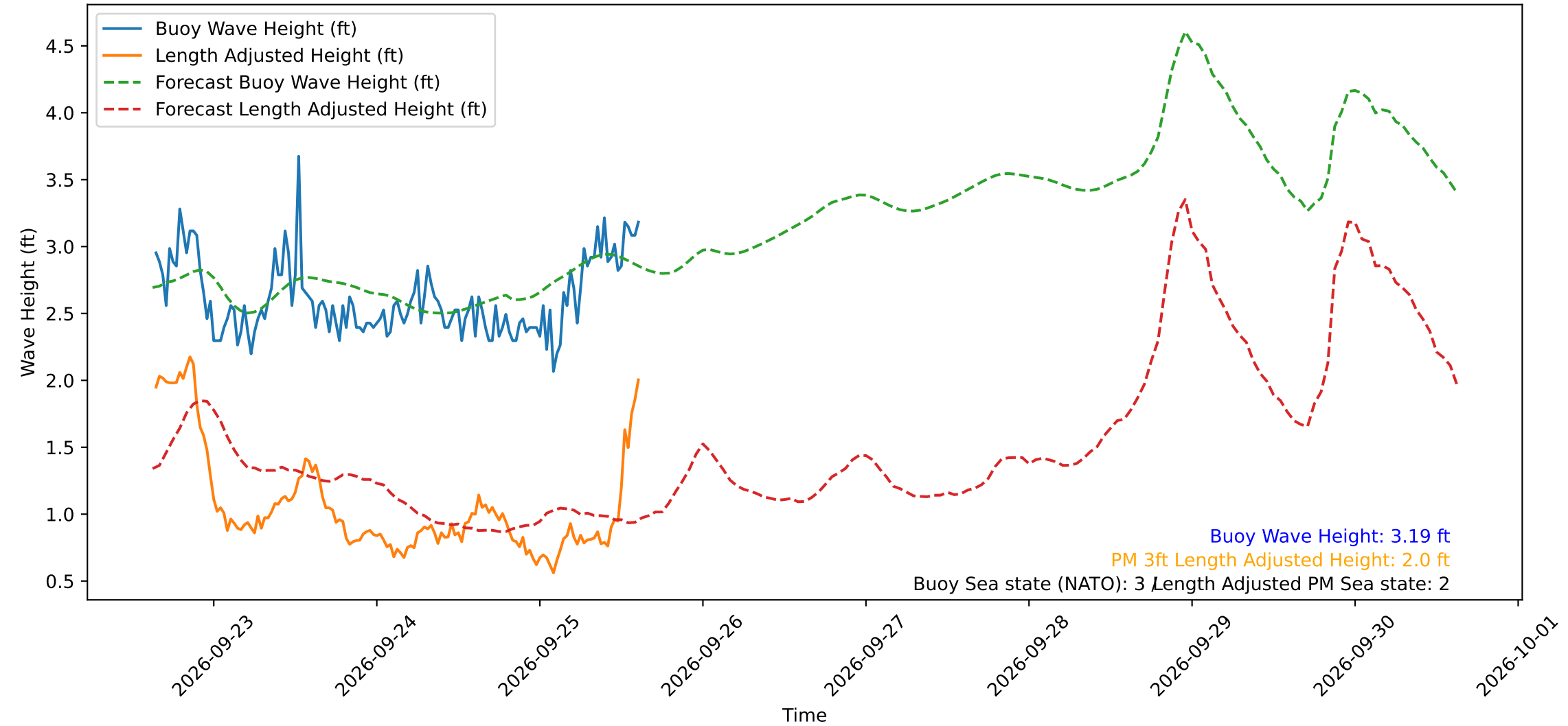
Wave Heights over Time for Red Beach at 2026-09-25 15:20:50
