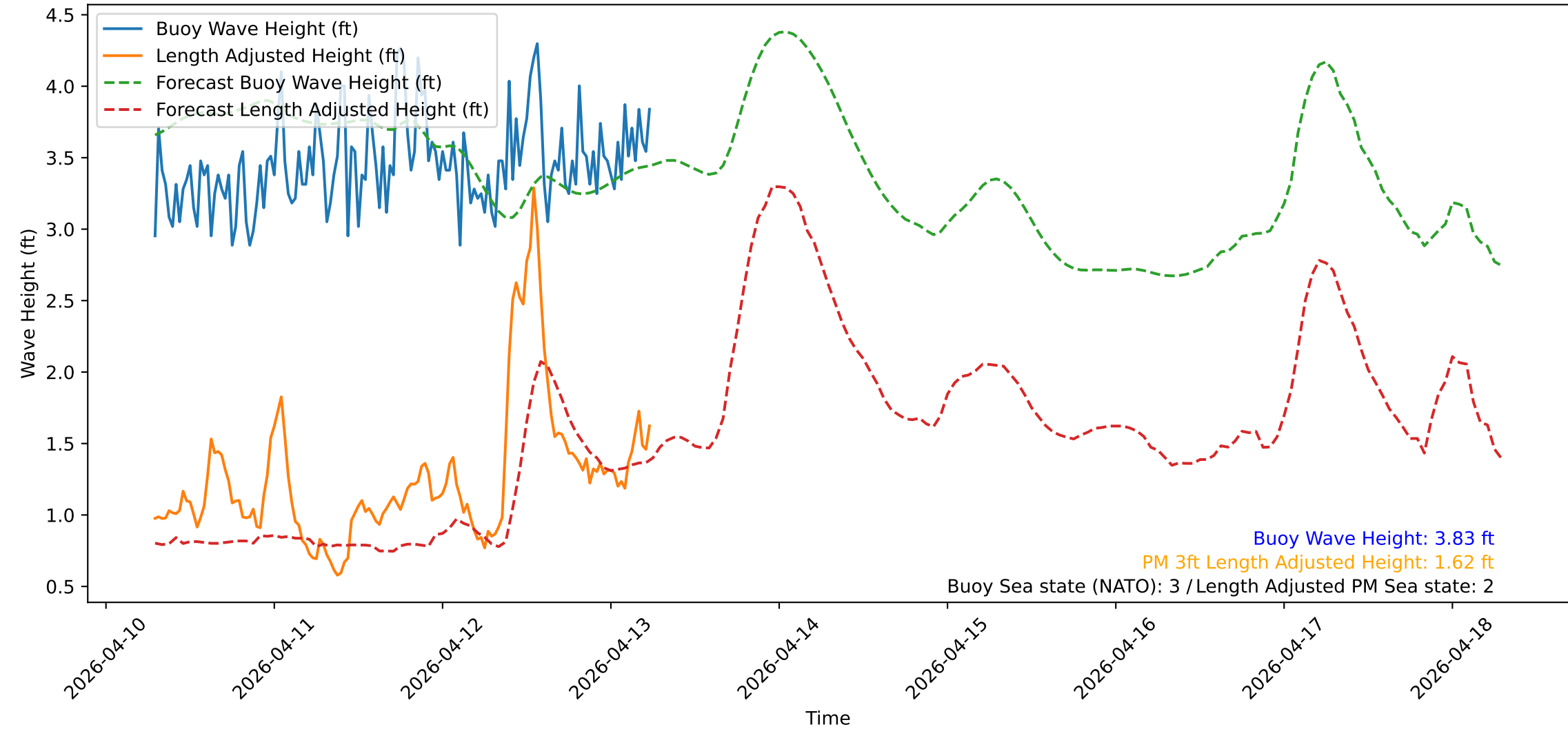
Wave Heights over Time for Red Beach at 2026-04-13 06:30:50
