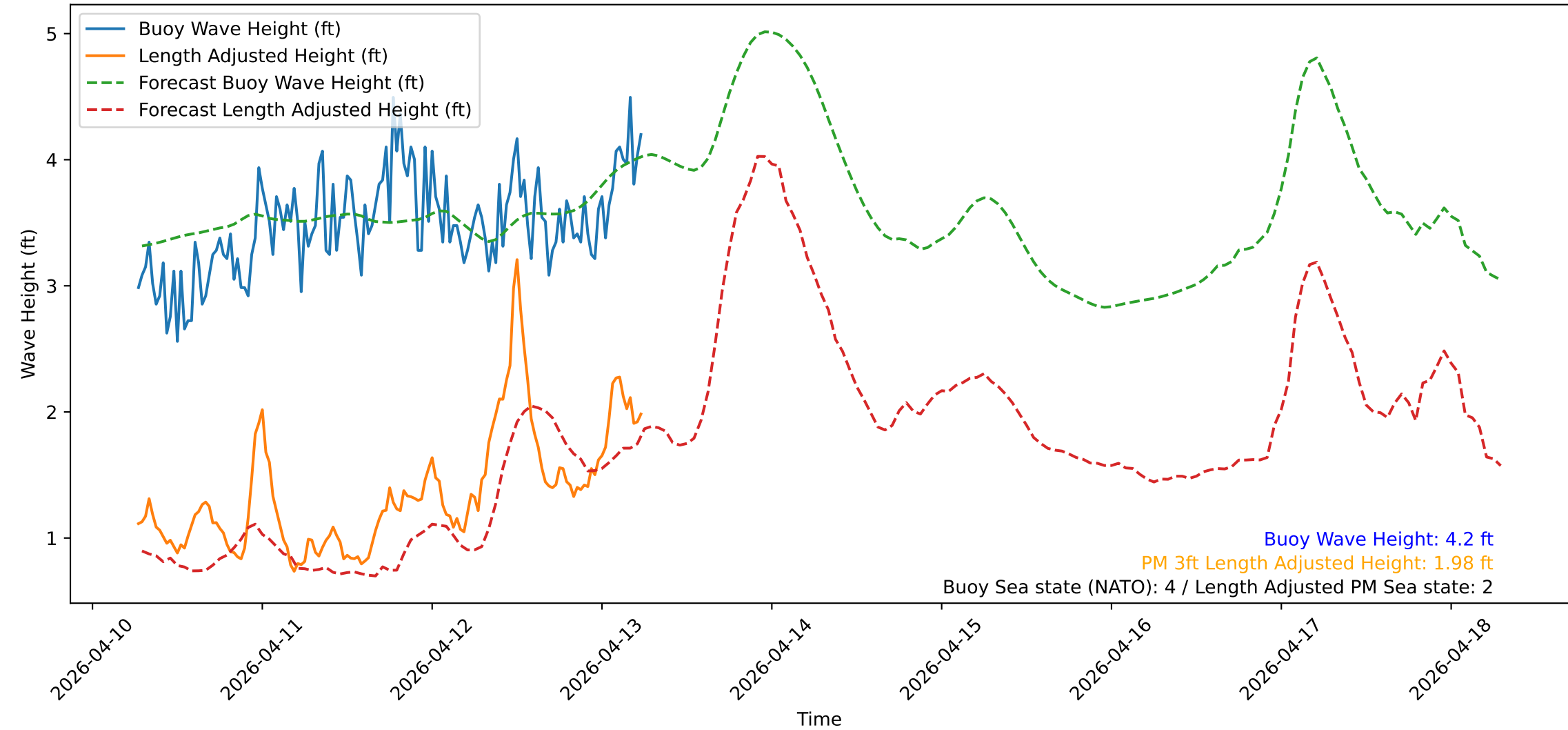
Wave Heights over Time for Green Beach at 2026-04-13 06:31:12
