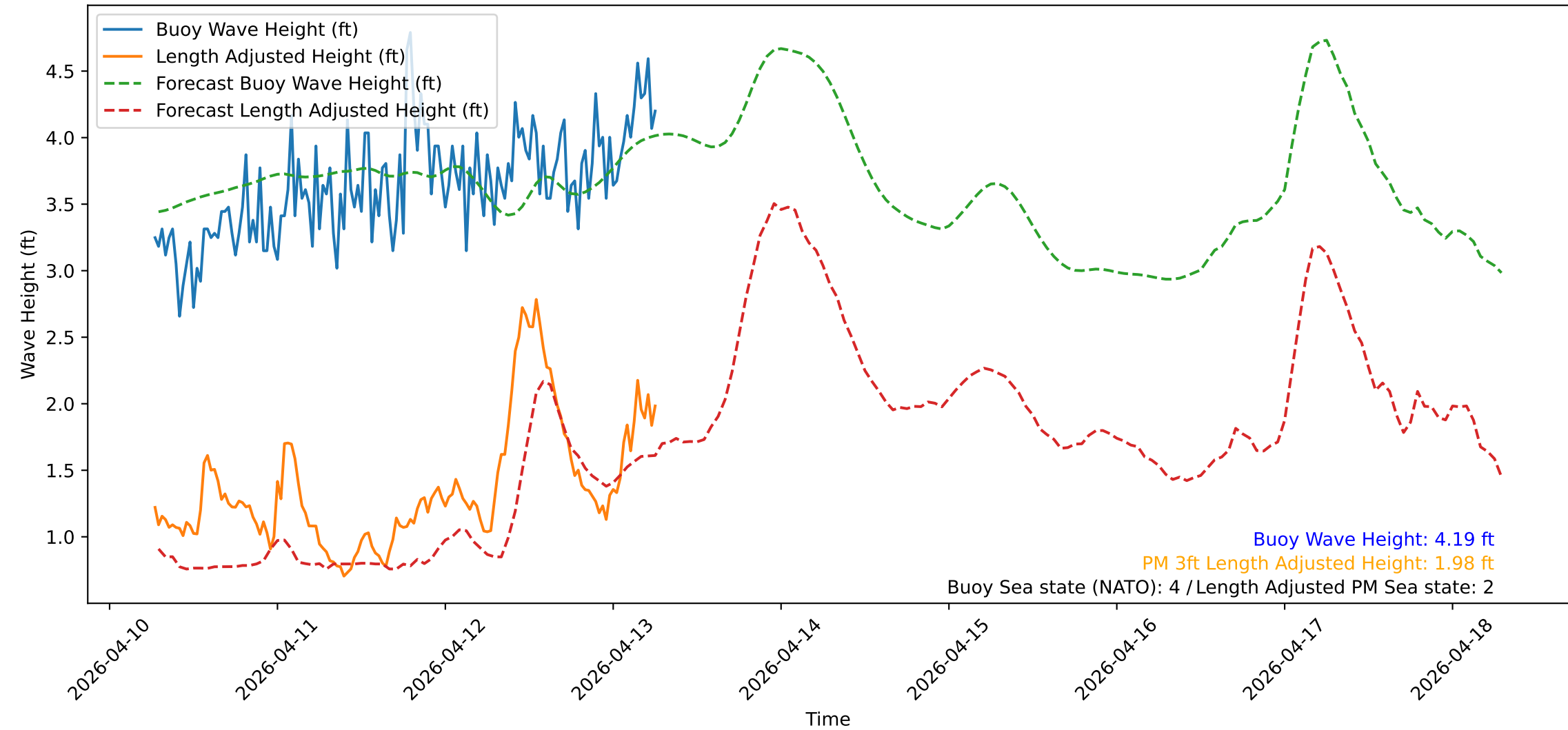
Wave Heights over Time for Oceanside Harbor at 2026-04-13 06:30:31
