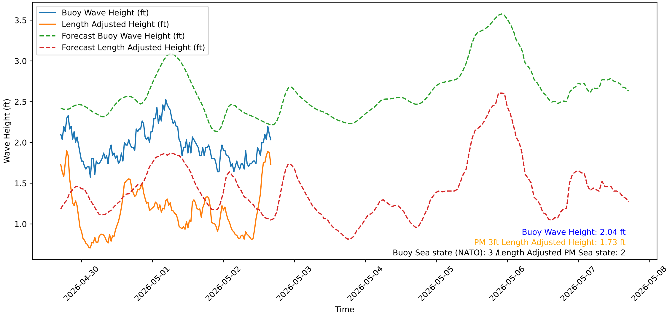
Wave Heights over Time for Red Beach at 2026-05-02 16:50:52
