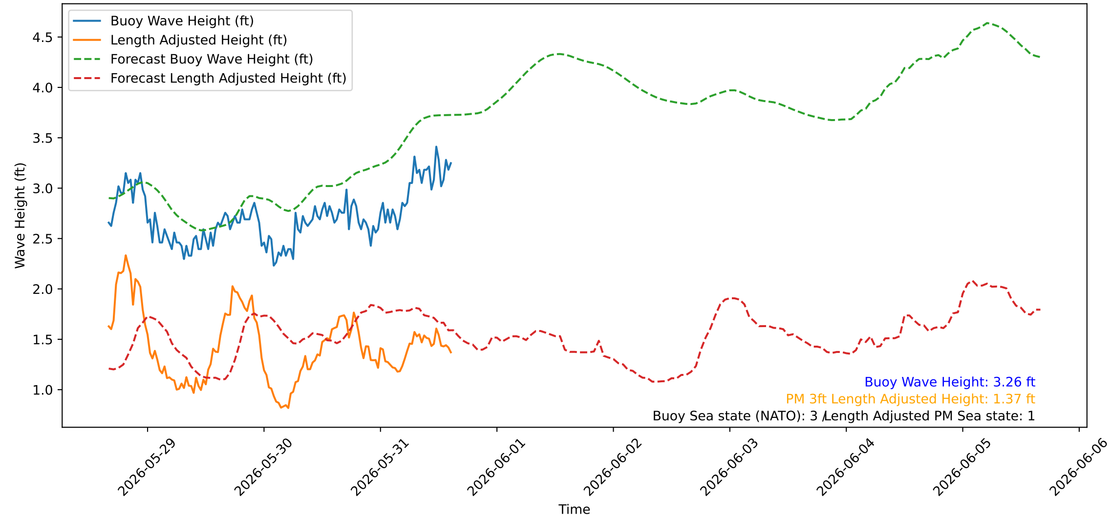
Wave Heights over Time for Red Beach at 2026-05-31 15:50:46
