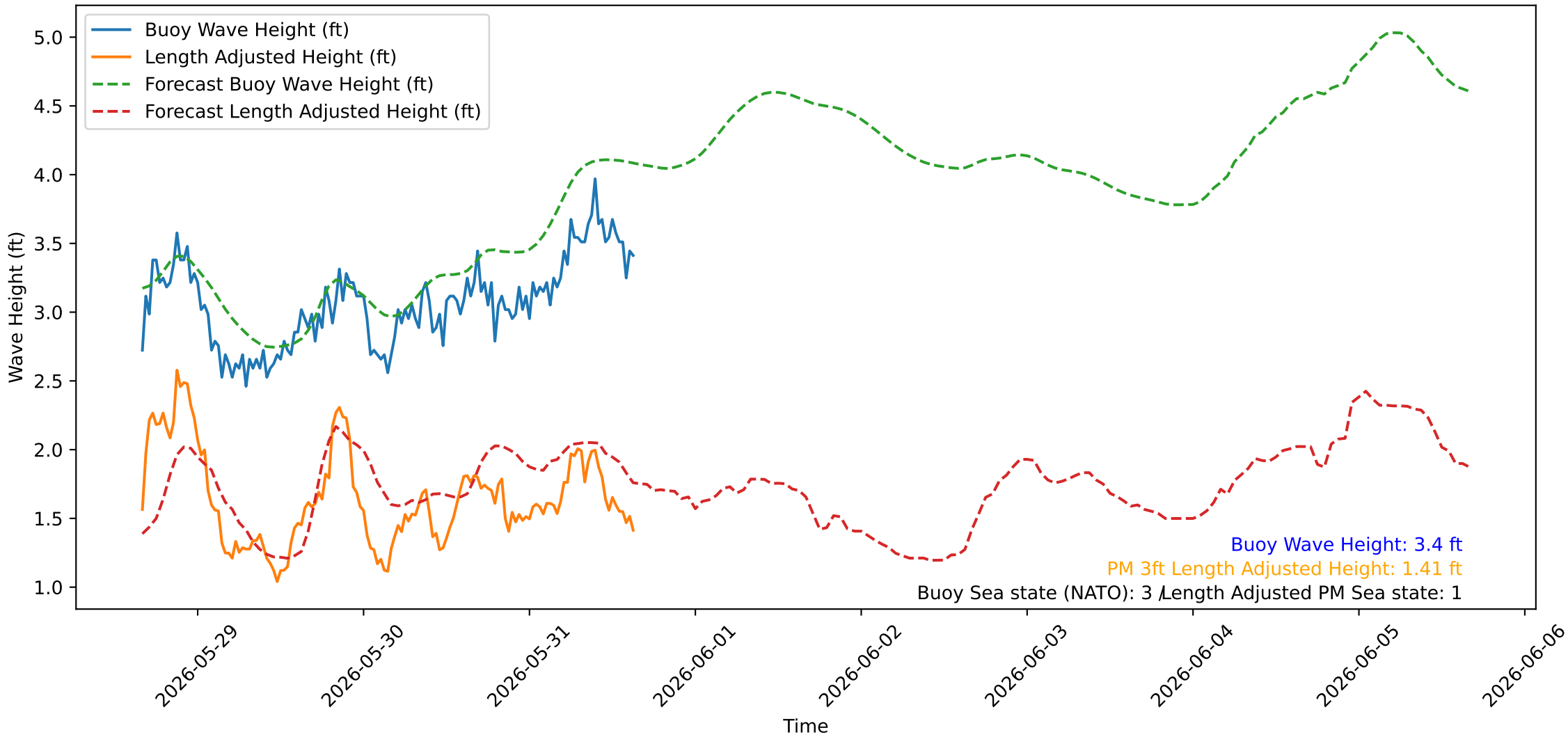
Wave Heights over Time for Green Beach at 2026-05-31 15:51:09
