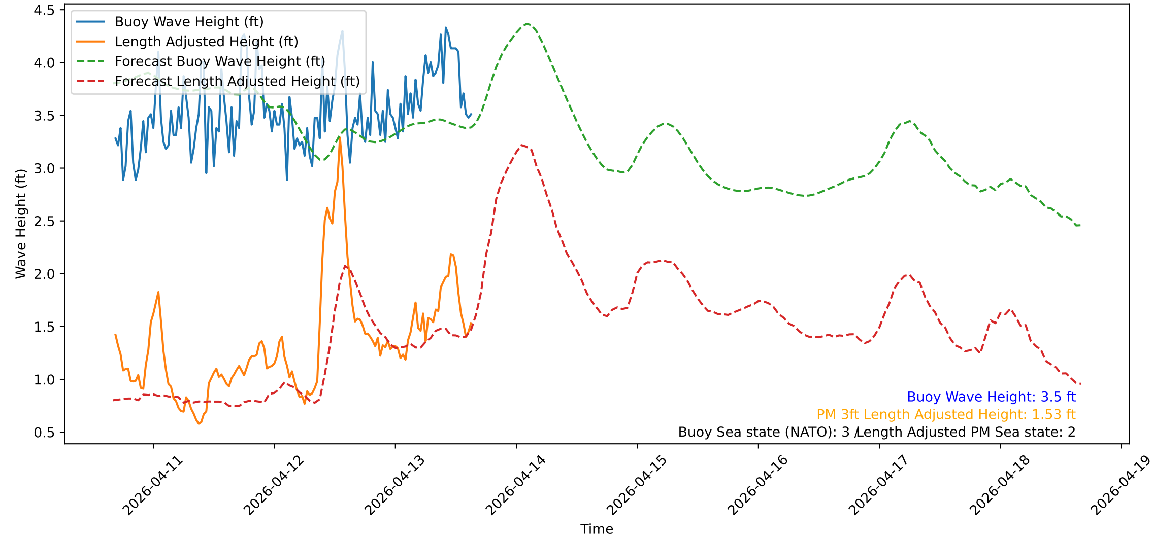
Wave Heights over Time for Red Beach at 2026-04-13 16:00:50
