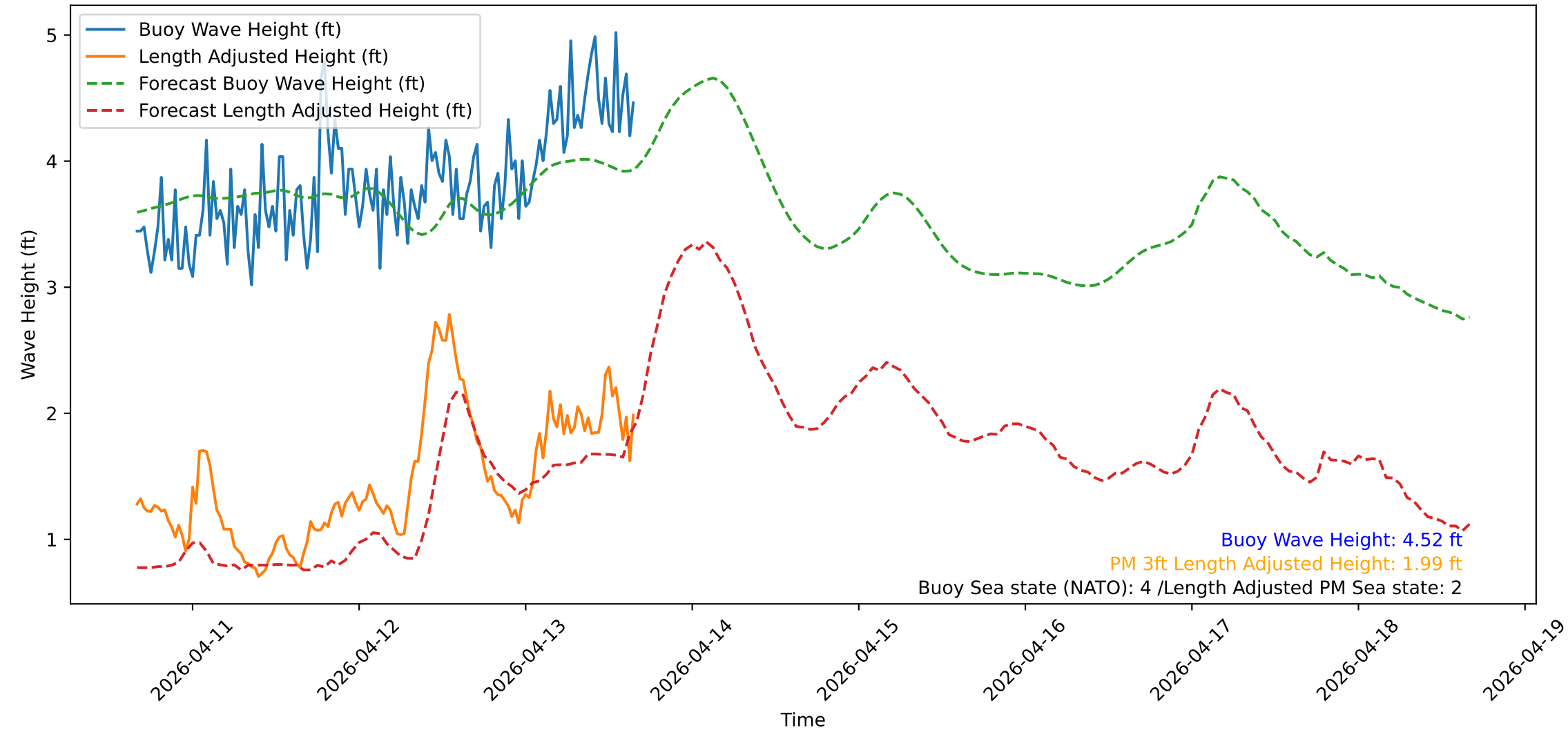
Wave Heights over Time for Oceanside Harbor at 2026-04-13 16:00:31
