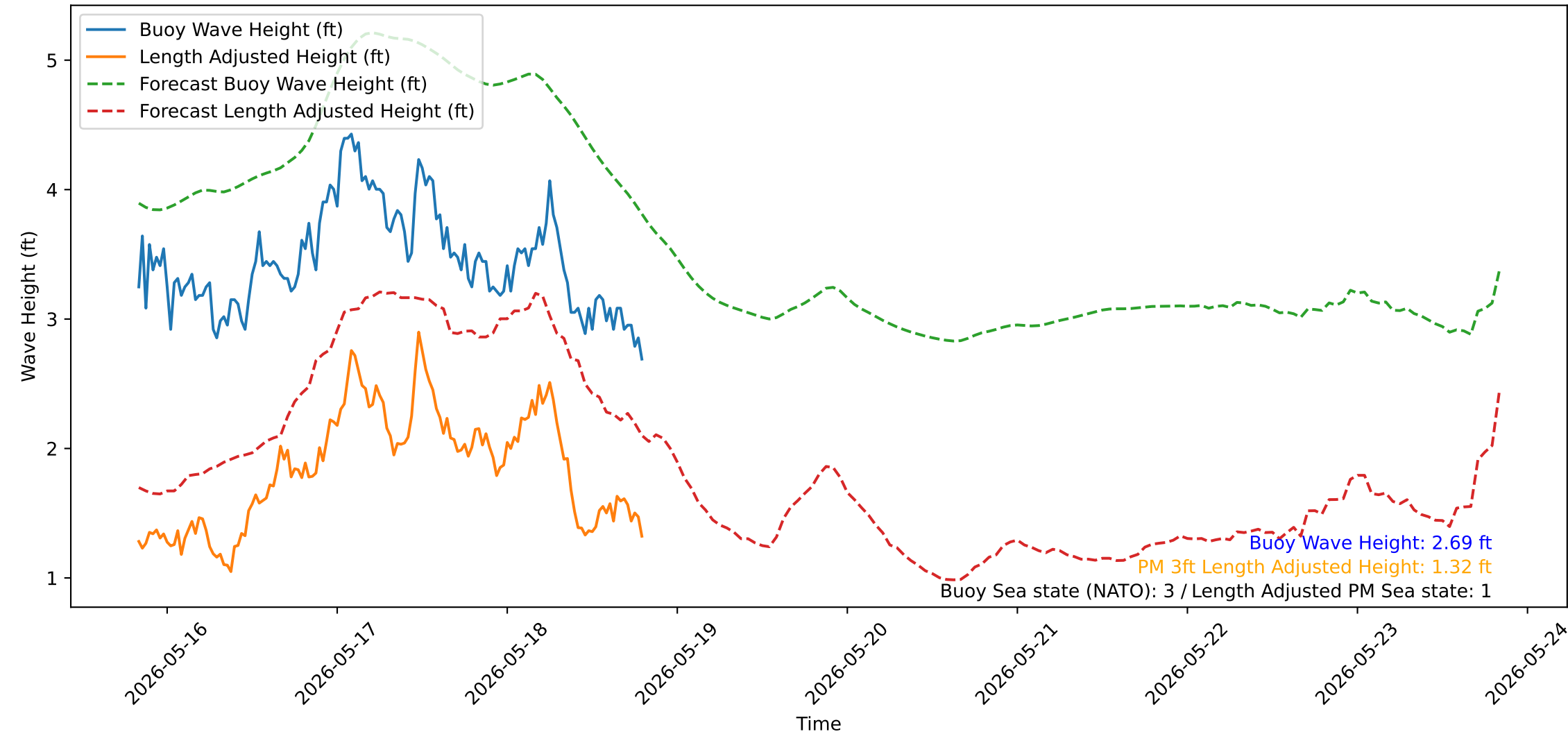
Wave Heights over Time for Green Beach at 2026-05-18 19:51:16
