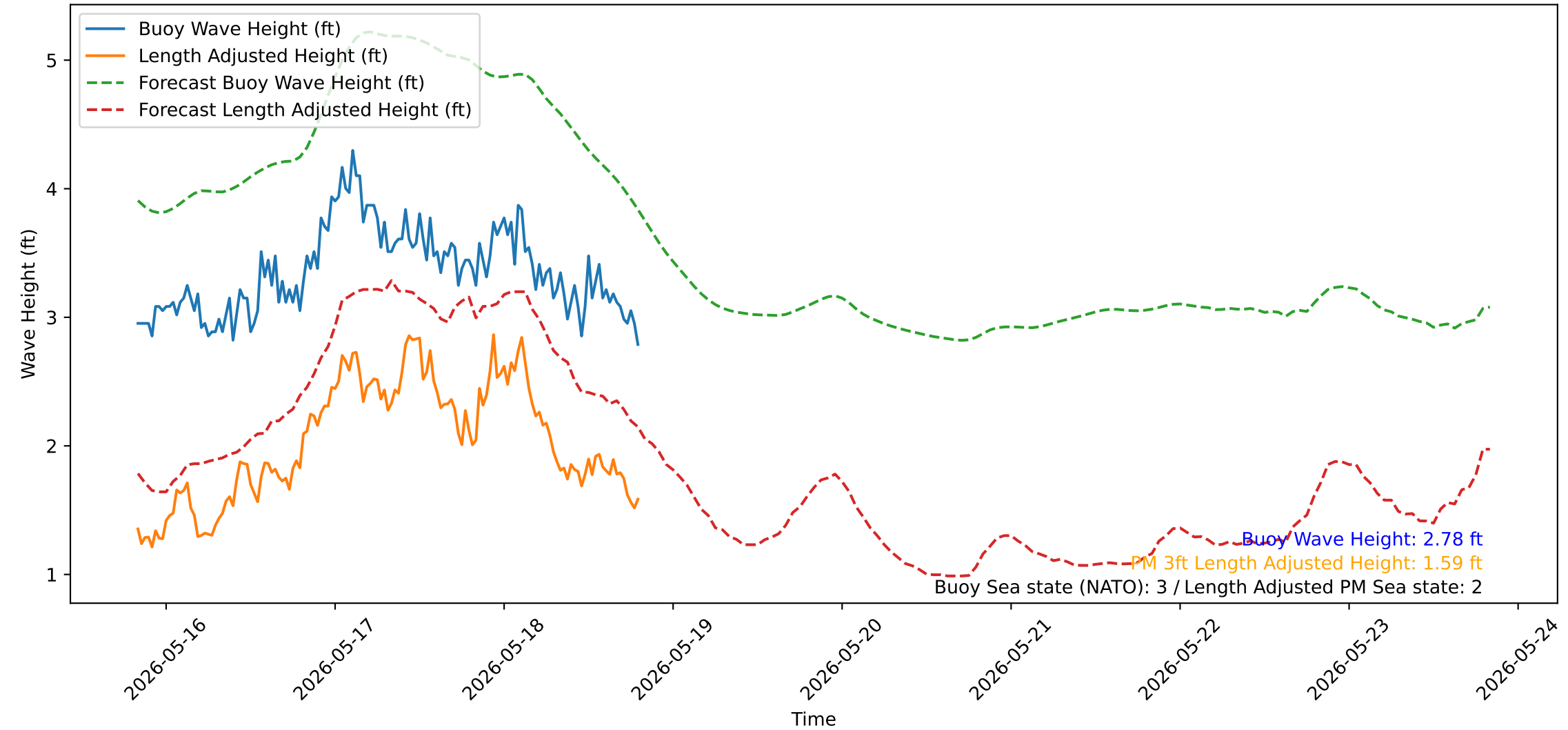
Wave Heights over Time for Oceanside Harbor at 2026-05-18 19:50:31
