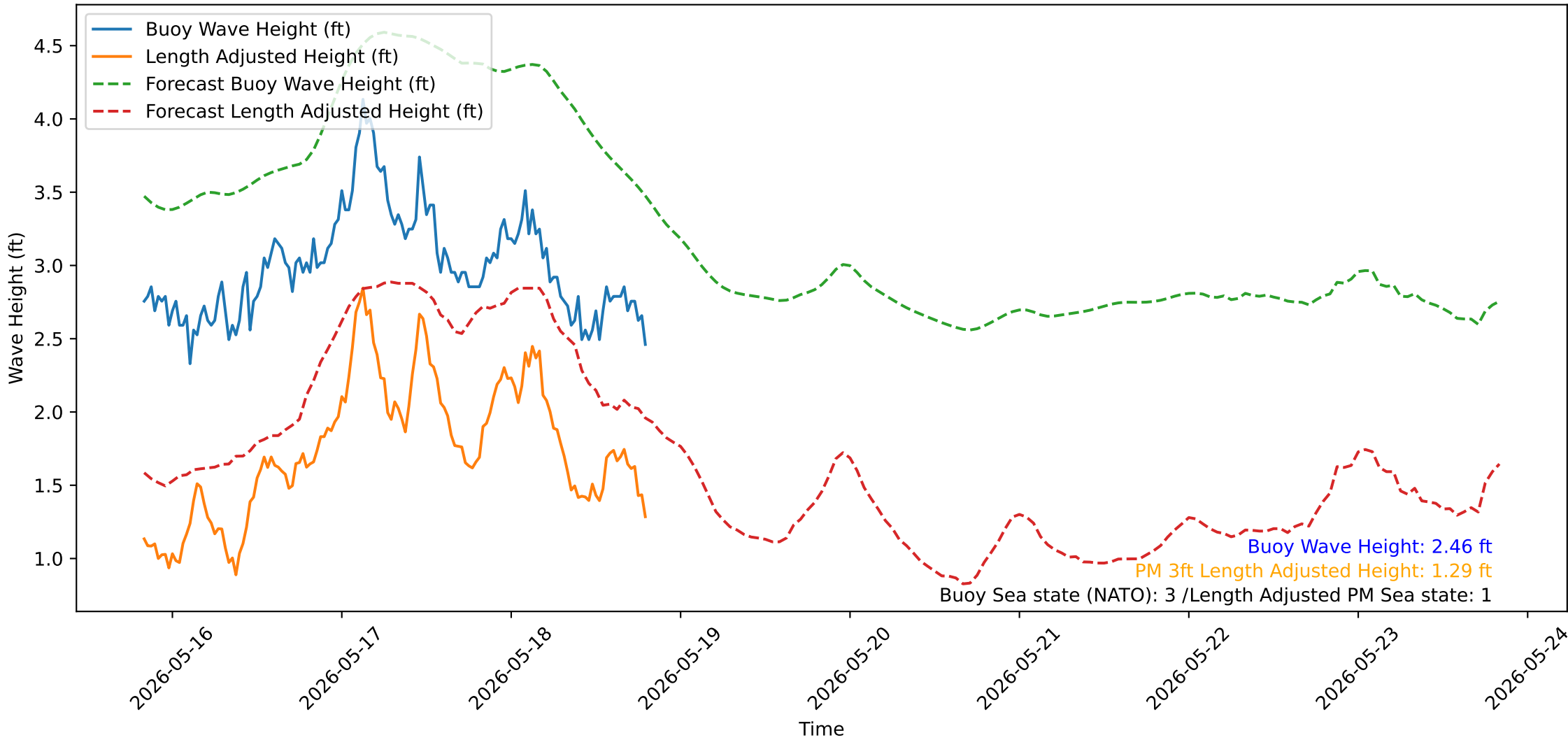
Wave Heights over Time for Red Beach at 2026-05-18 19:50:52
