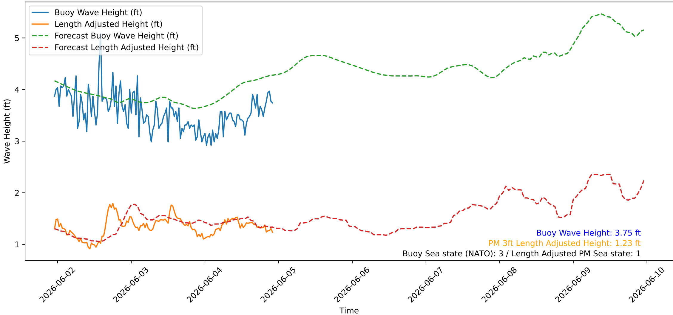
Wave Heights over Time for Oceanside Harbor at 2026-06-04 22:50:26
