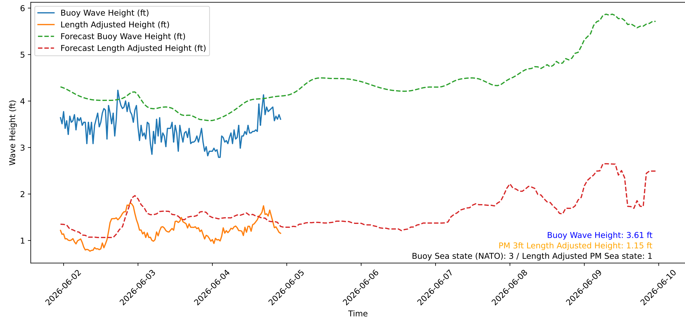
Wave Heights over Time for Green Beach at 2026-06-04 22:51:09
