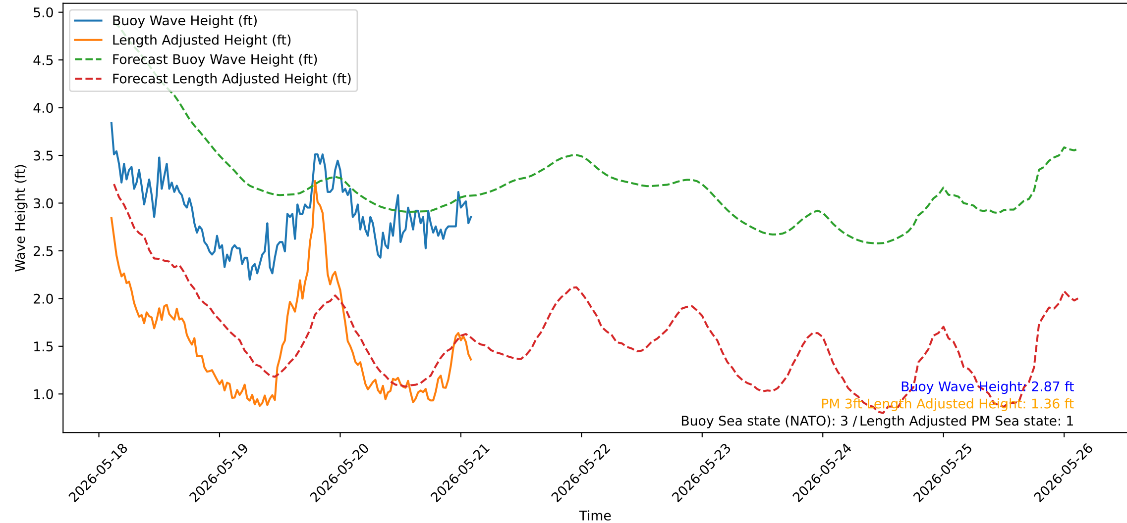
Wave Heights over Time for Oceanside Harbor at 2026-05-21 02:30:31
