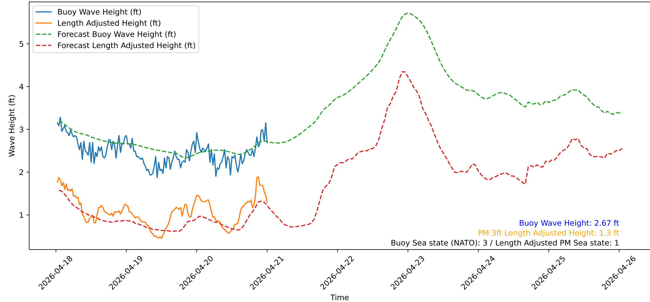
Wave Heights over Time for Green Beach at 2026-04-21 00:41:13
