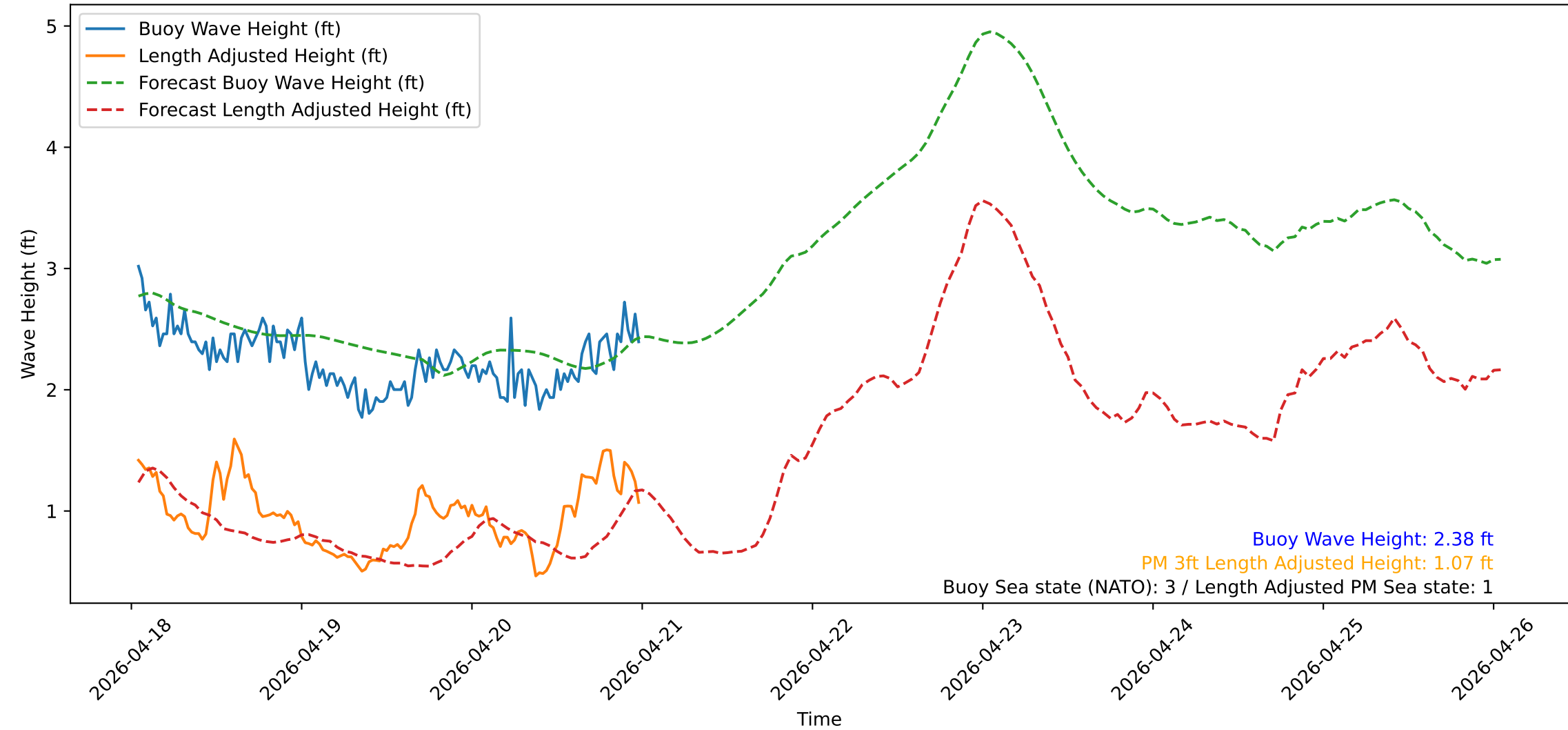
Wave Heights over Time for Red Beach at 2026-04-21 00:40:51
