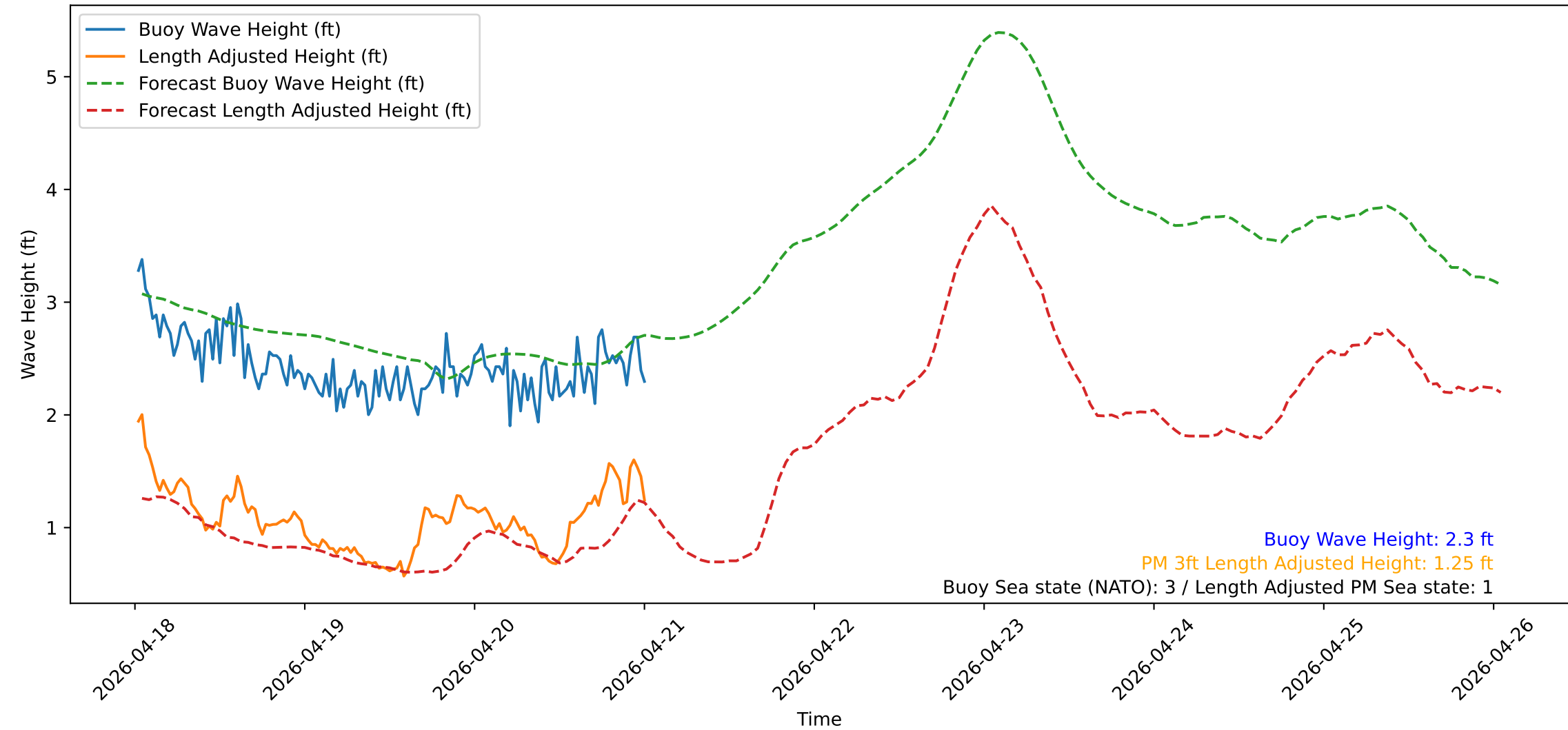
Wave Heights over Time for Oceanside Harbor at 2026-04-21 00:40:31
