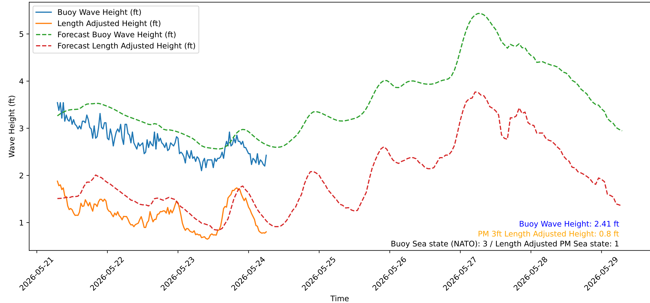
Wave Heights over Time for Green Beach at 2026-05-24 07:01:15
