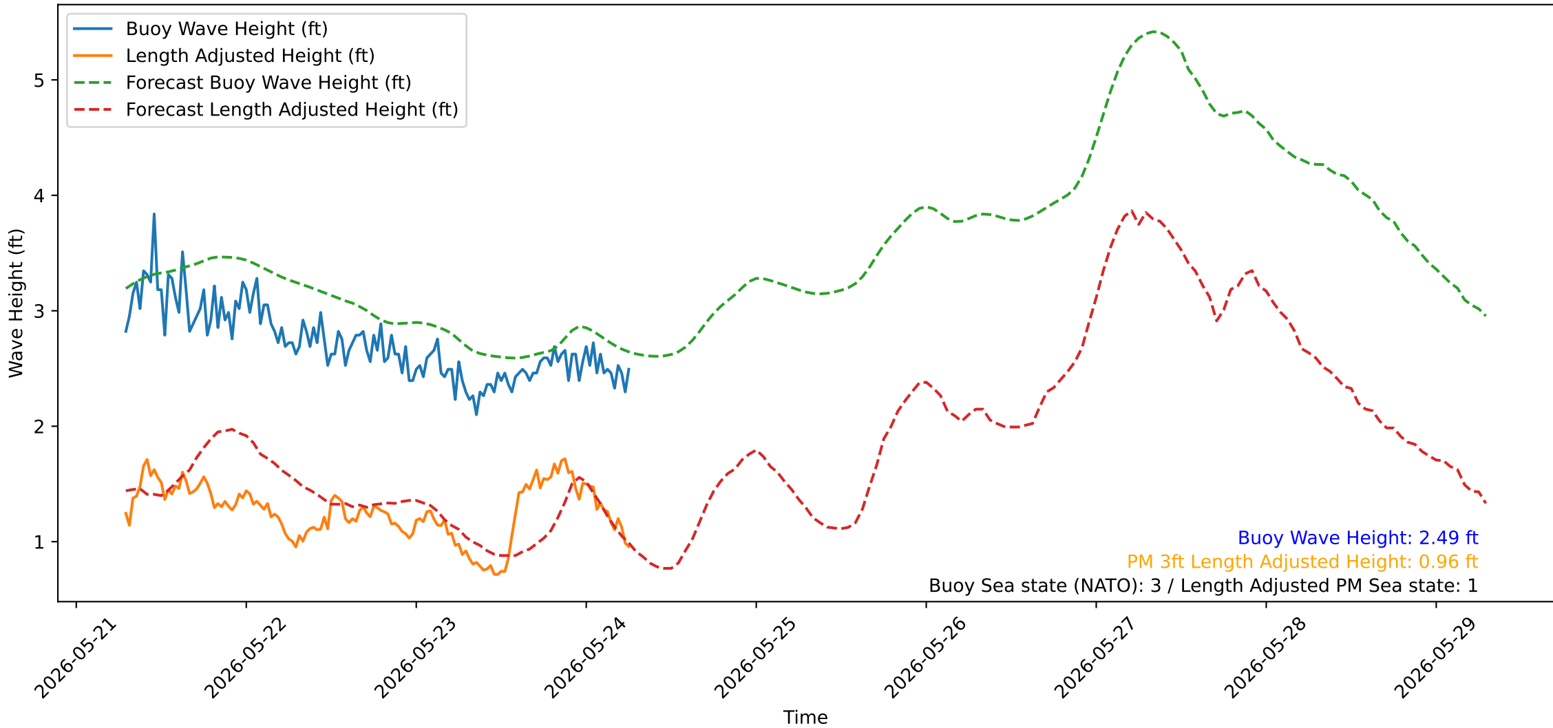
Wave Heights over Time for Oceanside Harbor at 2026-05-24 07:00:32
