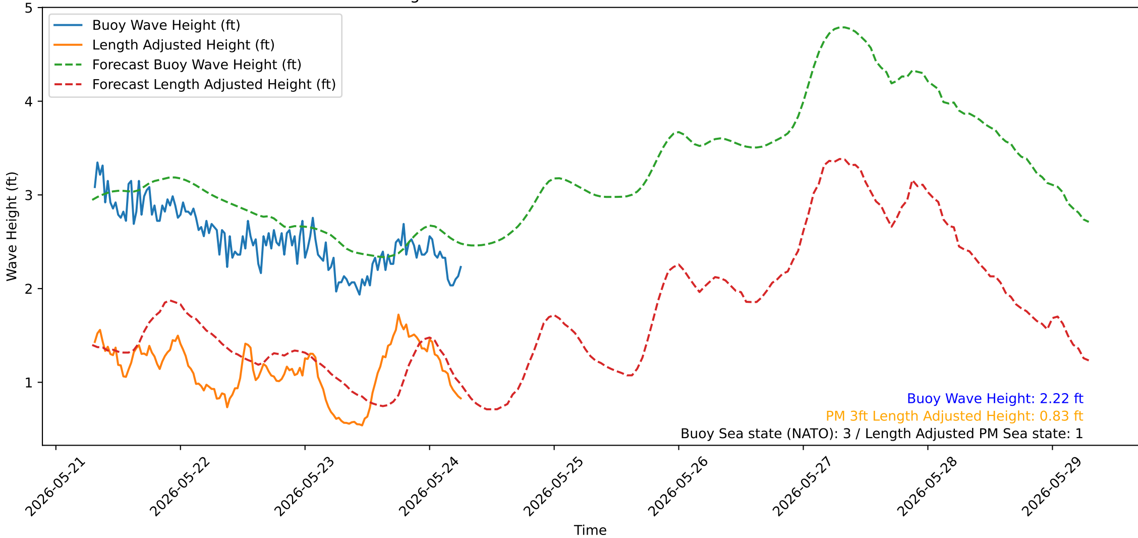
Wave Heights over Time for Red Beach at 2026-05-24 07:00:52
