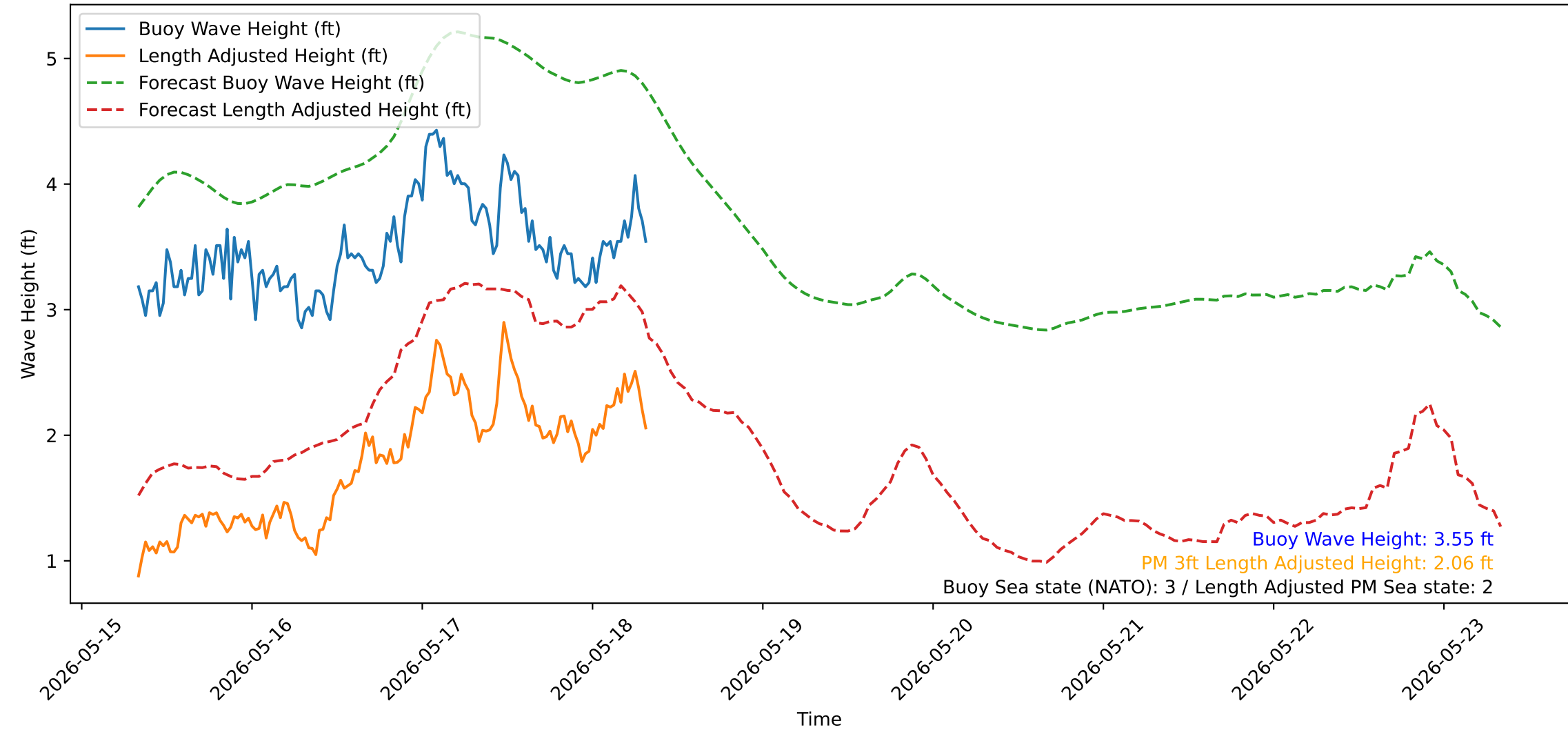
Wave Heights over Time for Green Beach at 2026-05-18 08:11:14
