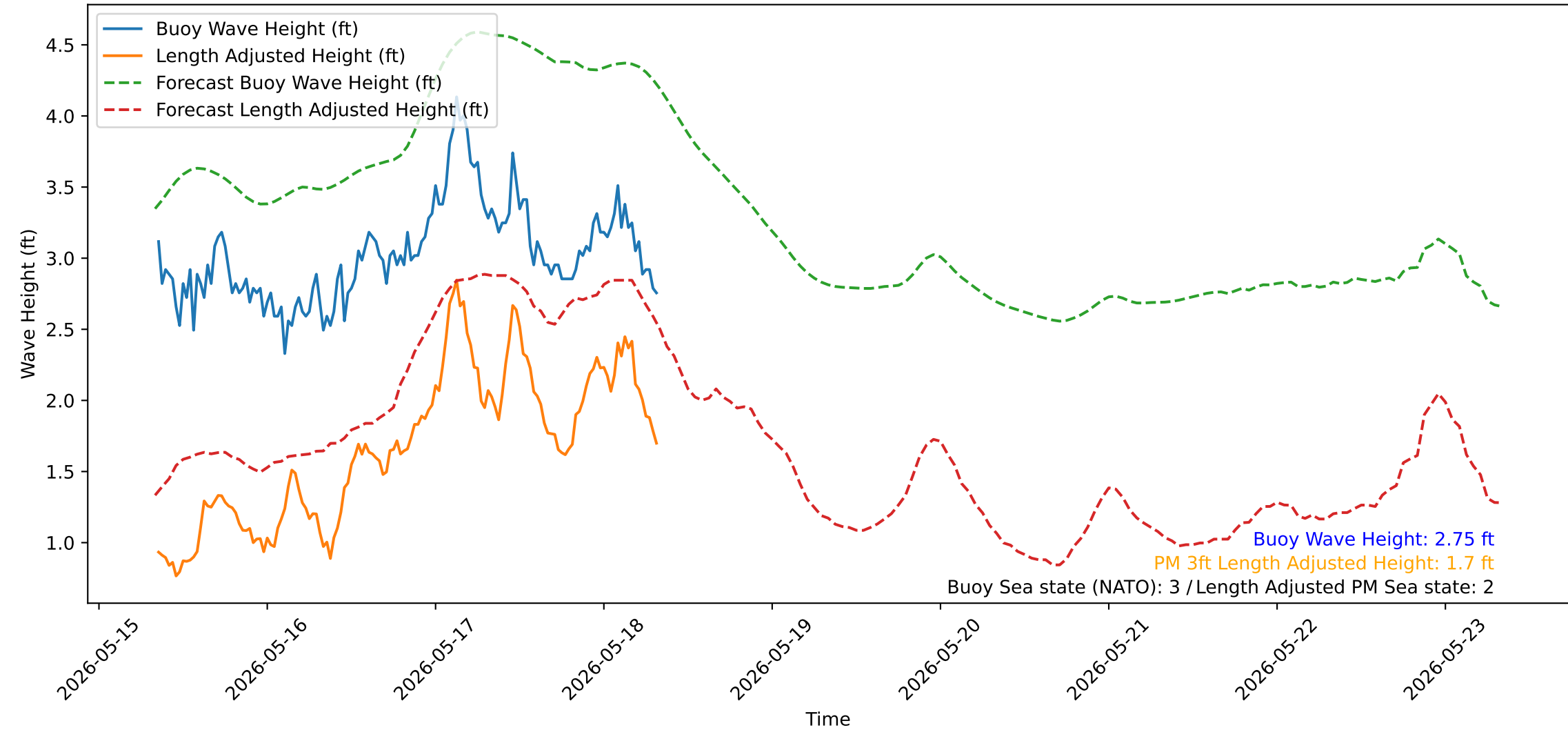
Wave Heights over Time for Red Beach at 2026-05-18 08:10:51
