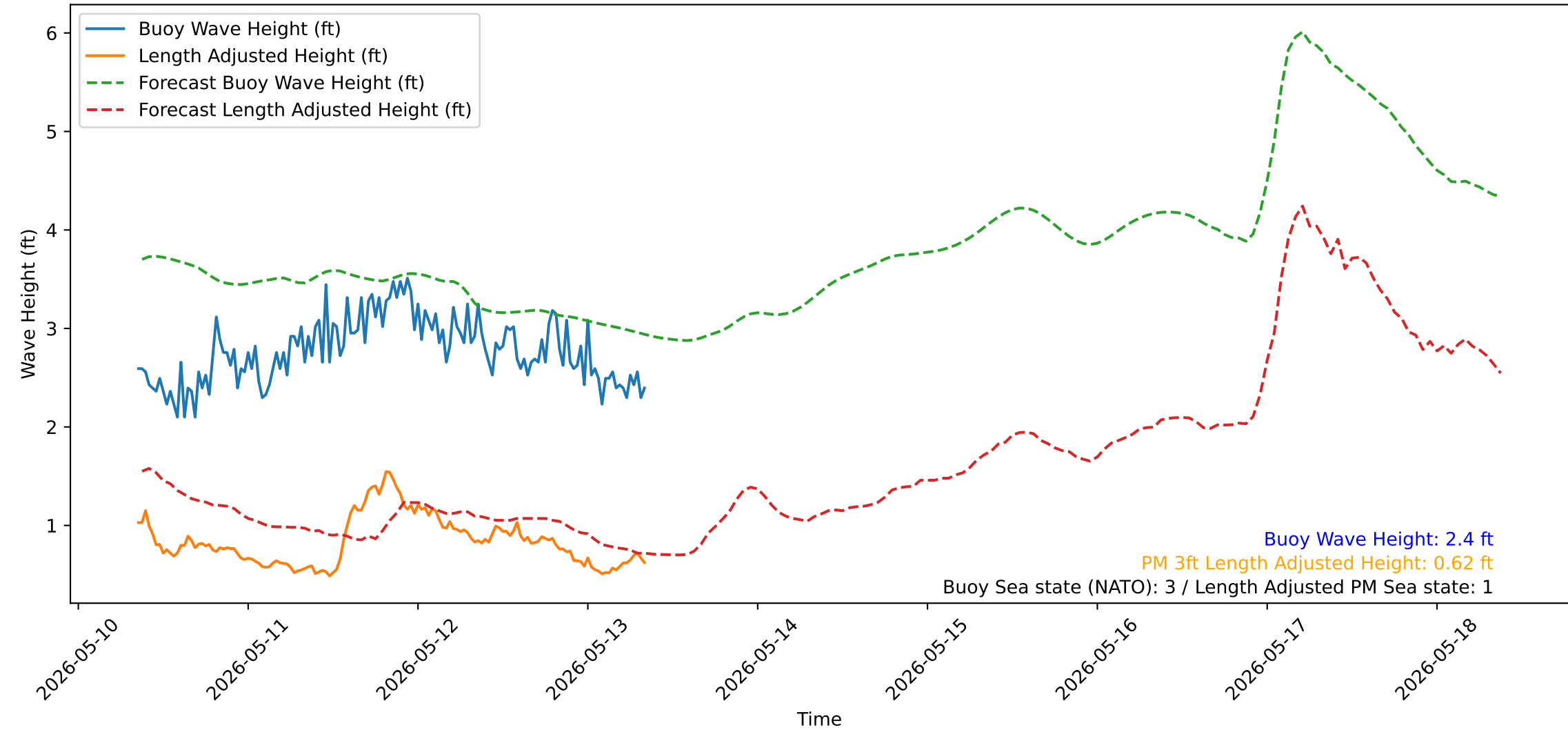
Wave Heights over Time for Green Beach at 2026-05-13 08:41:14
