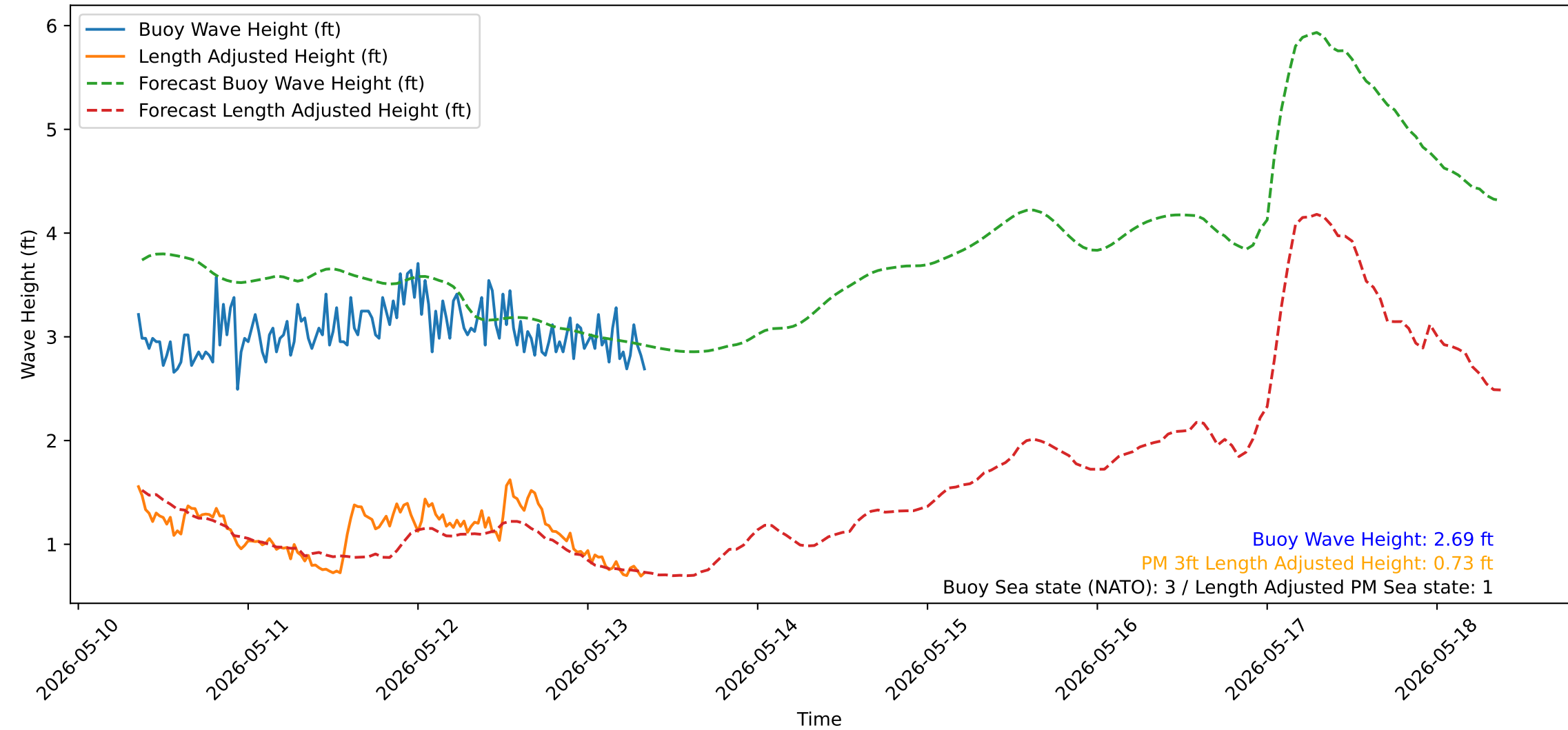
Wave Heights over Time for Oceanside Harbor at 2026-05-13 08:40:32
