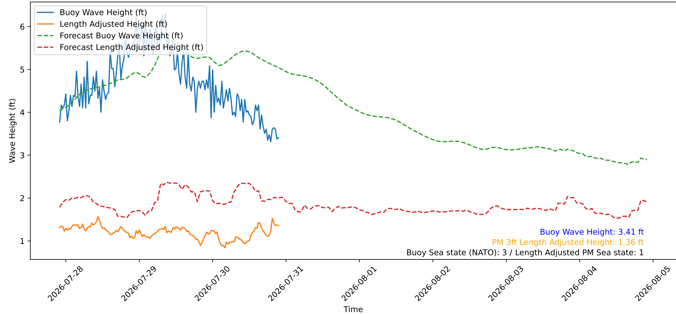
Wave Heights over Time for Green Beach at 2026-07-30 22:11:08
