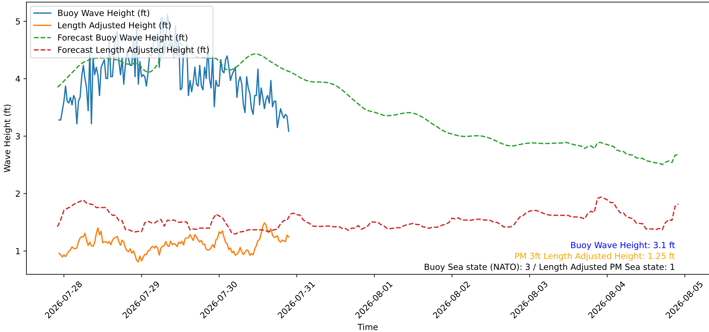
Wave Heights over Time for Red Beach at 2026-07-30 22:10:46
