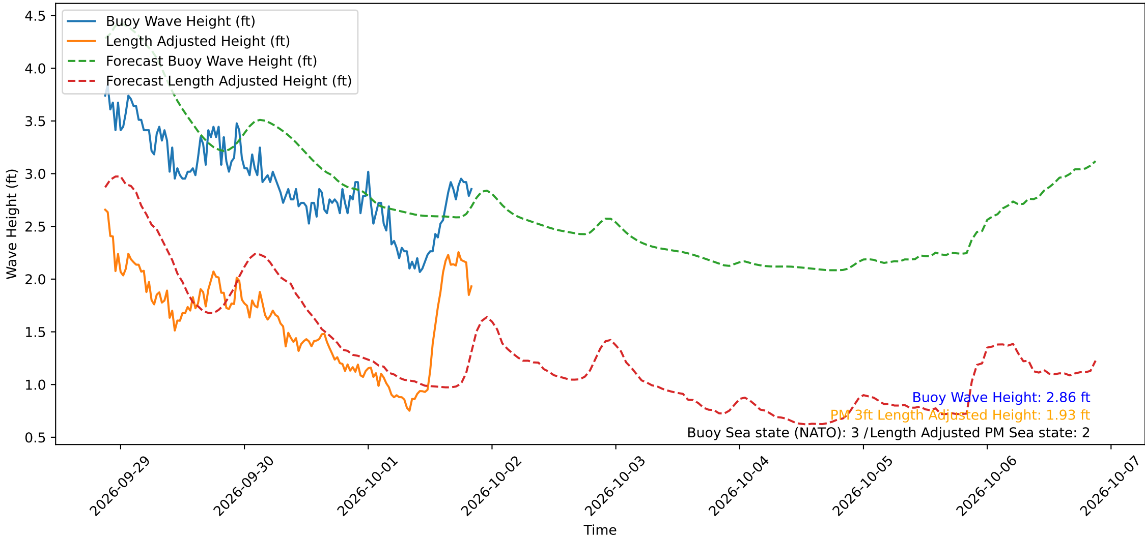
Wave Heights over Time for Red Beach at 2026-10-01 20:40:50
