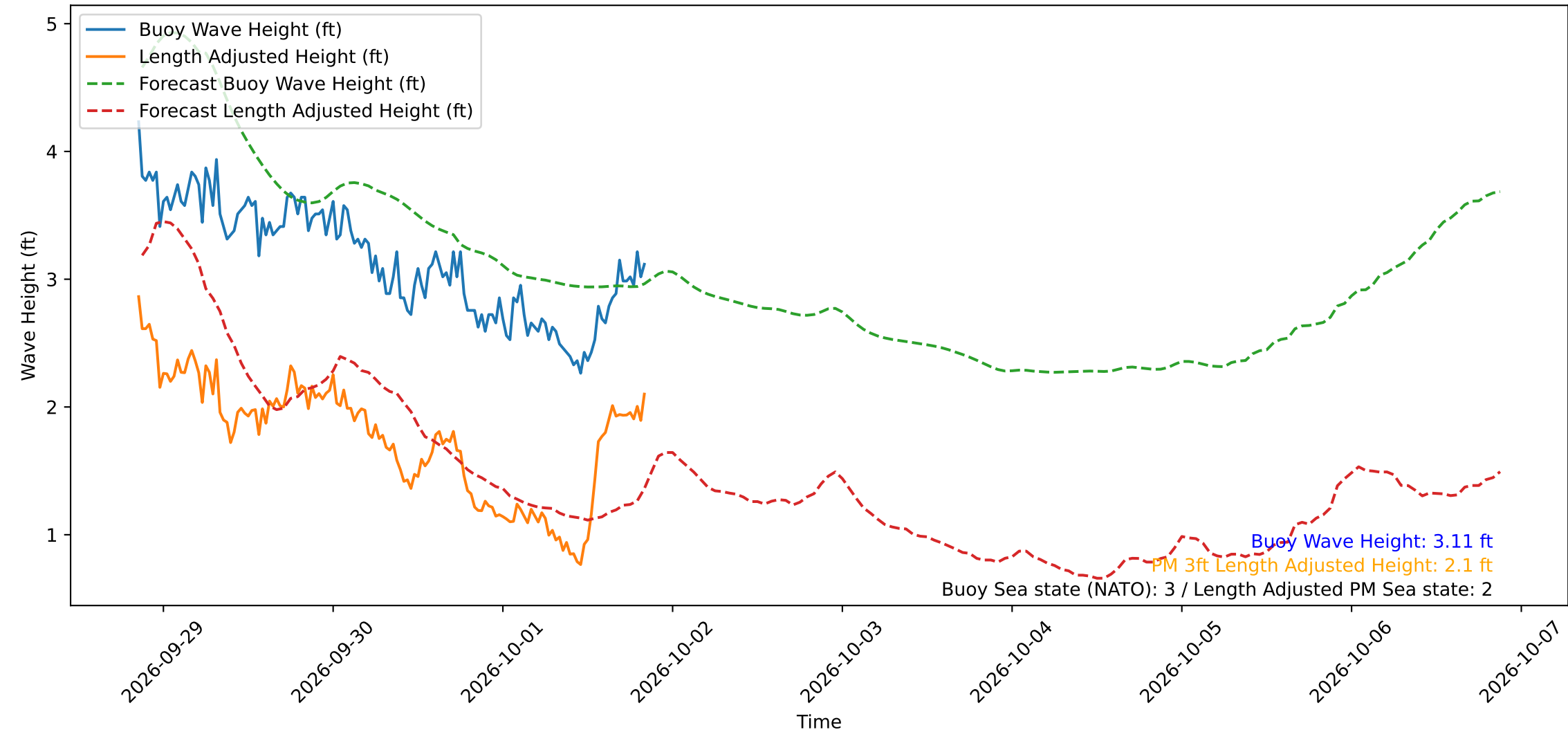
Wave Heights over Time for Oceanside Harbor at 2026-10-01 20:40:30
