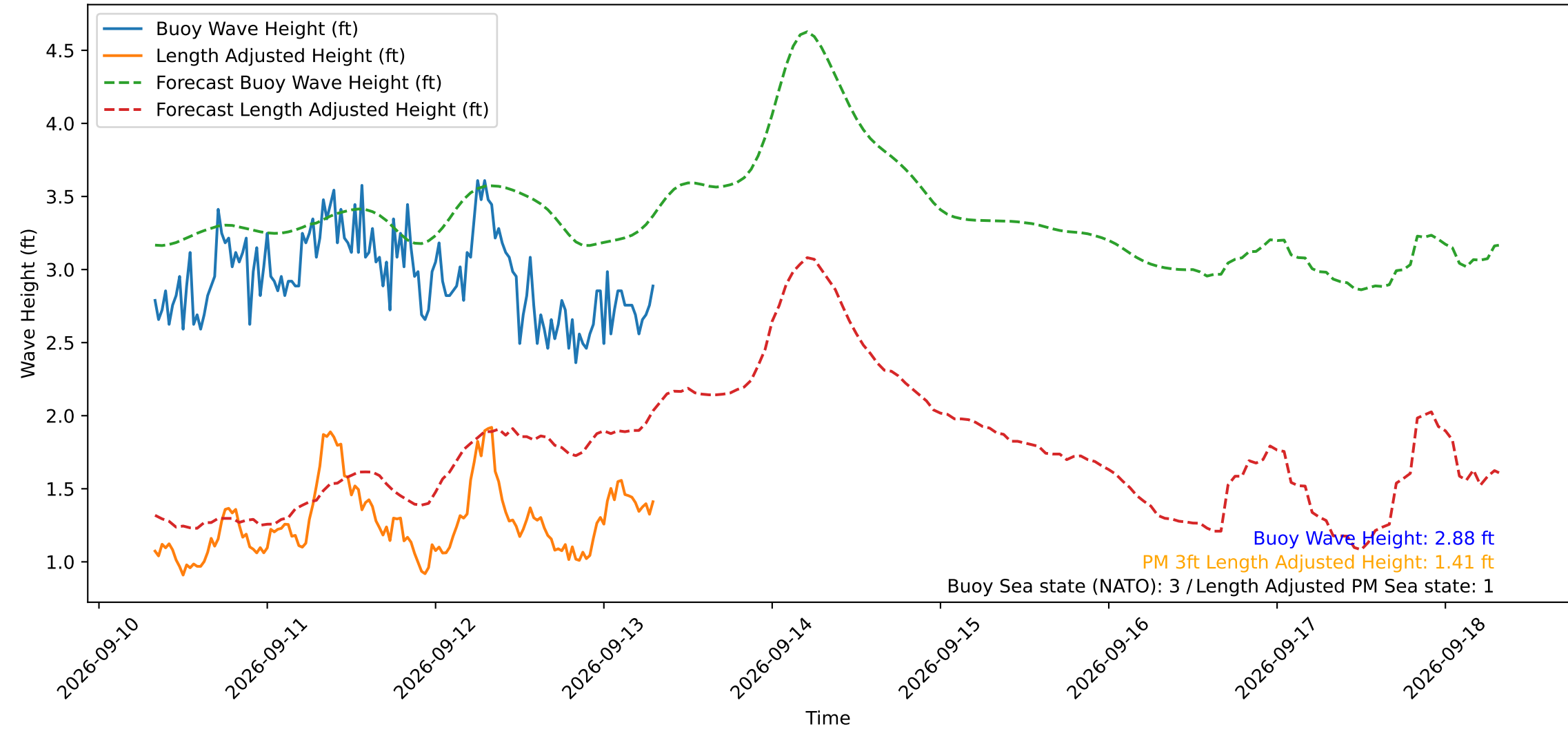
Wave Heights over Time for Green Beach at 2026-09-13 07:41:11
