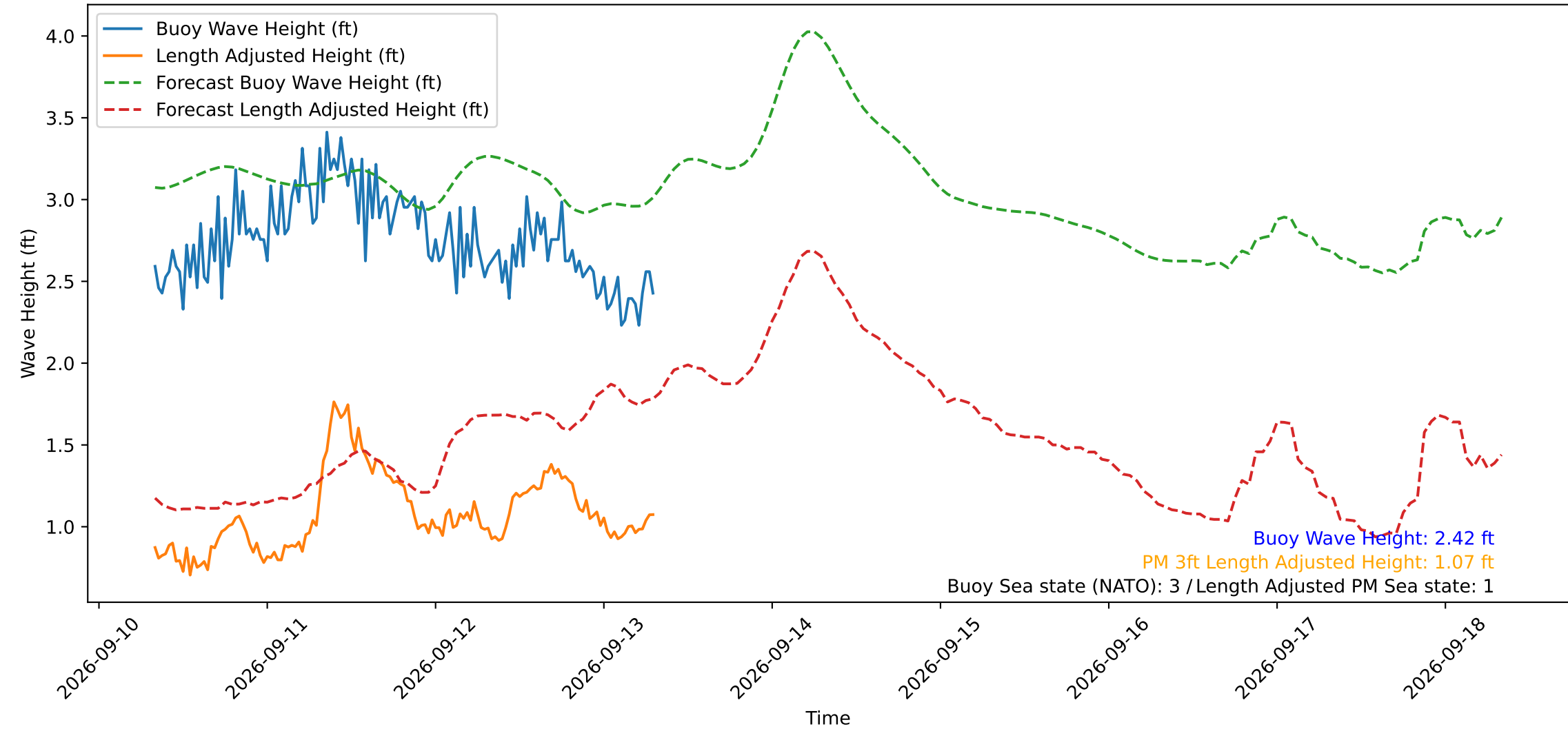
Wave Heights over Time for Red Beach at 2026-09-13 07:40:49
