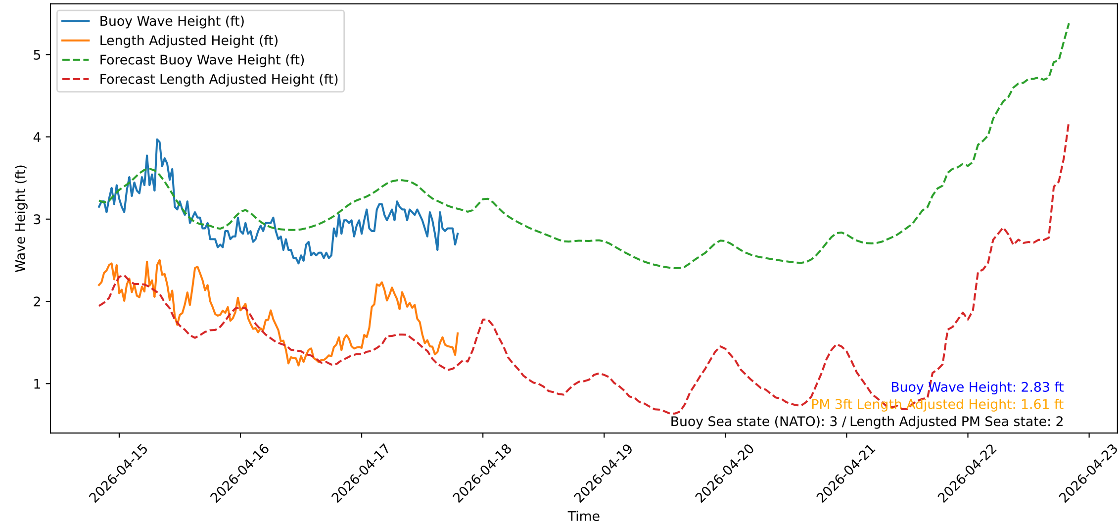
Wave Heights over Time for Green Beach at 2026-04-17 20:01:12
