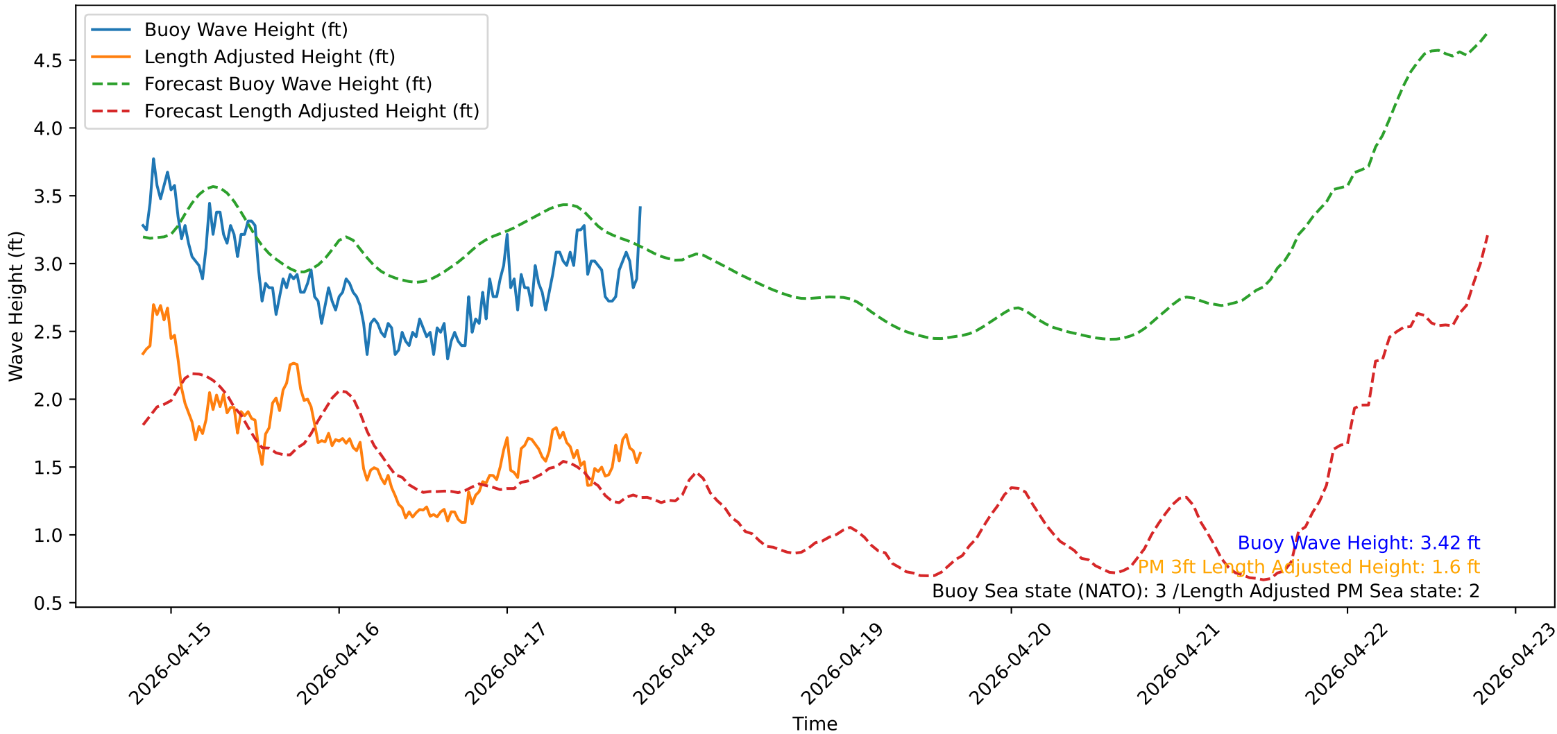
Wave Heights over Time for Oceanside Harbor at 2026-04-17 20:00:31
