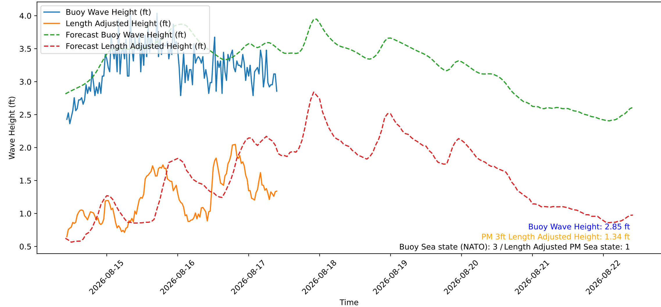
Wave Heights over Time for Red Beach at 2026-08-17 10:10:46
