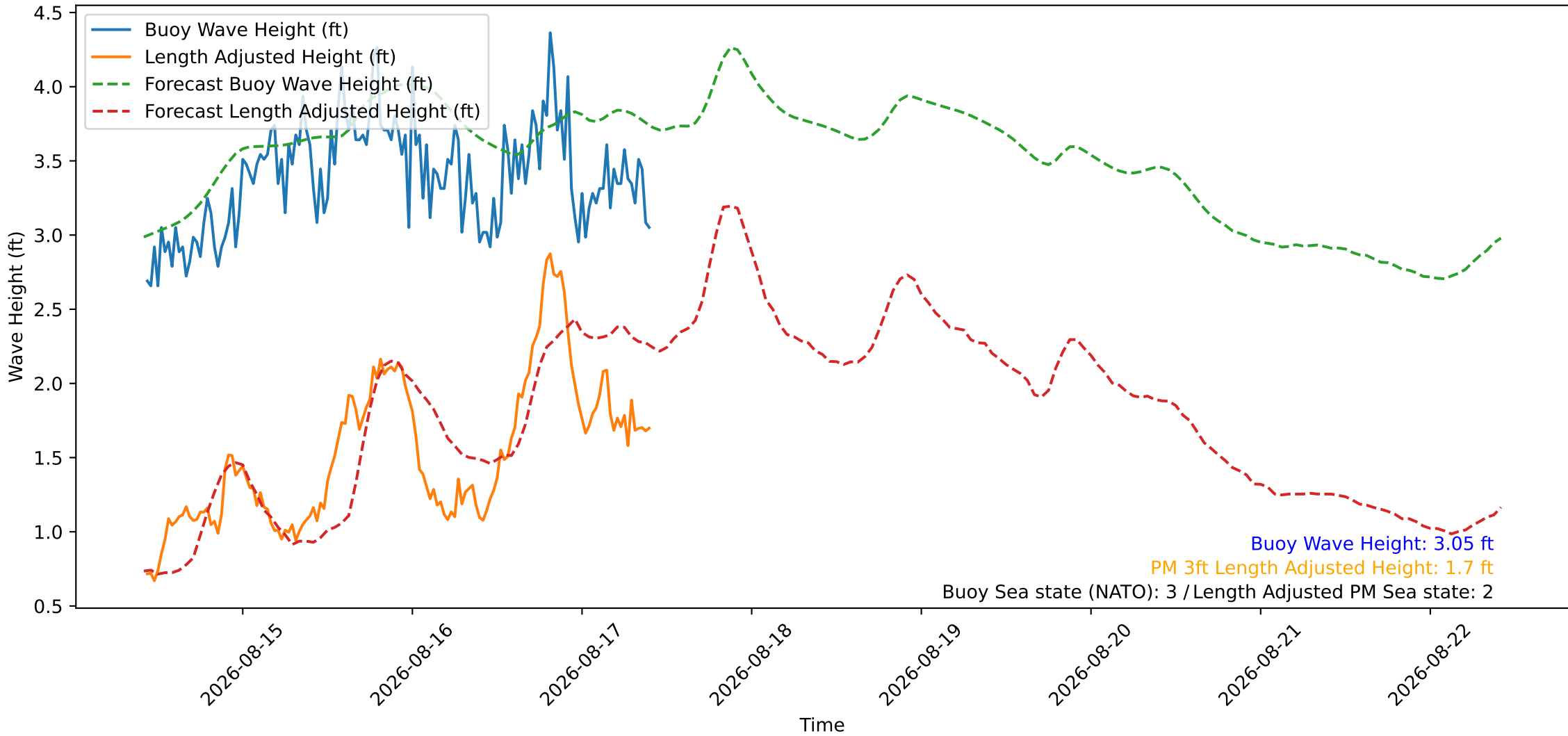
Wave Heights over Time for Green Beach at 2026-08-17 10:11:09
