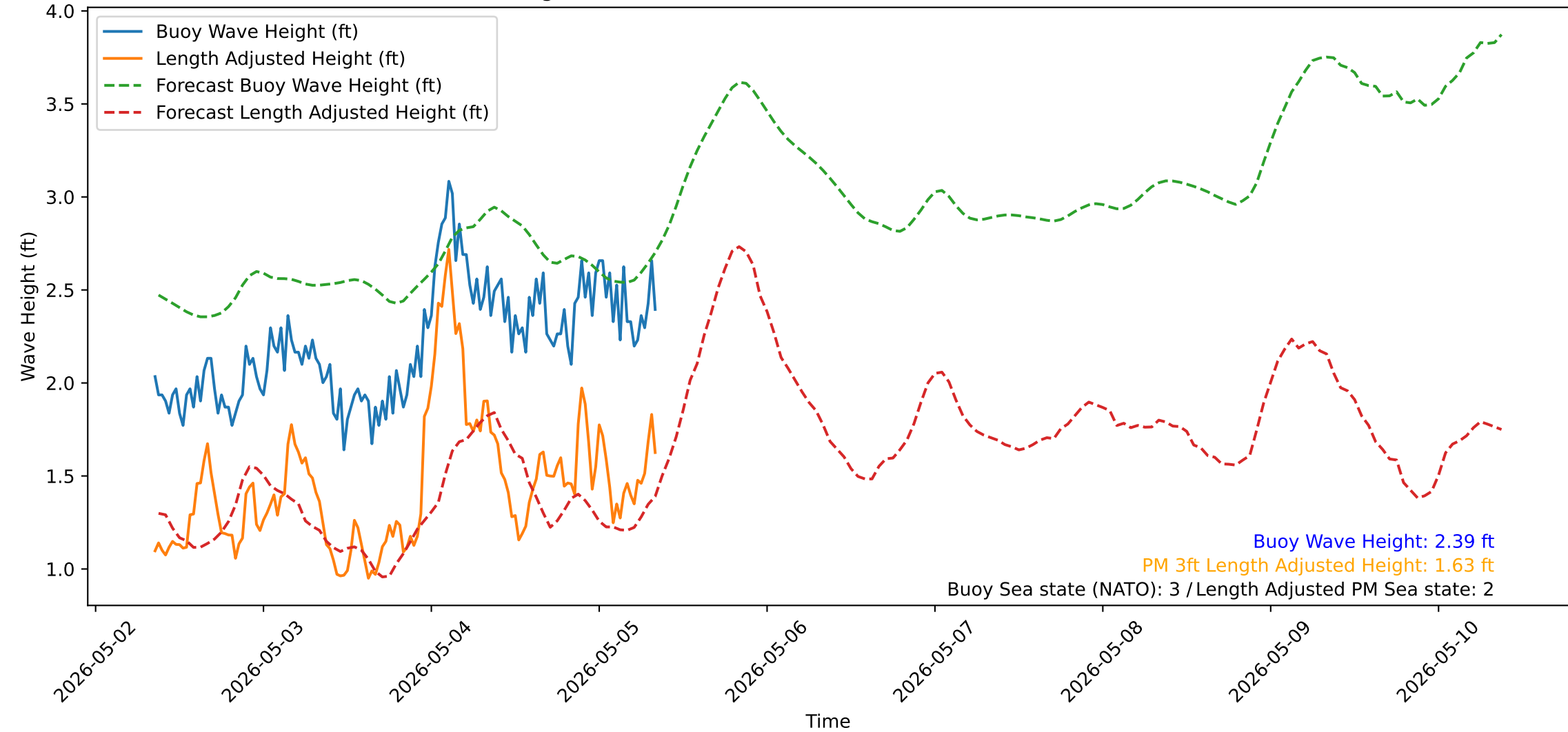
Wave Heights over Time for Oceanside Harbor at 2026-05-05 08:30:32
