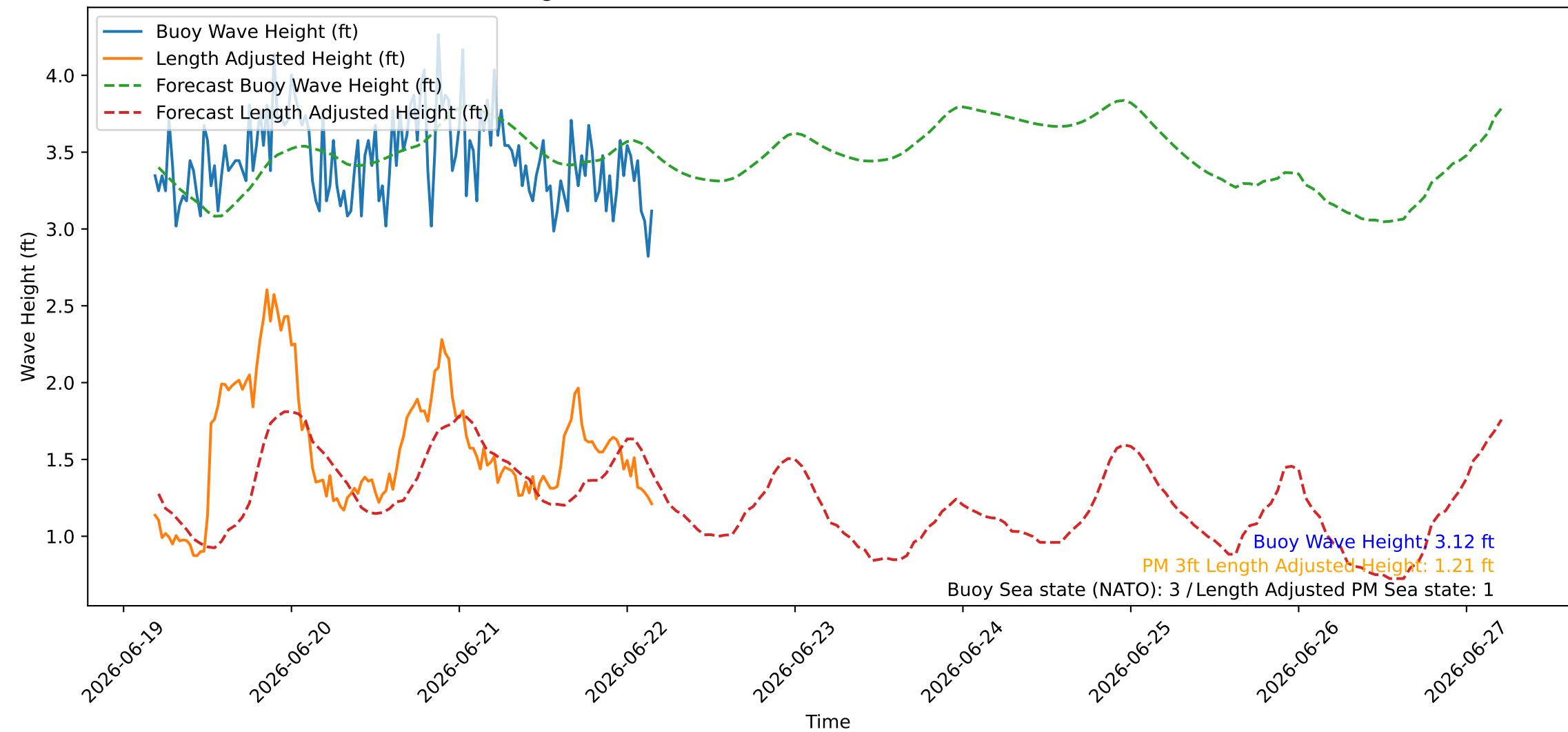
Wave Heights over Time for Oceanside Harbor at 2026-06-22 04:30:27
