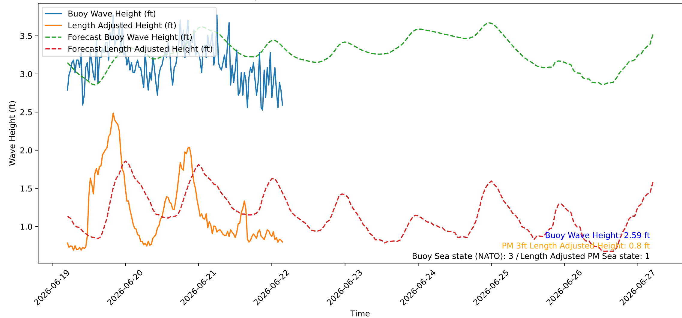
Wave Heights over Time for Red Beach at 2026-06-22 04:30:46
