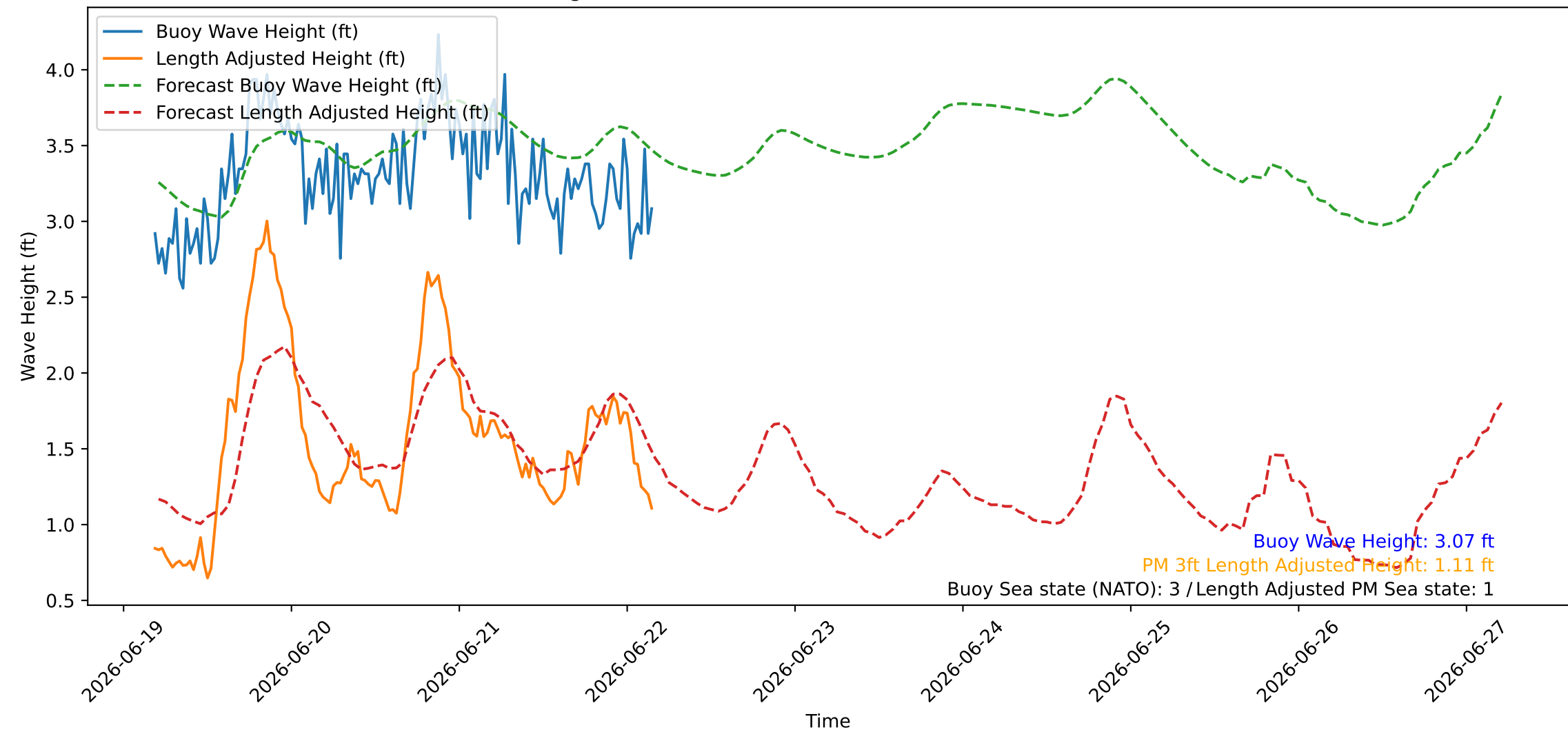
Wave Heights over Time for Green Beach at 2026-06-22 04:31:11
