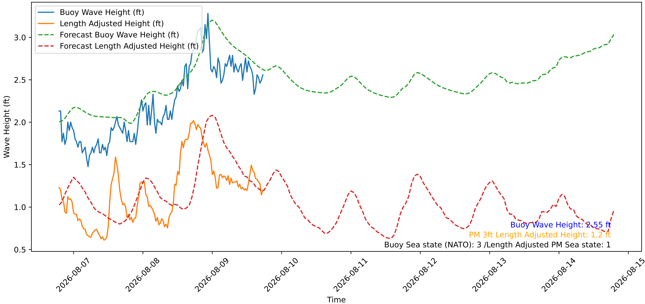
Wave Heights over Time for Red Beach at 2026-08-09 18:30:46
