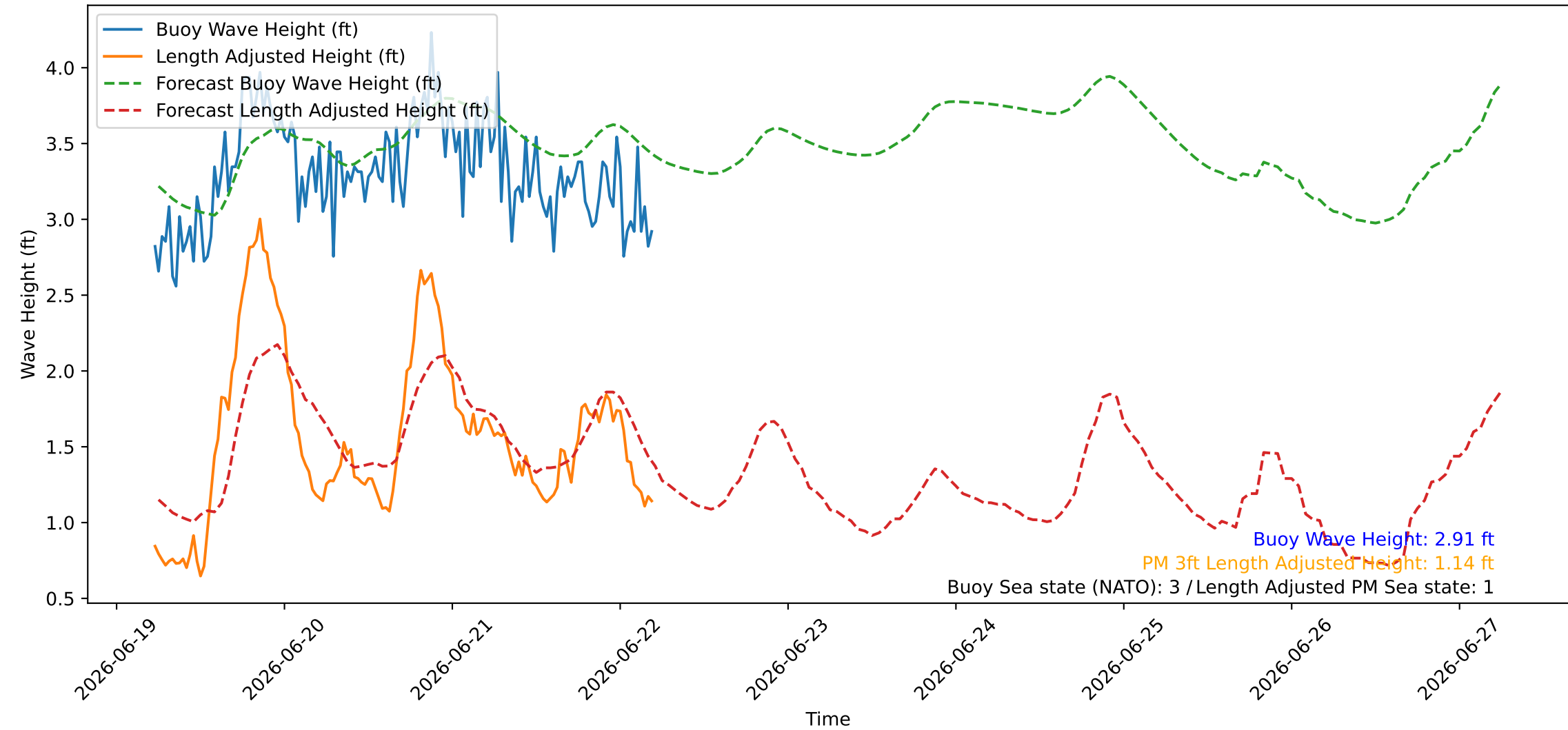
Wave Heights over Time for Green Beach at 2026-06-22 05:31:08
