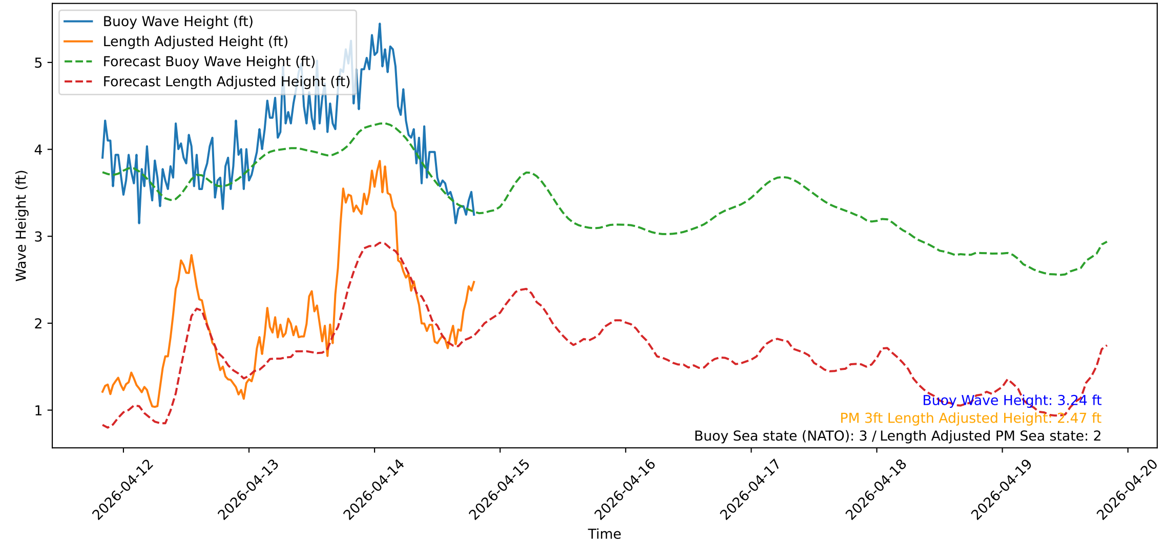
Wave Heights over Time for Oceanside Harbor at 2026-04-14 19:50:31
