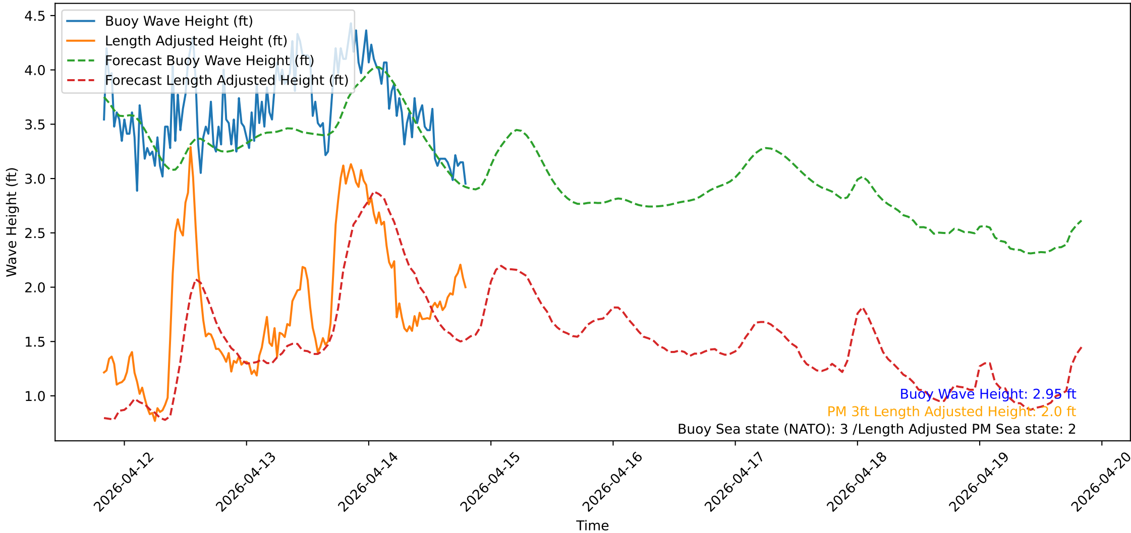
Wave Heights over Time for Red Beach at 2026-04-14 19:50:52
