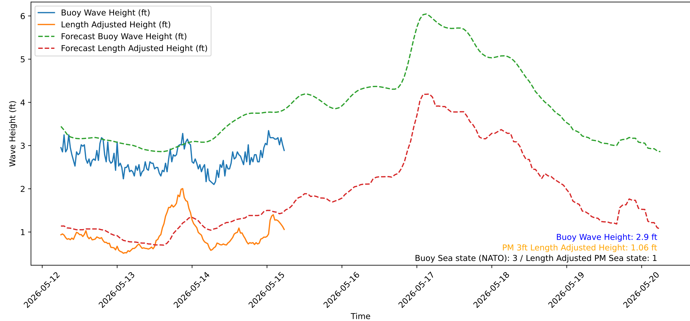
Wave Heights over Time for Green Beach at 2026-05-15 06:11:14
