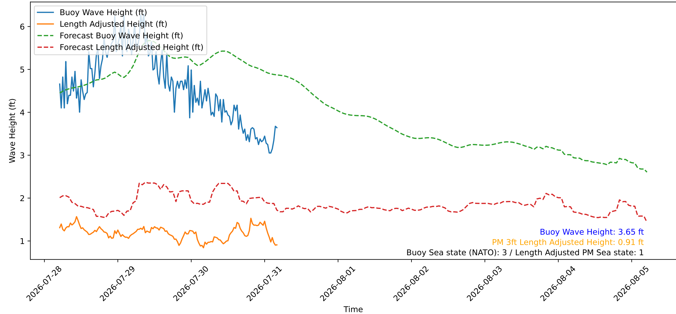
Wave Heights over Time for Green Beach at 2026-07-31 04:51:10
