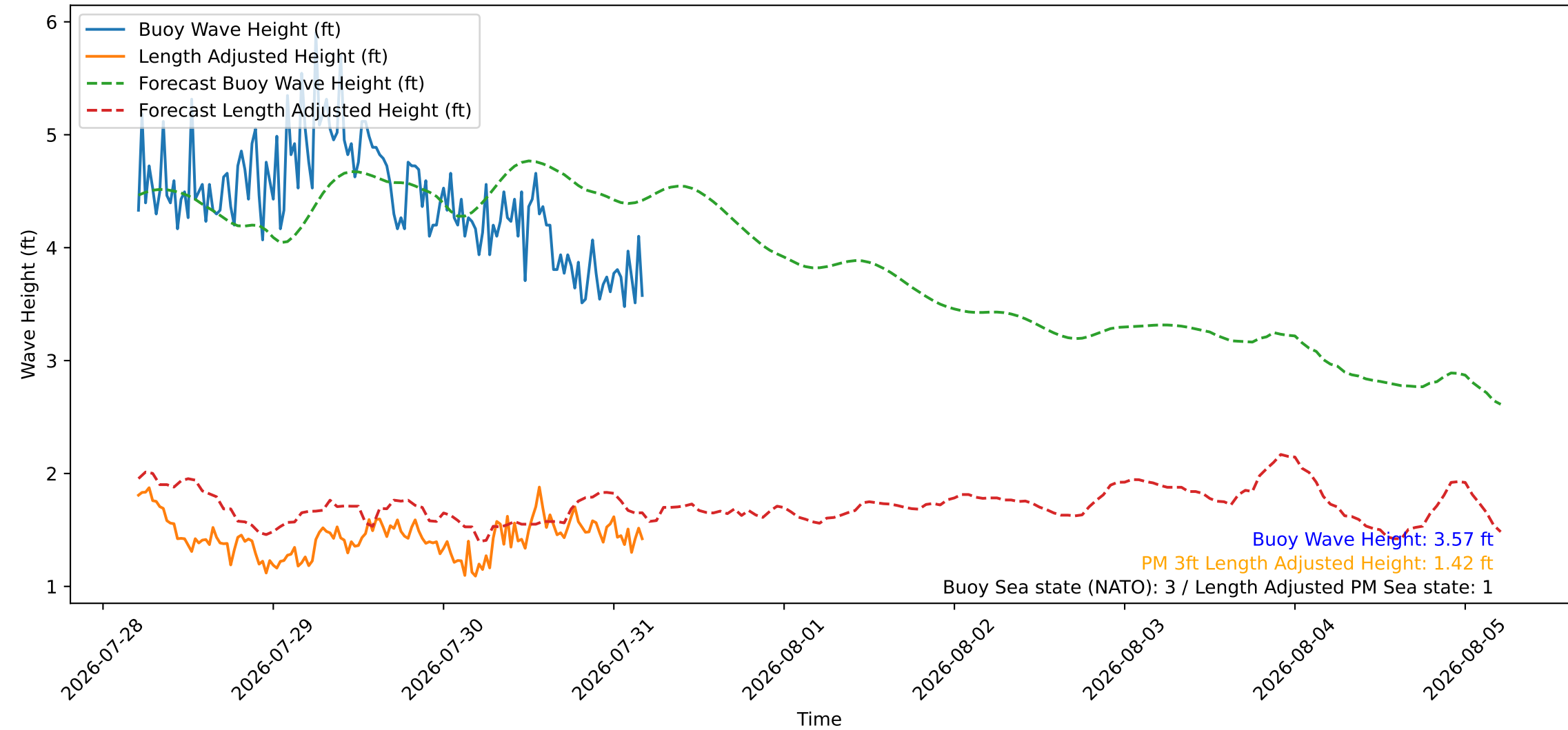
Wave Heights over Time for Oceanside Harbor at 2026-07-31 04:50:26
