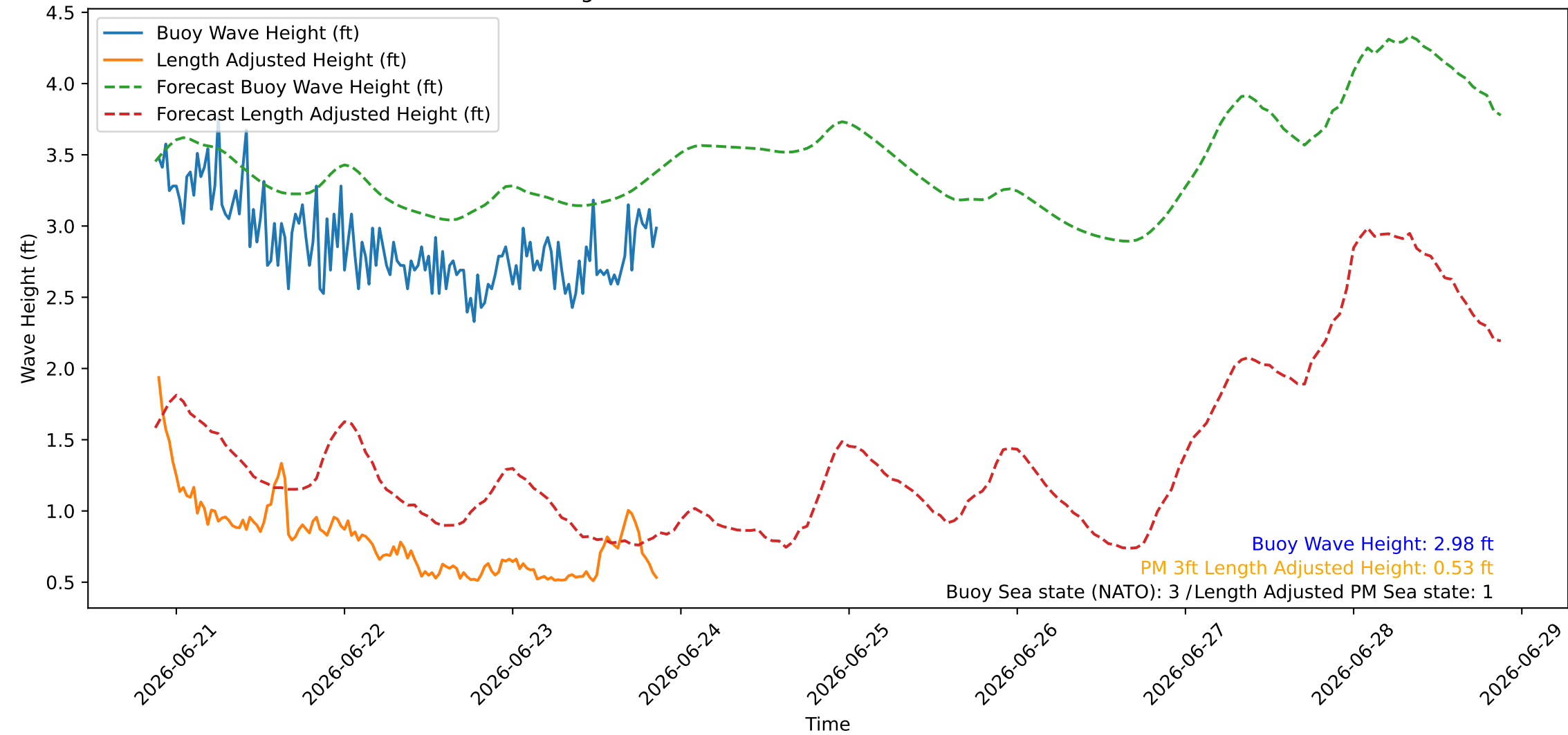
Wave Heights over Time for Red Beach at 2026-06-23 21:10:45
