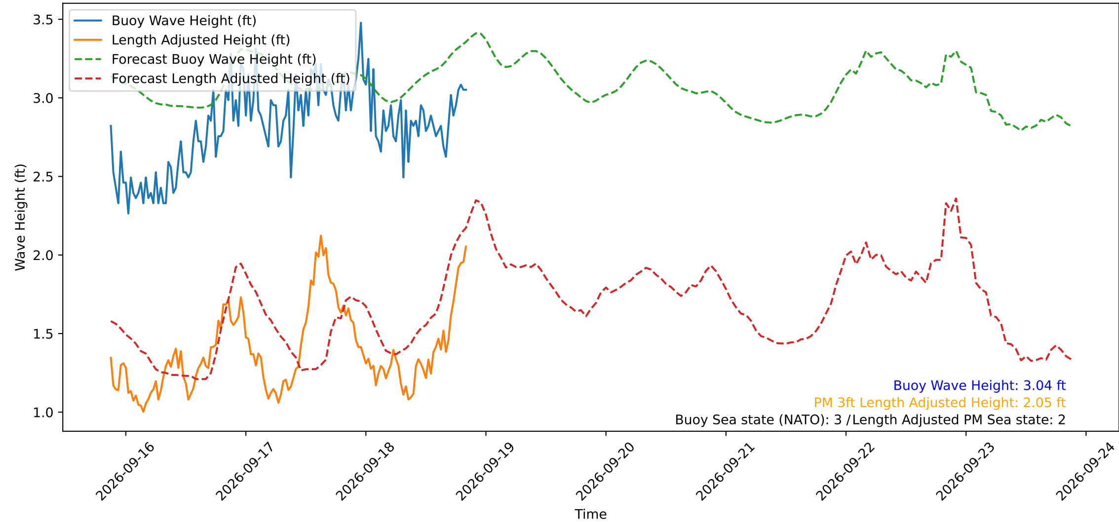
Wave Heights over Time for Green Beach at 2026-09-18 20:51:13
