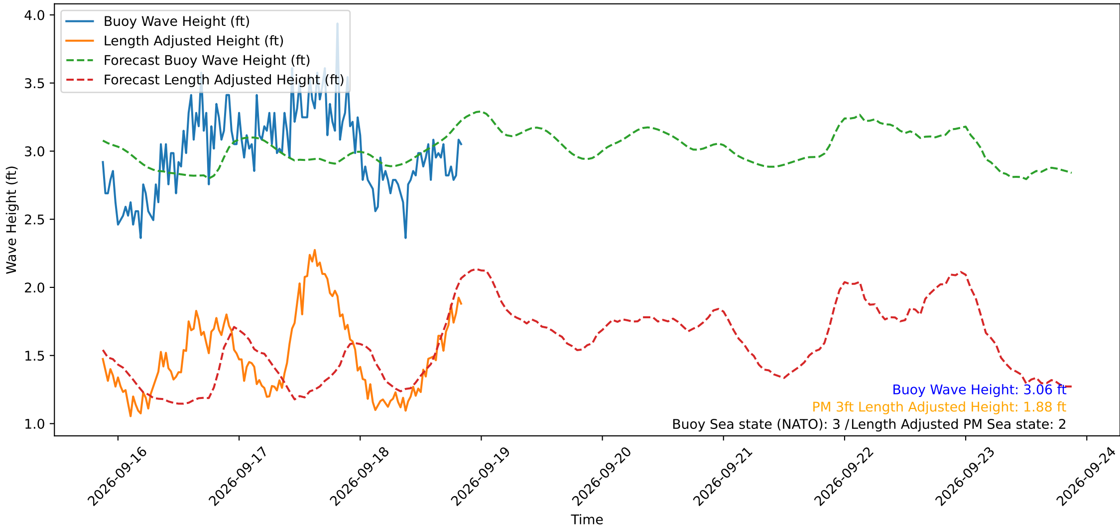
Wave Heights over Time for Oceanside Harbor at 2026-09-18 20:50:30
