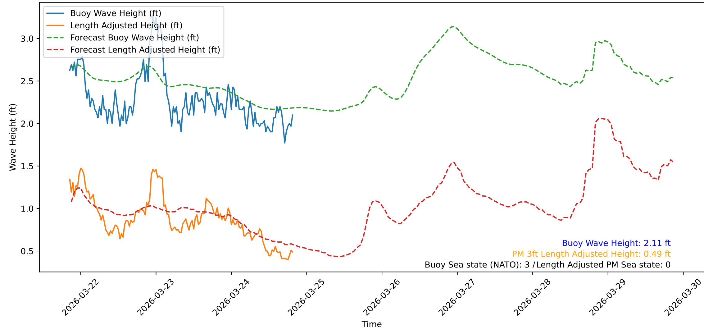
Wave Heights over Time for Green Beach at 2026-03-24 20:31:09
