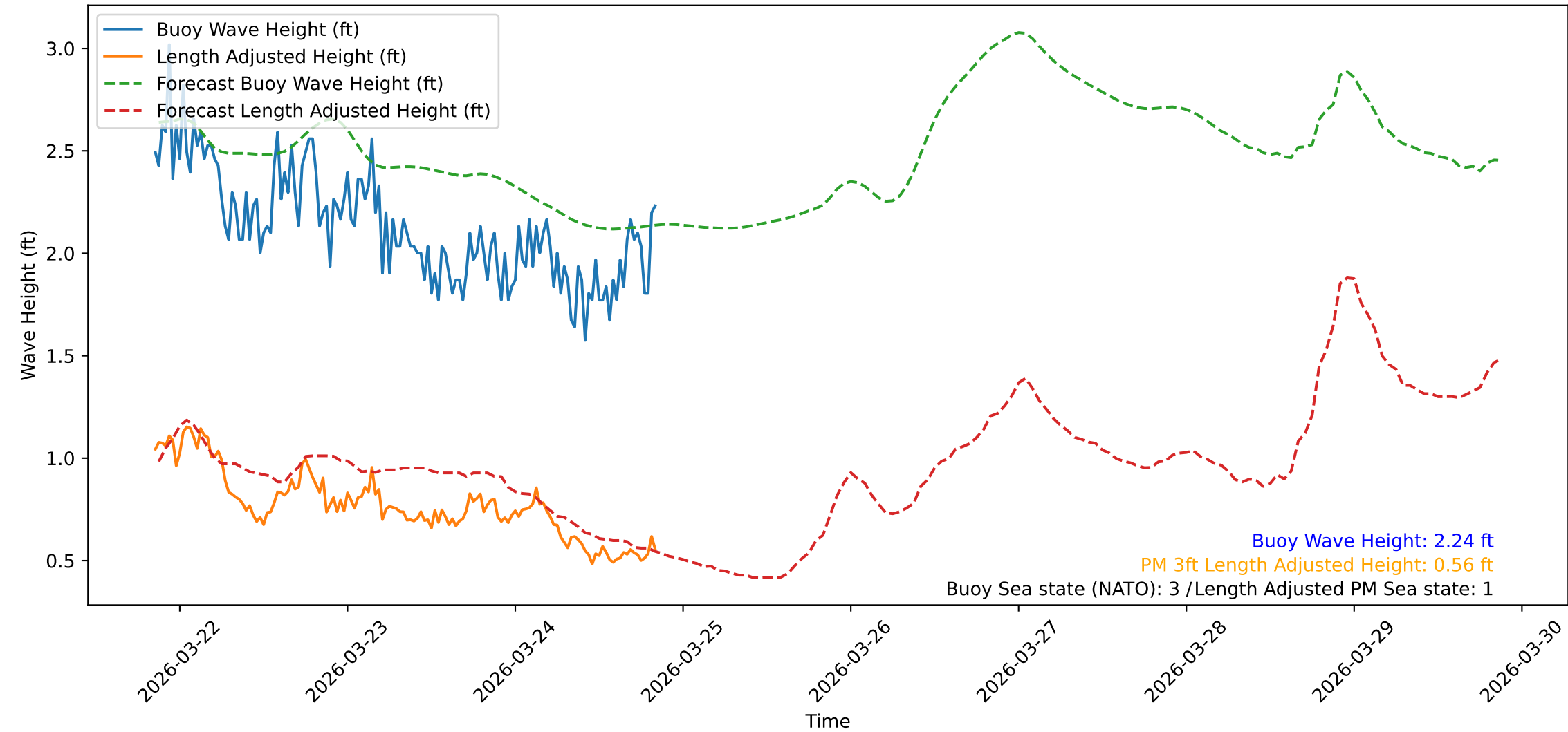
Wave Heights over Time for Oceanside Harbor at 2026-03-24 20:30:31
