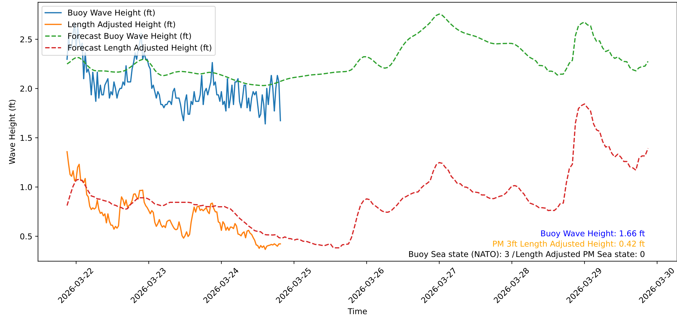
Wave Heights over Time for Red Beach at 2026-03-24 20:30:47
