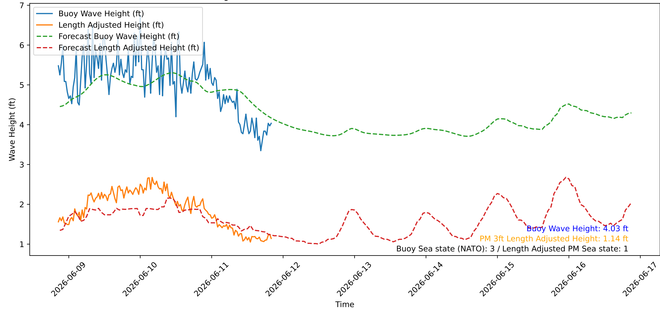
Wave Heights over Time for Oceanside Harbor at 2026-06-11 20:30:26
