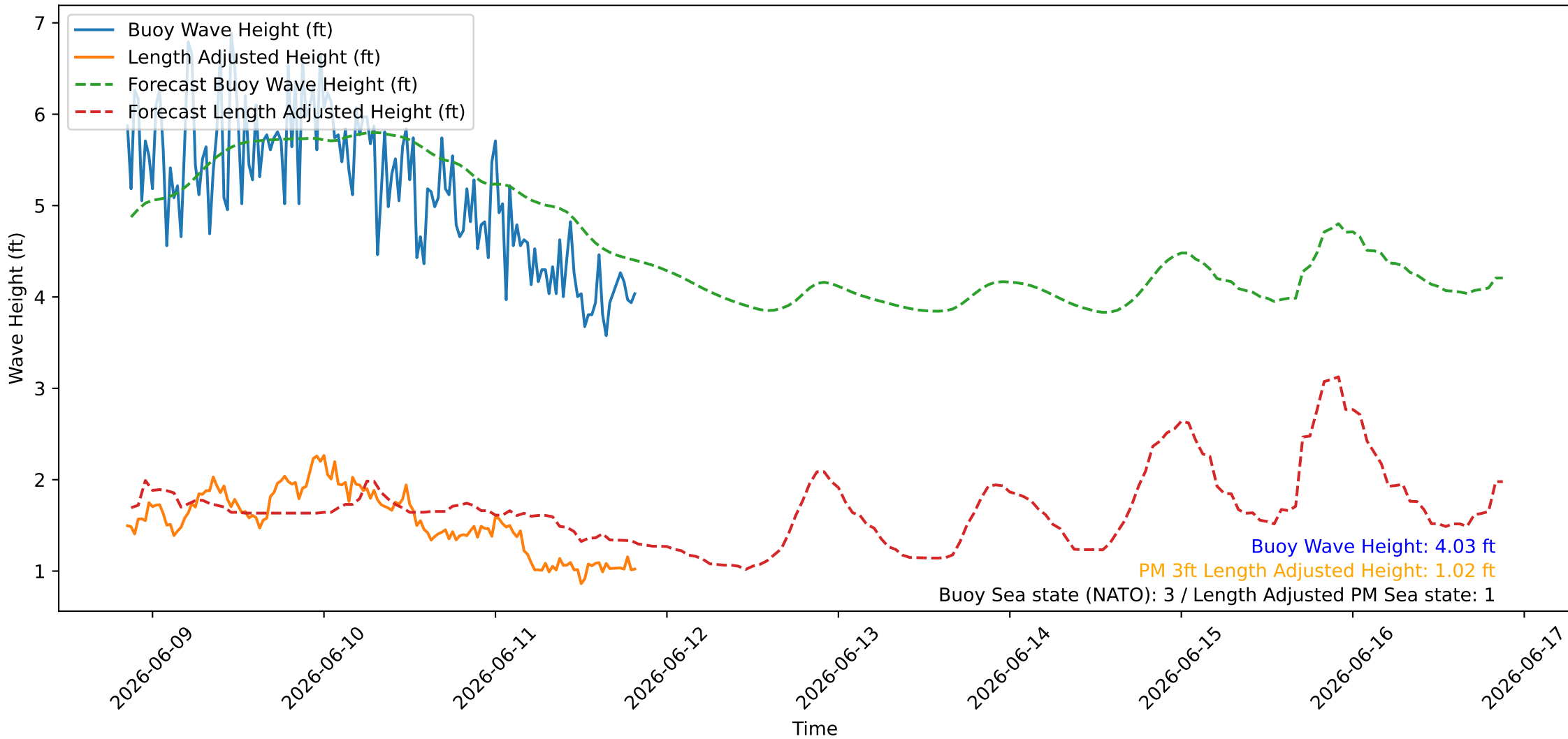
Wave Heights over Time for Green Beach at 2026-06-11 20:31:09
