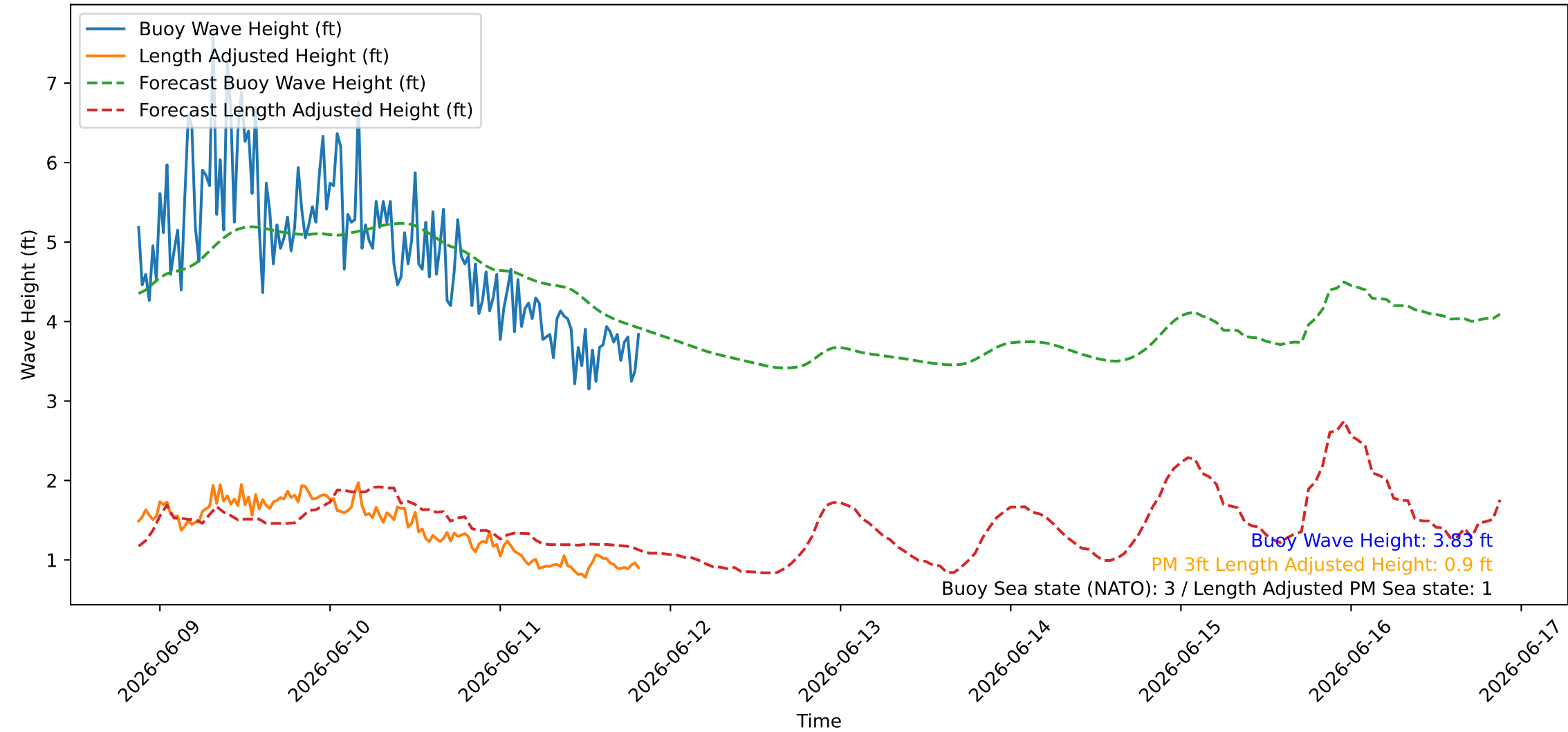
Wave Heights over Time for Red Beach at 2026-06-11 20:30:46
