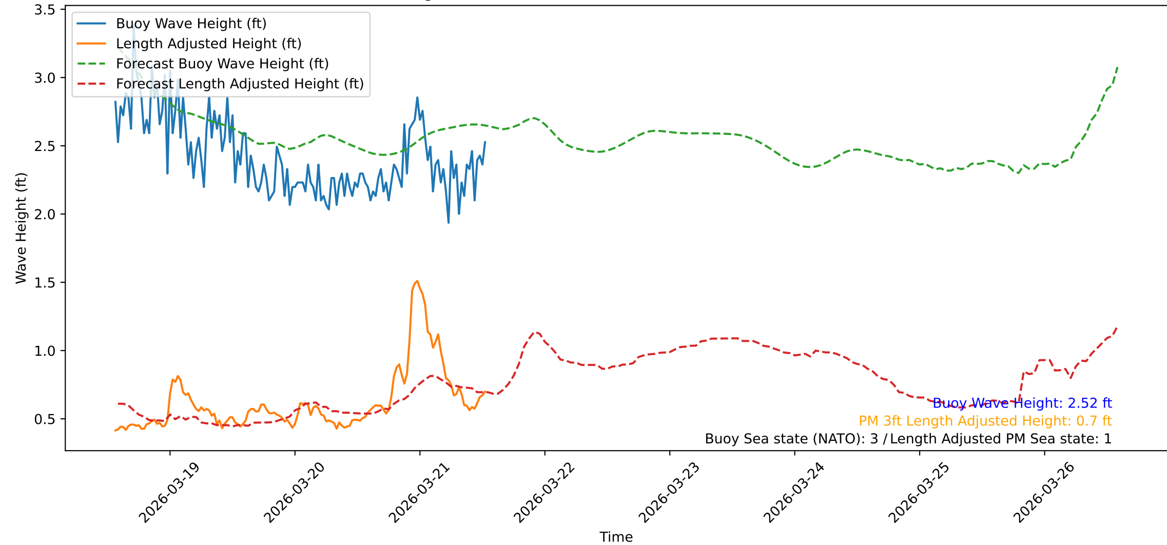
Wave Heights over Time for Green Beach at 2026-03-21 13:31:11
