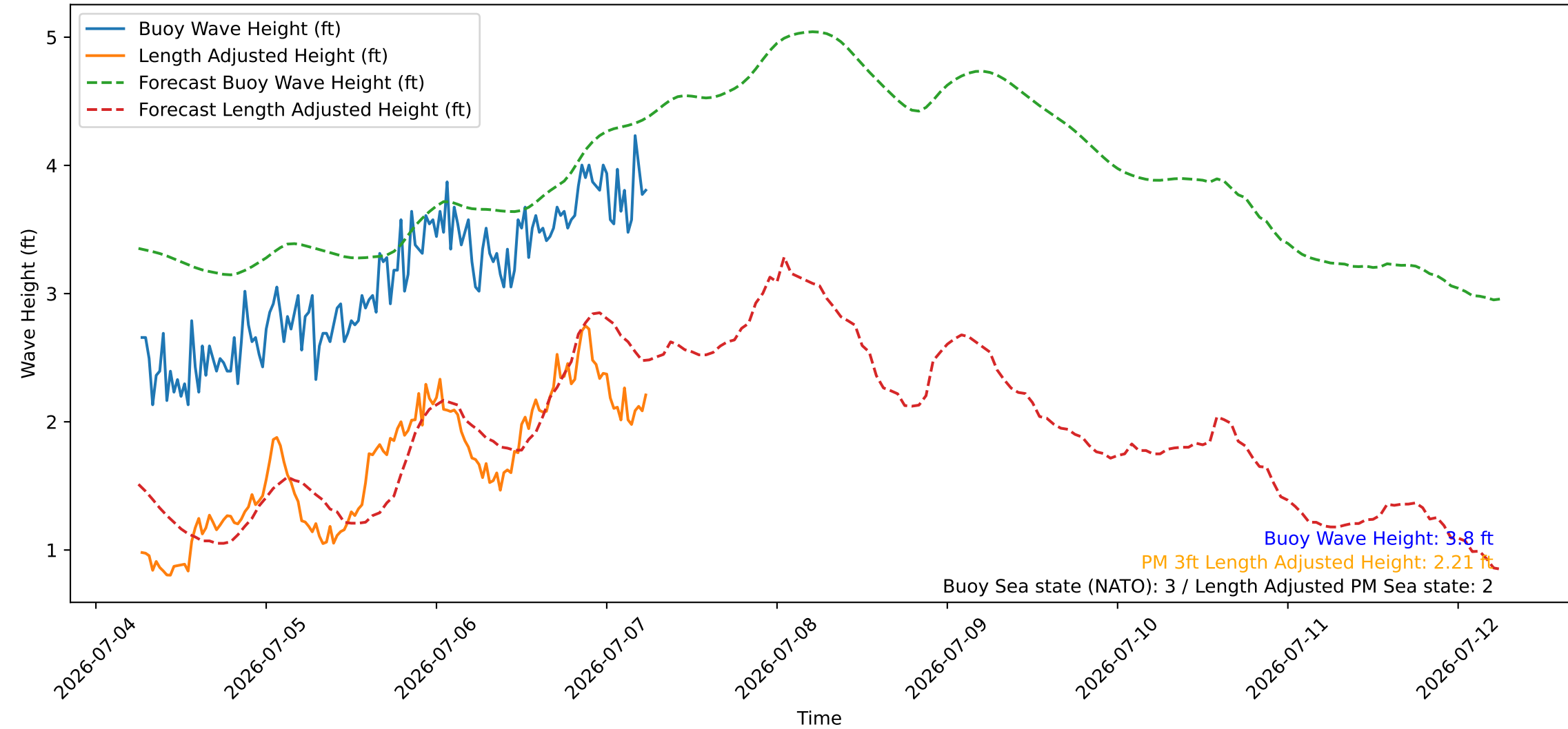
Wave Heights over Time for Oceanside Harbor at 2026-07-07 06:20:26
