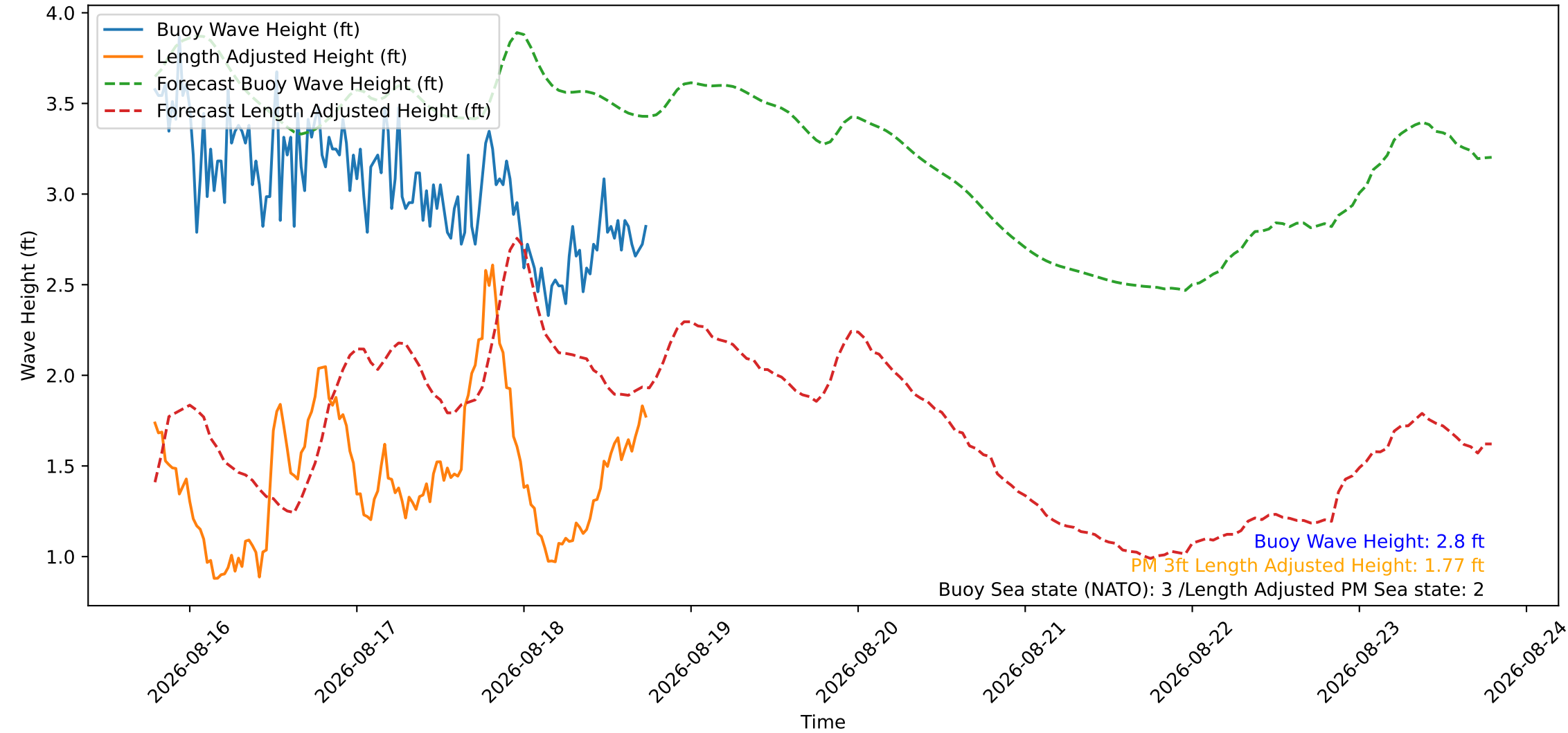
Wave Heights over Time for Red Beach at 2026-08-18 18:40:46
