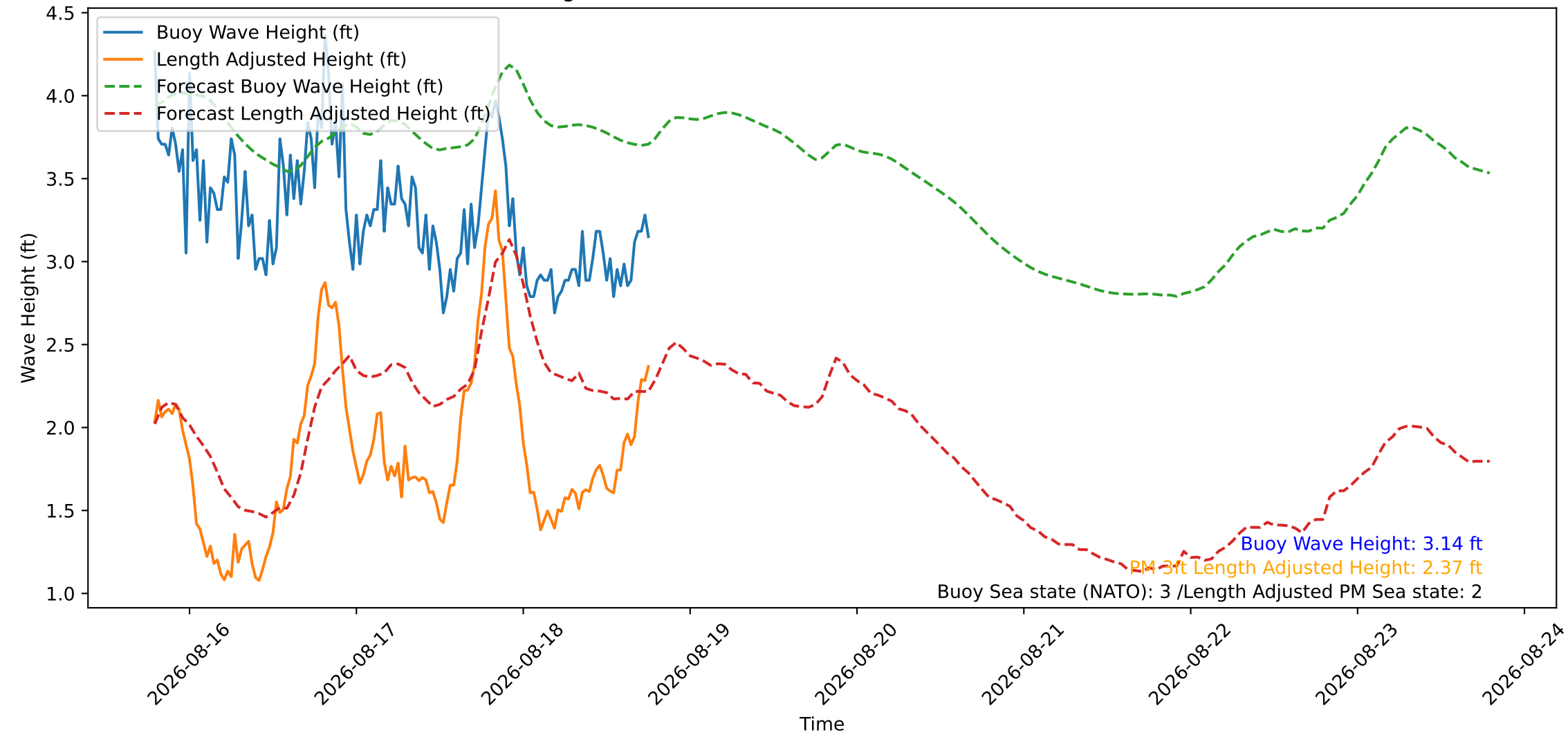
Wave Heights over Time for Green Beach at 2026-08-18 18:41:09
