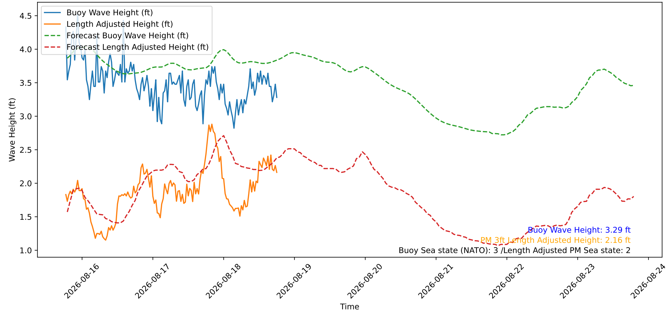
Wave Heights over Time for Oceanside Harbor at 2026-08-18 18:40:27
