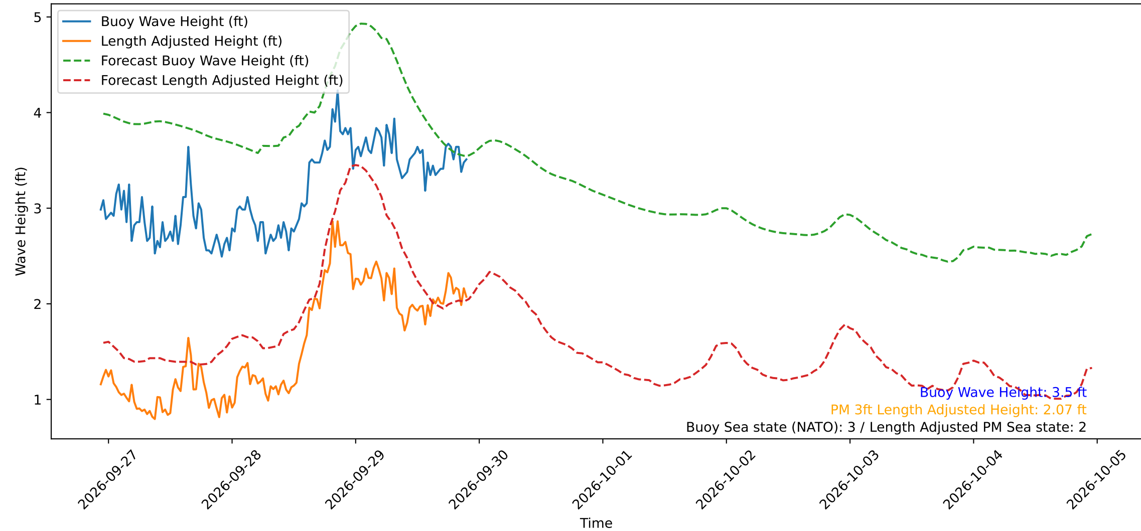
Wave Heights over Time for Oceanside Harbor at 2026-09-29 22:30:29
