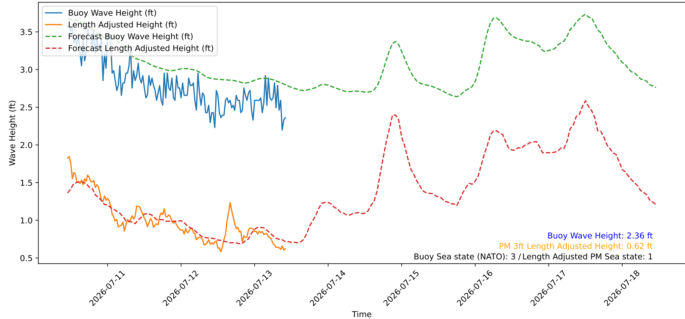
Wave Heights over Time for Green Beach at 2026-07-13 10:51:09
