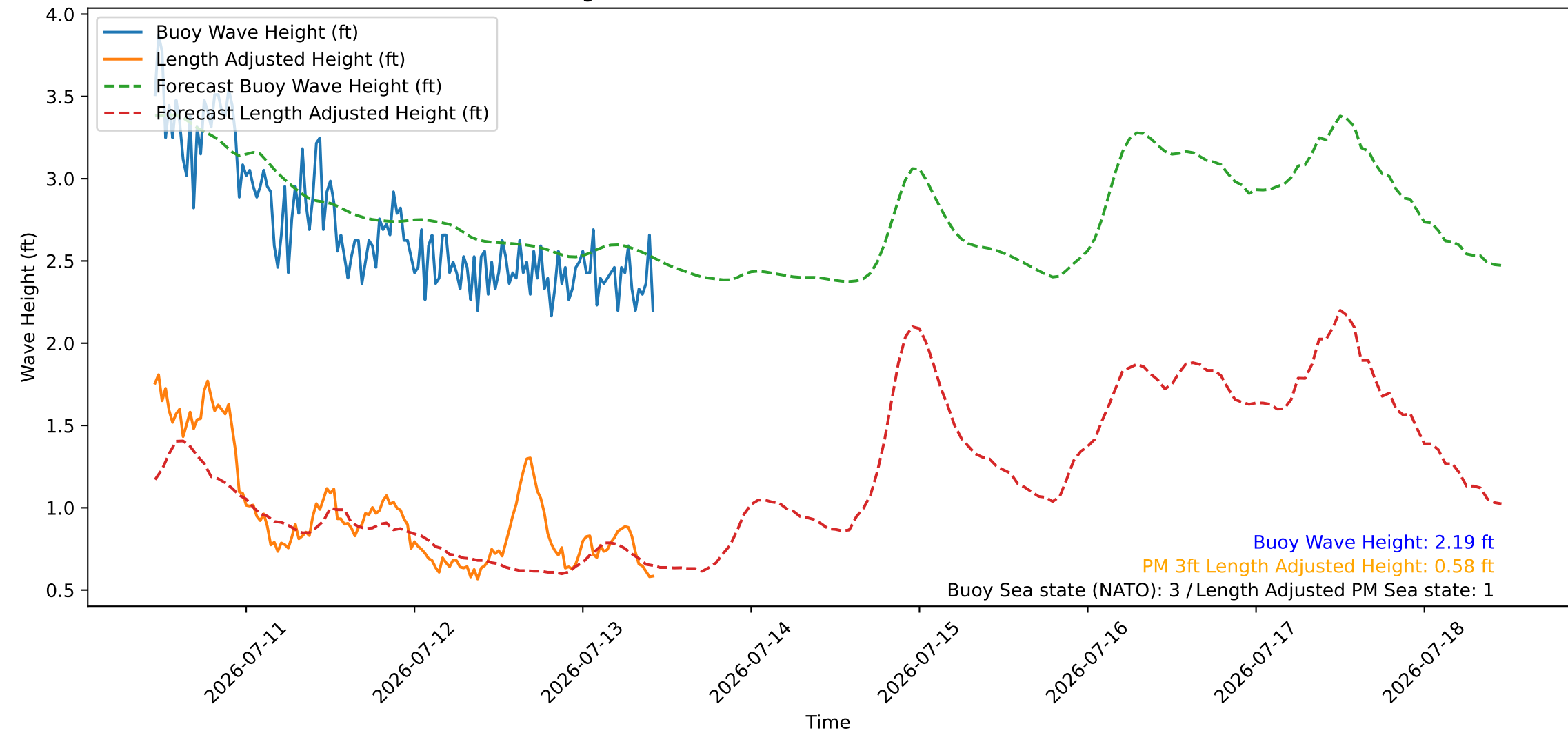
Wave Heights over Time for Red Beach at 2026-07-13 10:50:47
