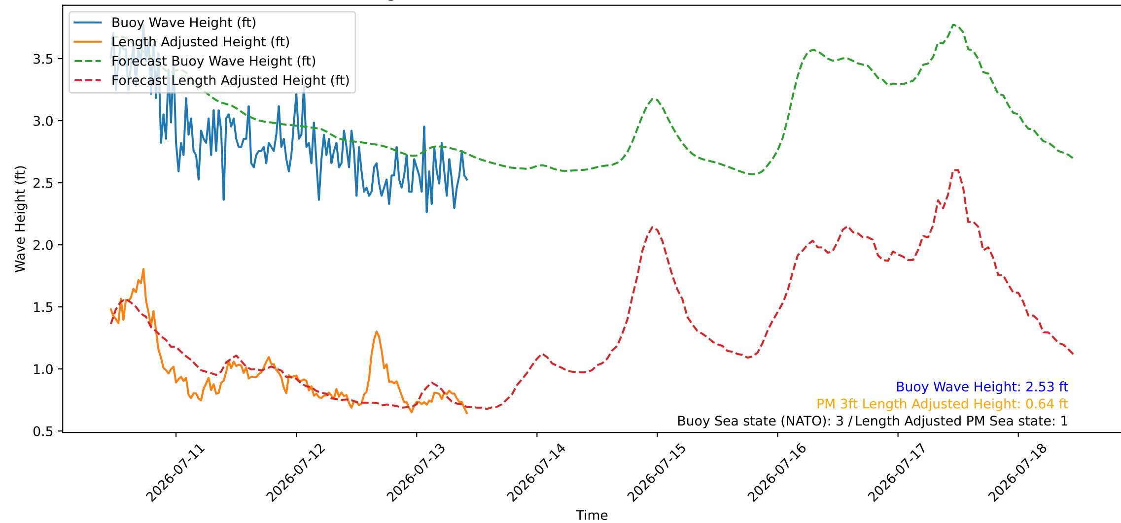
Wave Heights over Time for Oceanside Harbor at 2026-07-13 10:50:26
