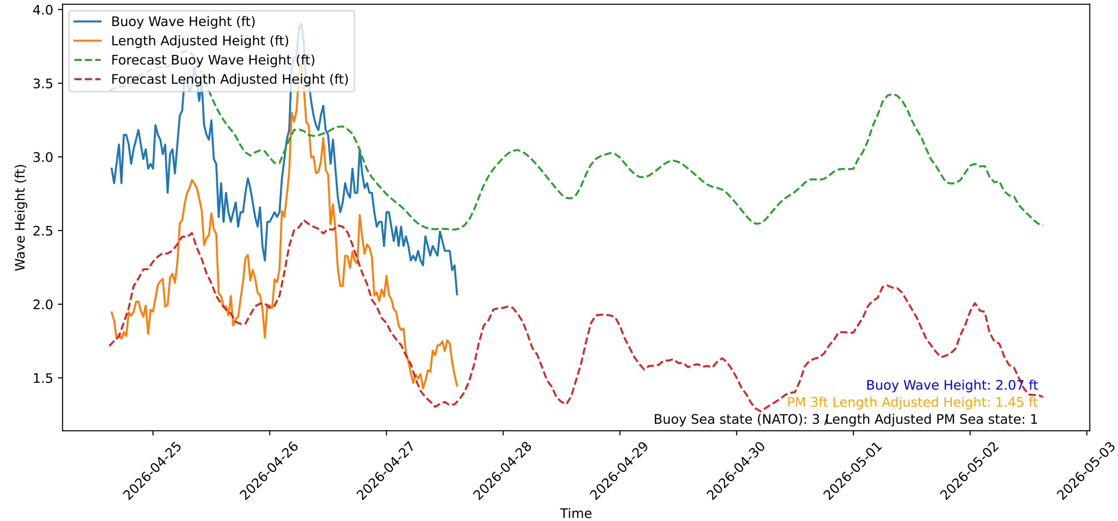
Wave Heights over Time for Oceanside Harbor at 2026-04-27 15:20:30
