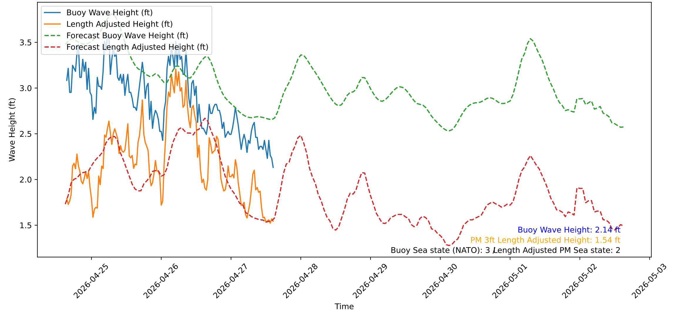
Wave Heights over Time for Green Beach at 2026-04-27 15:21:12
