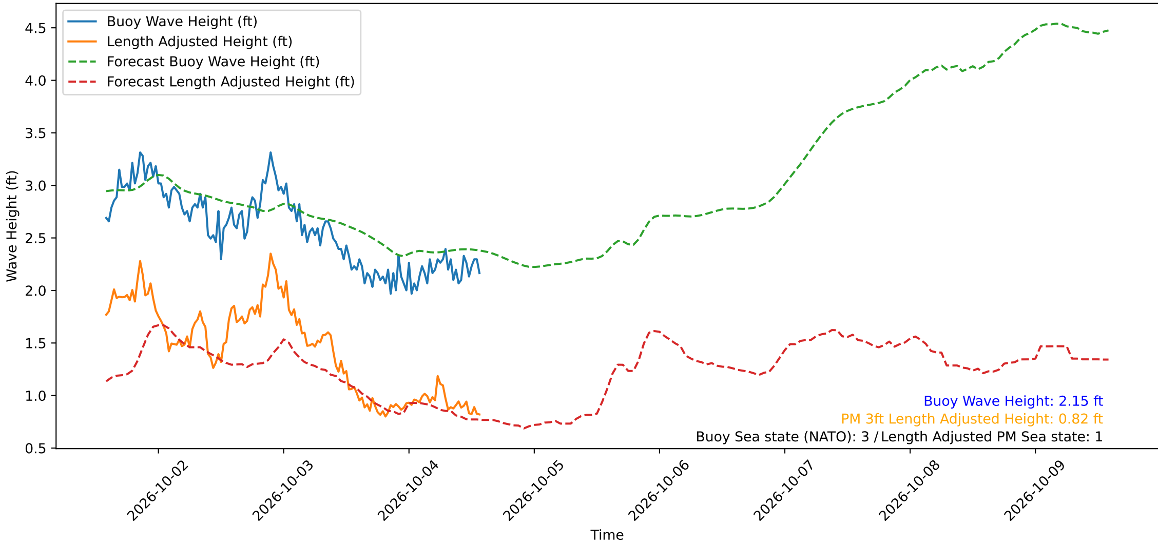
Wave Heights over Time for Oceanside Harbor at 2026-10-04 14:10:30
