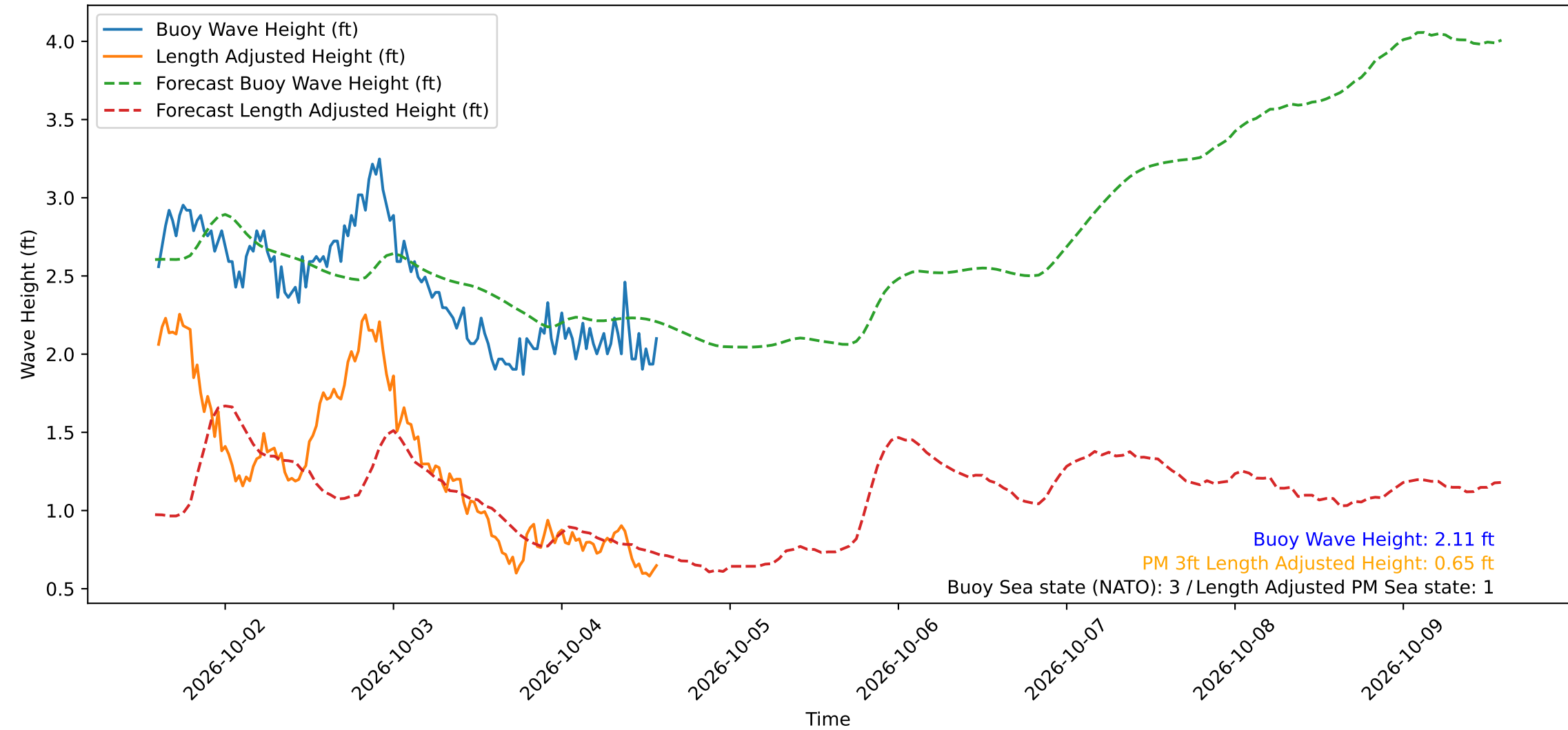
Wave Heights over Time for Red Beach at 2026-10-04 14:10:49
