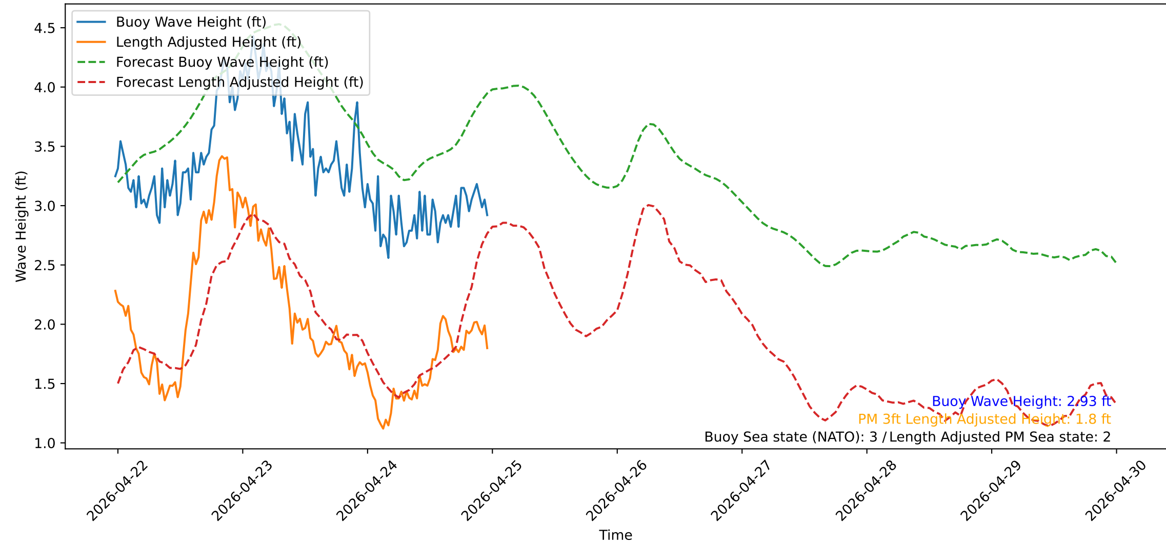
Wave Heights over Time for Oceanside Harbor at 2026-04-24 23:40:31
