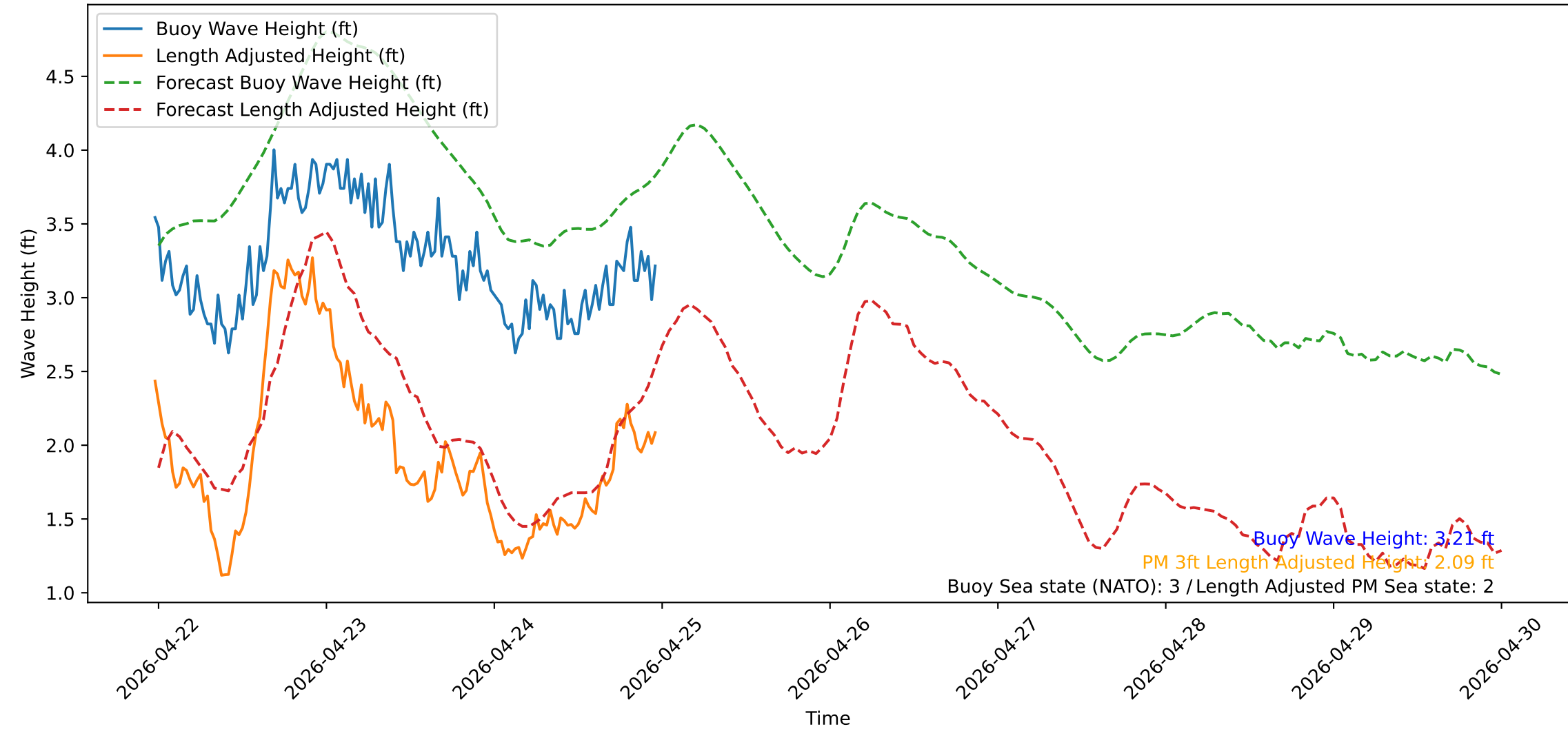
Wave Heights over Time for Green Beach at 2026-04-24 23:41:13
