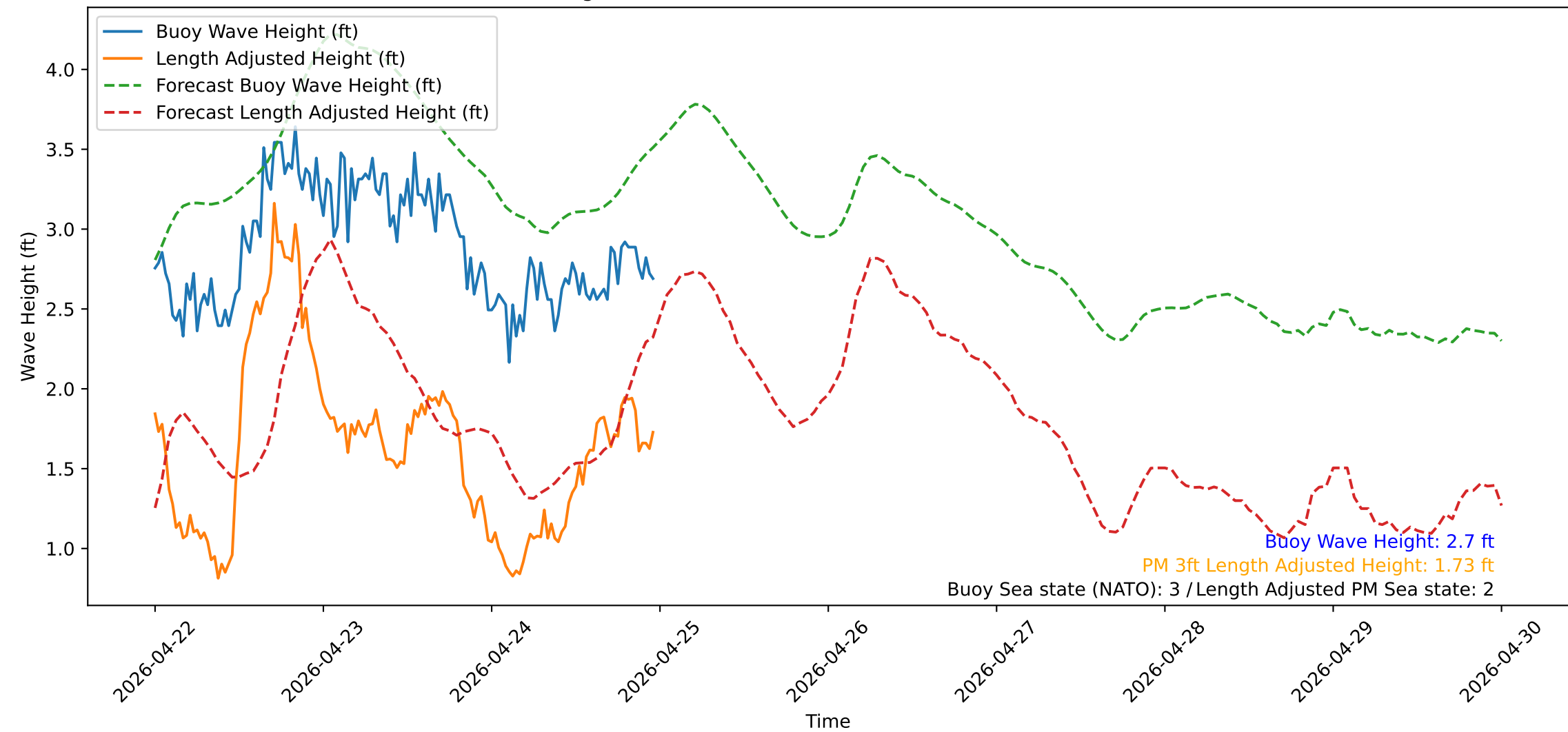
Wave Heights over Time for Red Beach at 2026-04-24 23:40:50
