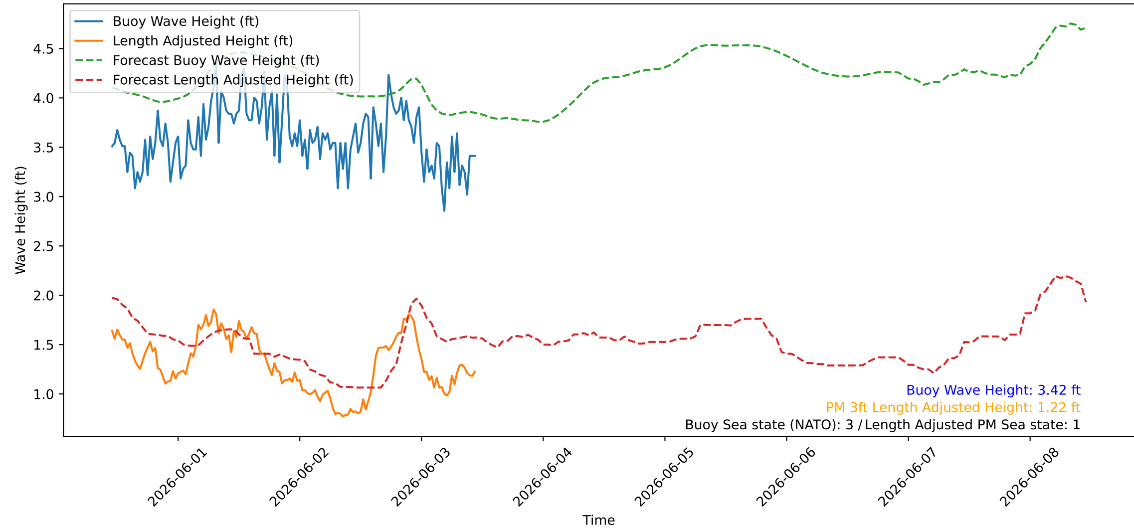
Wave Heights over Time for Green Beach at 2026-06-03 11:11:07
