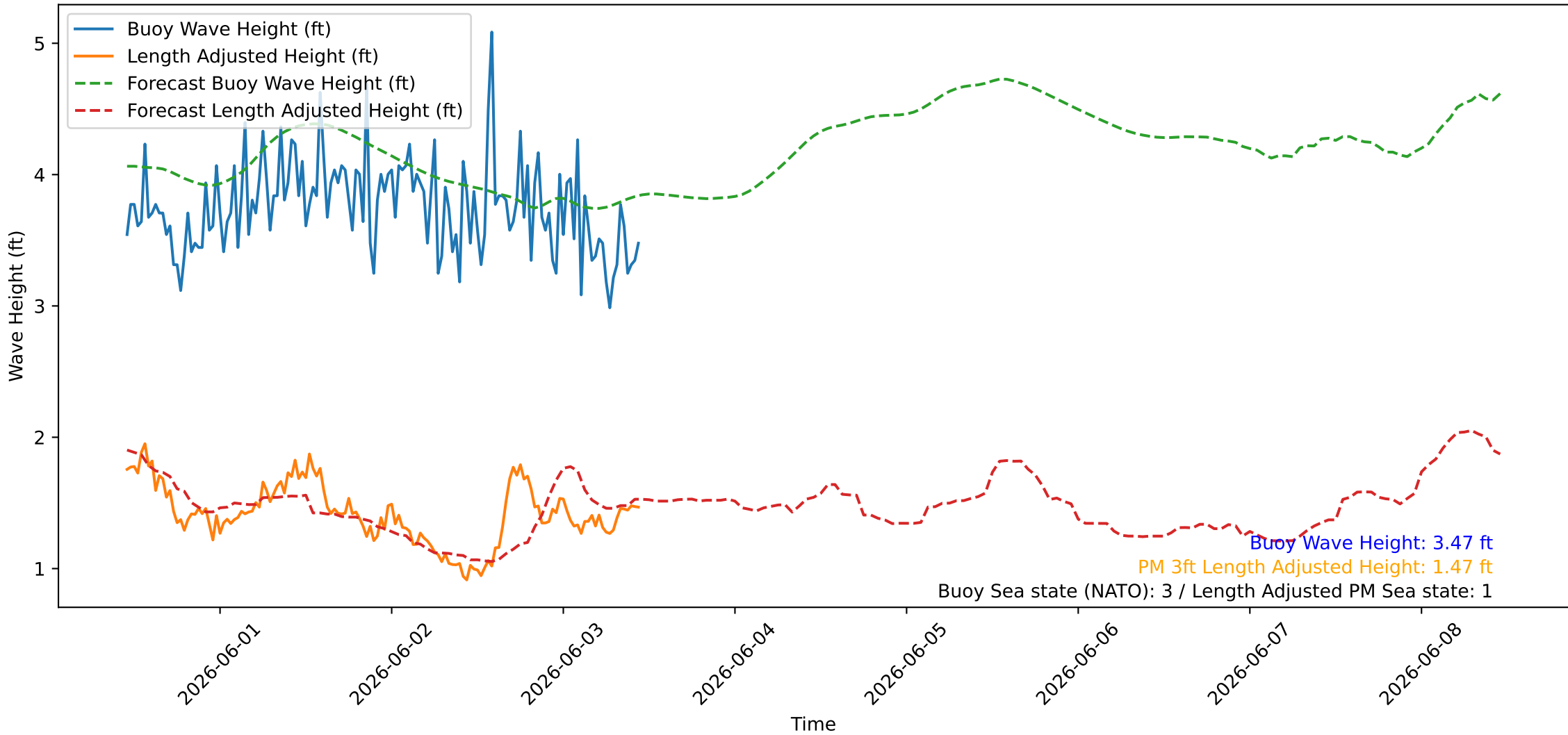
Wave Heights over Time for Oceanside Harbor at 2026-06-03 11:10:26
